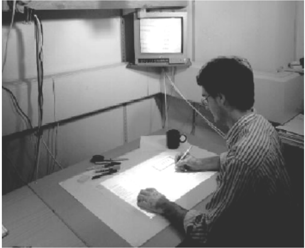
Figure 8: The Digital Desk (Wellner, 1993).
