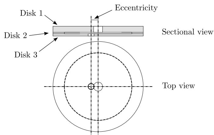
Figure 2.13: Triple-disk injector (Dumouchel et al. 2005 [22])
