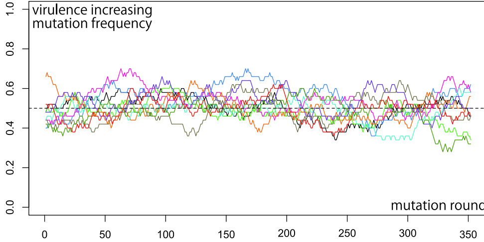
Figure δ.2.6. – Frequency of virulence increasing mutations.
