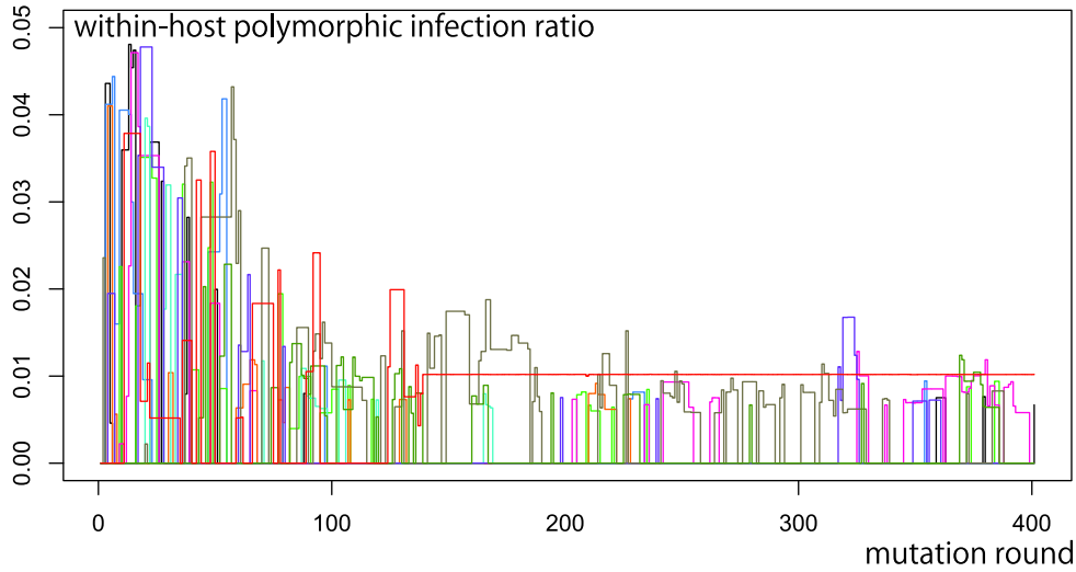
Figure δ.2.9. – Within-host polymorphic infection ratio.
