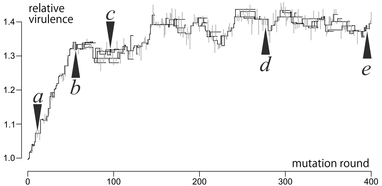
Figure δ.2.2. – Virulence phylogenetics: a commented example.
