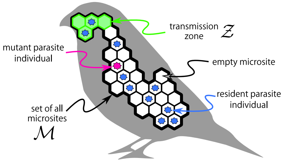
Figure δ.1.1. – Host microsite discretization.
