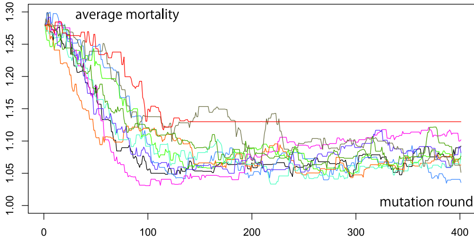
Figure δ.2.11. – Average host mortality.
