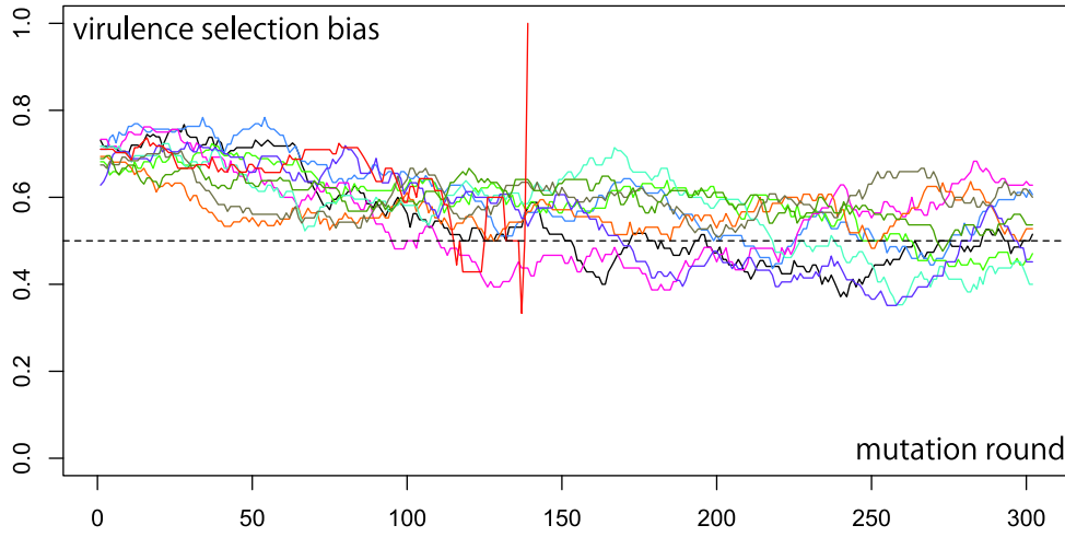
Figure δ.2.7. – Virulence selection bias.
