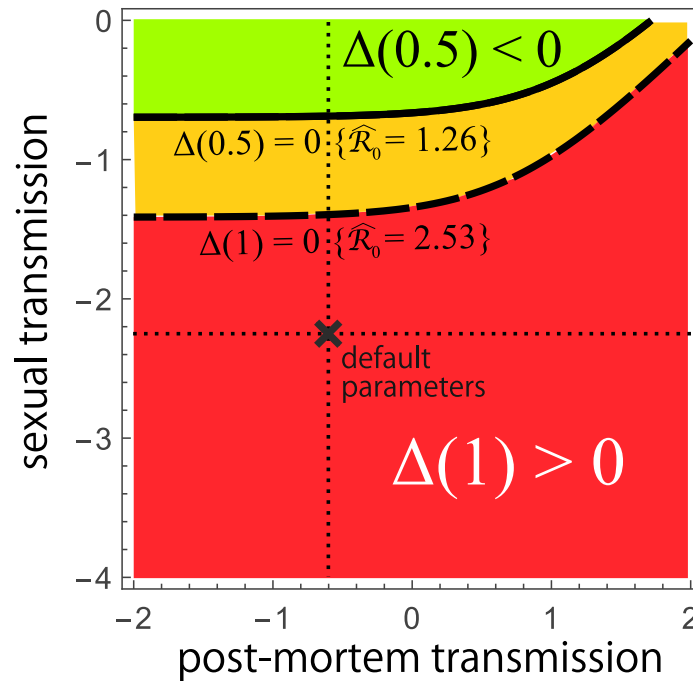
Figure 0.3.3. – Sensitivity analysis of long-term virulence evolution.
