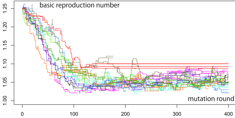
Figure δ.2.10. – Basic reproduction number phylogenetics.
