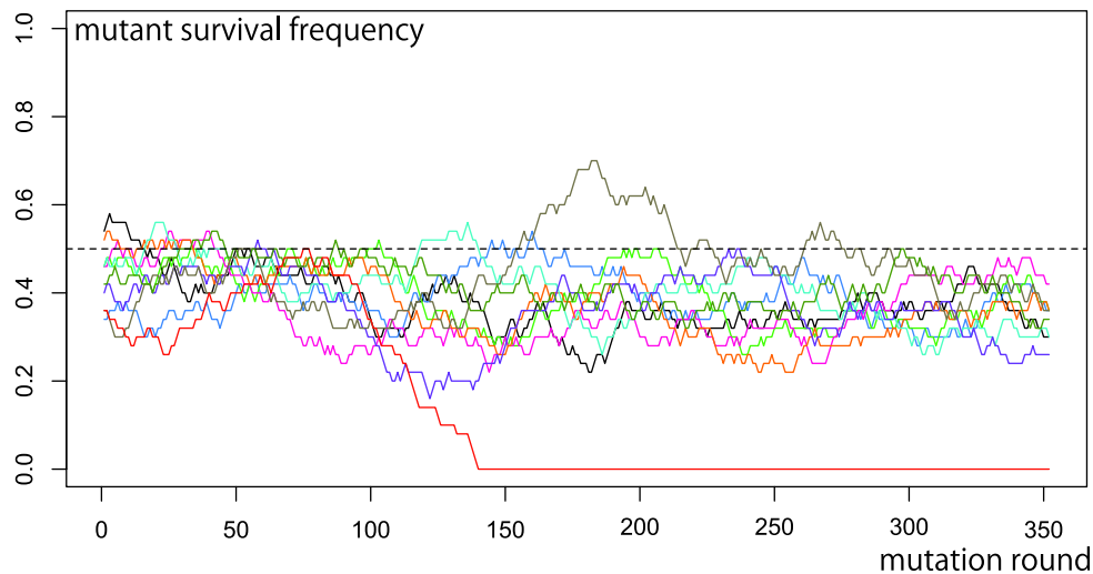
Figure δ.2.4. – Frequency of surviving mutants.
