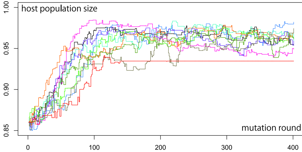
Figure δ.2.12. – Total host population size.
