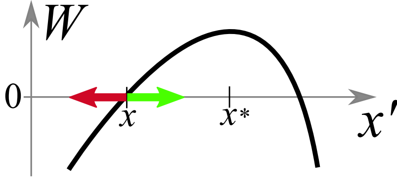
Figure 4.f.1. – Mutant survival in priorinfection.
