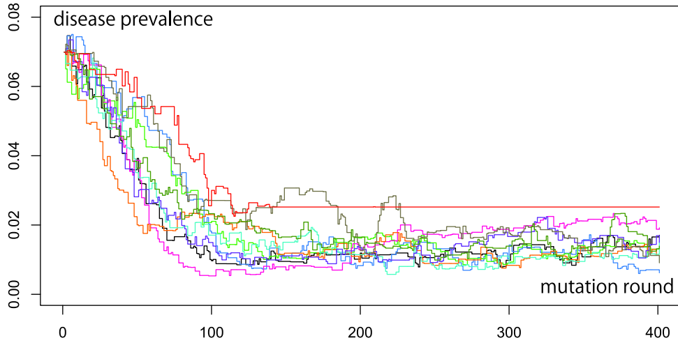
Figure δ.2.13. – Total prevalence.
