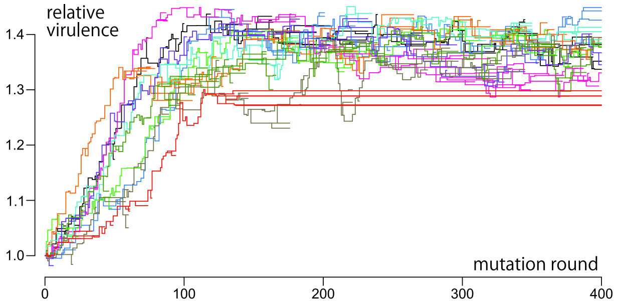
Figure δ.2.3. – Virulence phylogenetics
