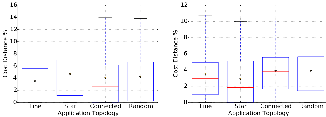
Figure 5.11: Cost distances between 2PCAP and S.A.2, a S.A. implementation that uses 2PCAP to calculate initial solutions. Brown triangles indicate cost distance averages.
