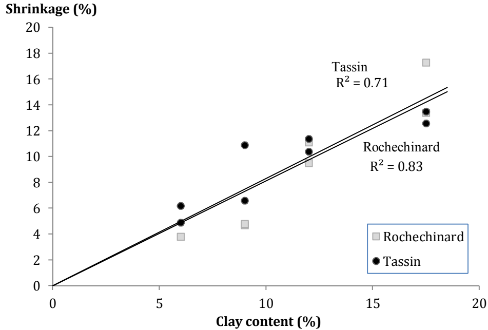
Figure 49. Influence of the clay content on the longitudinal shrinkage of 40×40×160 mm samples. A zero shrinkage is assumed for the 0 % clay content.
