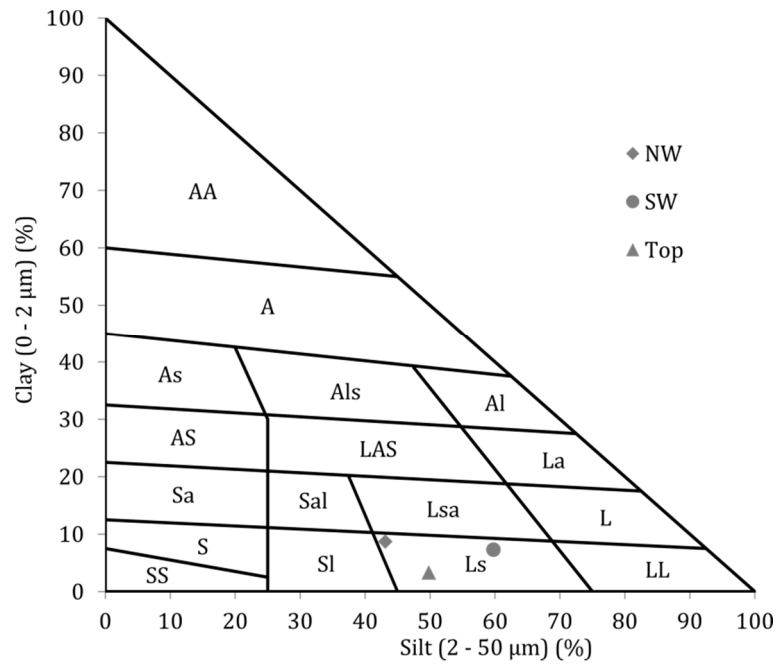
Figure 40. Texture of material collected in north window (NW), south window (SW) and top of the wall (Top) represented in the GEPPA triangle (A = clay, L = silt and S = sand).
