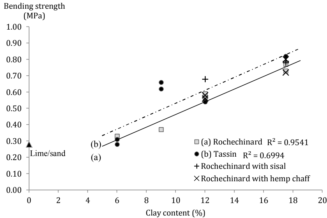
Figure 50. Influence of the clay content on the 3-point bending strength
