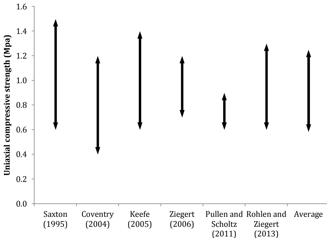
Figure 55. Range of cob compressive strengths found in the literature [12,15,22,35,115,120] and average values.
