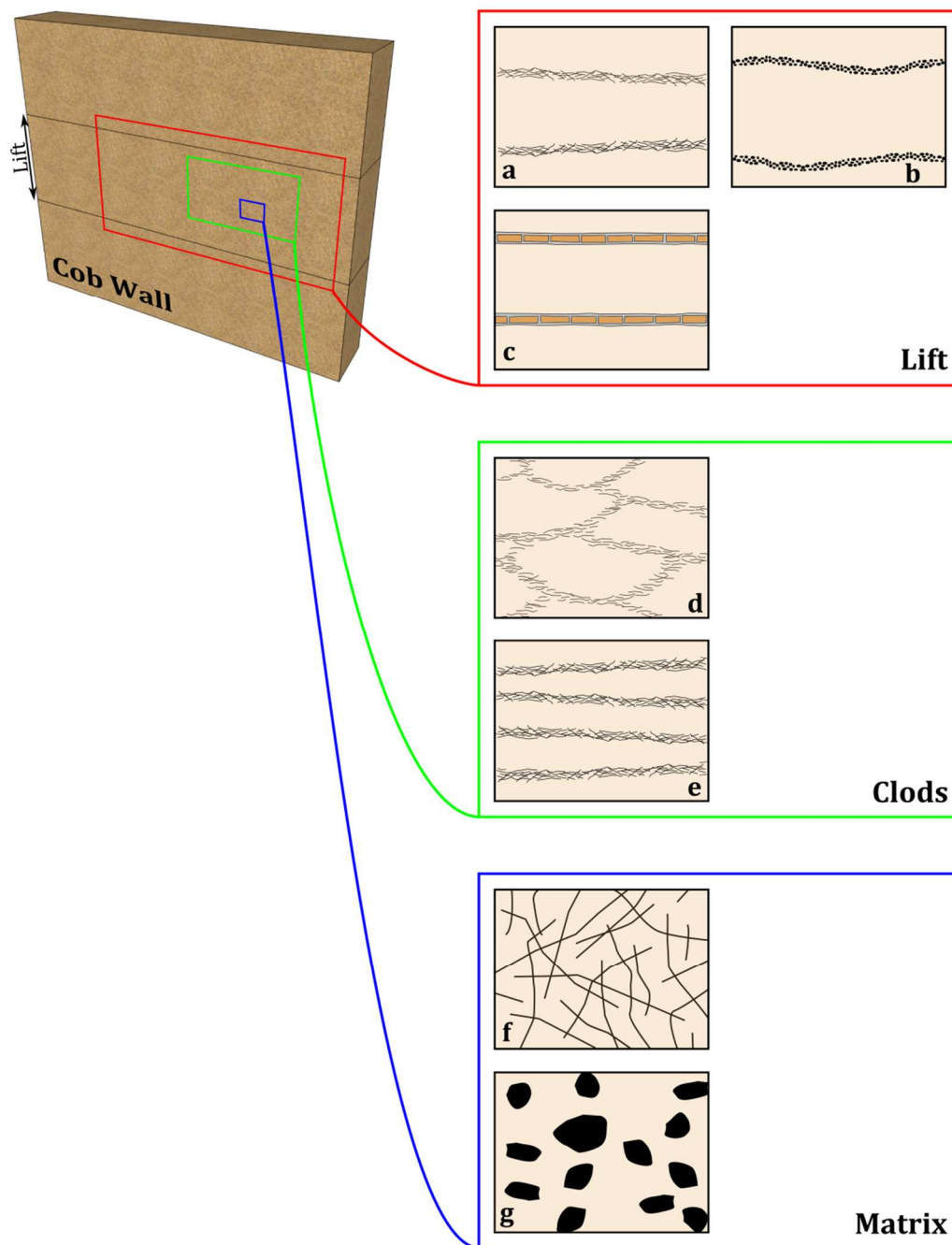
Figure 26. Crack shrinkage barriers placed between lifts (a: layer of fibre or wood, b: layer of stones, c: layer of adobe), between clods of earth (d: between each clod, e: between each layer of clods) or inside the matrix (f: fibres, g: gravels).
