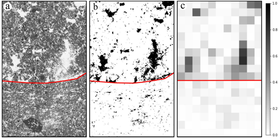
Figure 30. Detail of a rammed earth layer limit, marked with a red line, in grey scale (a), after binarization (b) and in porosity map (c).
