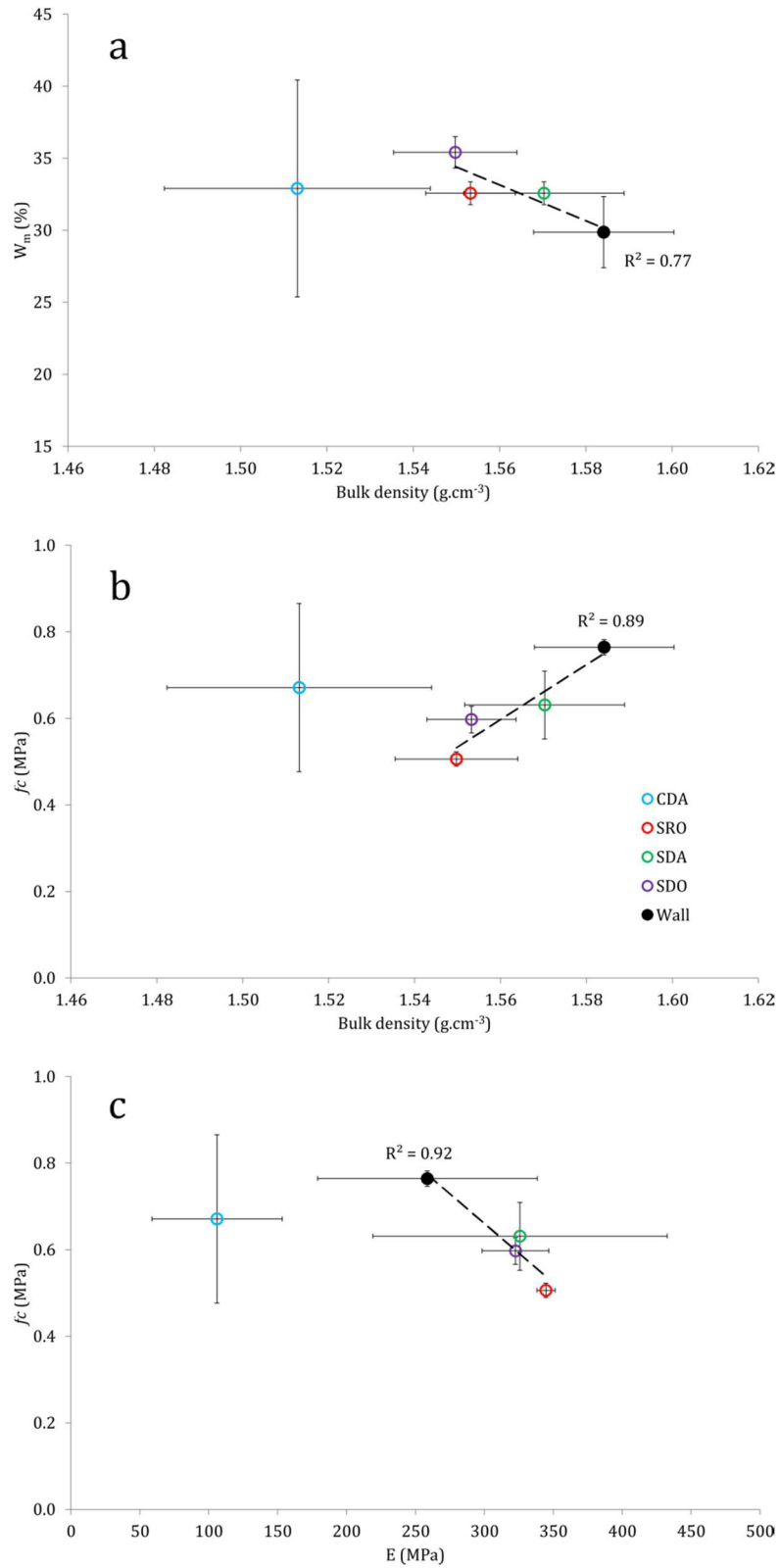
Figure 65. Average water content of manufacturing sae ( W_m ) with respect to average bulk density (a), average compressive strength ( f_c ) with respect to bulk density (b) and average Young's modulus ( E ) with respect to average compressive strength ( f_c ) of cob protocols (c).
