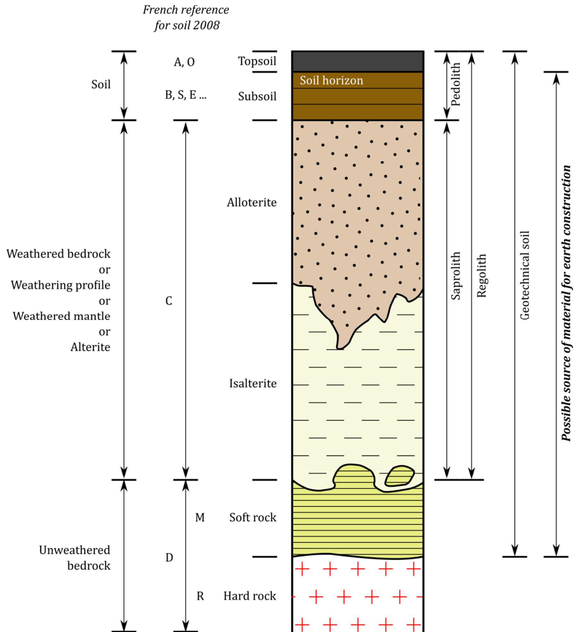
Figure 3. Vertical cross-section of weathered materials from ground surface to unweathered bedrock, according to several disciplines definitions.
