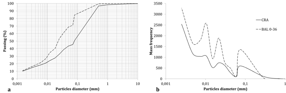
Figure 11. Comparison between particle size distributions and mass frequency of the rammed earth wall material (CRA) and material collected during the Balvay plateau survey, between 0 to 36 cm depth (BAL 0-36).
