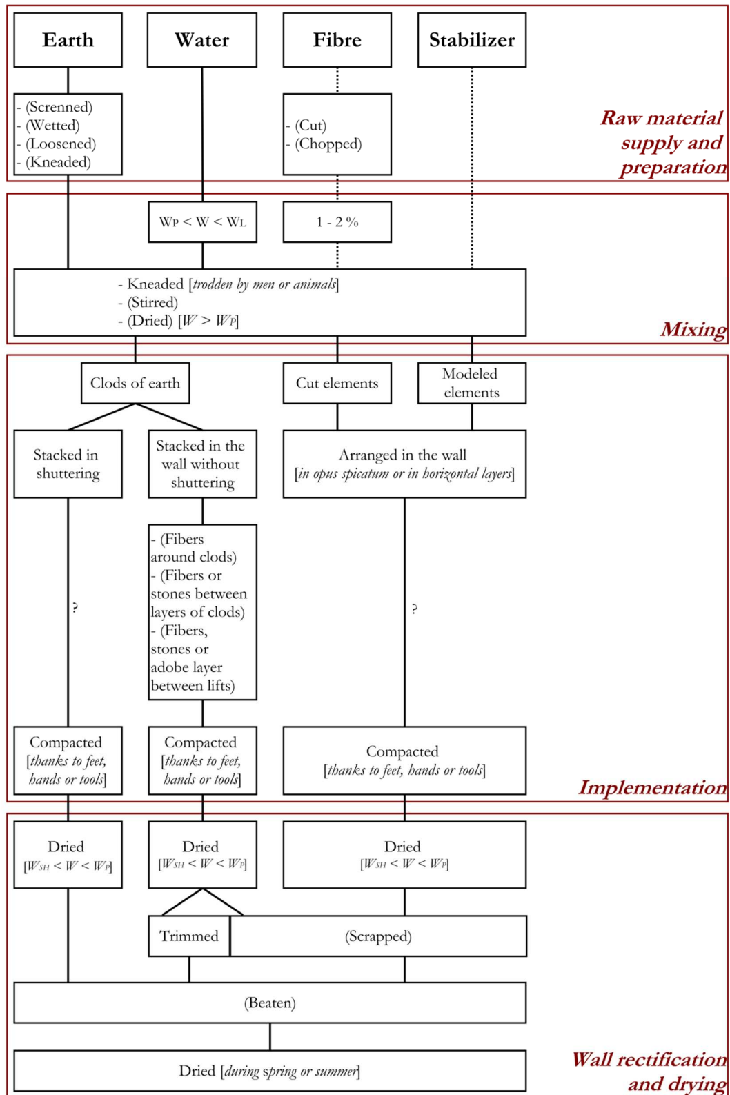
Figure 22. Summary of vernacular cob process. Water contents are to be regarded as order of magnitudes. (elements in brackets are optional; W = water content, WL = water content at liquid limit, WP = water content at plastic limit, WSH = Water content at shrinkage limit).
