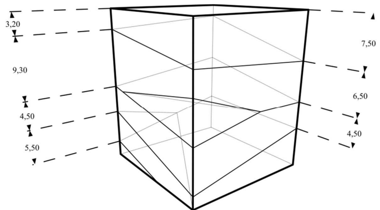
Figure 42. Cob clods limits of a wall portion underlined on a picture (on left) and depicted on a 3-dimension schematic diagram (on right, dimensions in cm).
