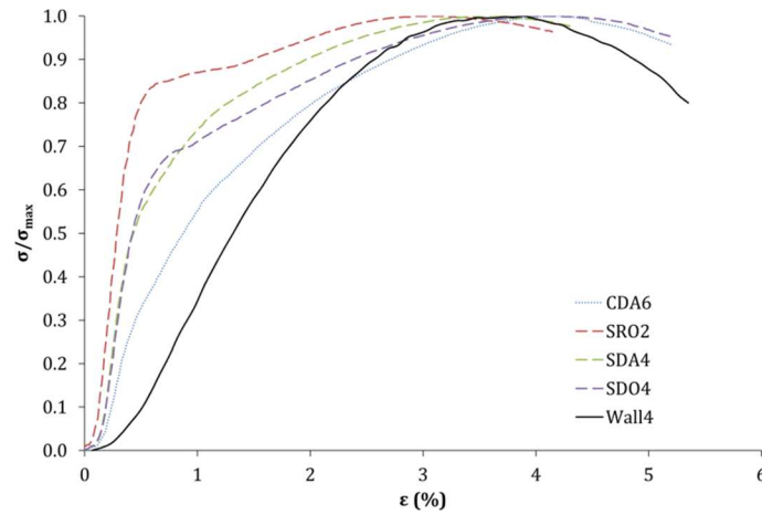
Figure 64. Normalized stress ( \sigma/\sigma_{max} ) strain ( \epsilon ) curve of one specimen of the four cob protocols and cob walls.
