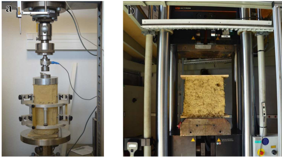
Figure 58. Mechanical tests of cob cylindrical specimens (a) and cob walls (b).
