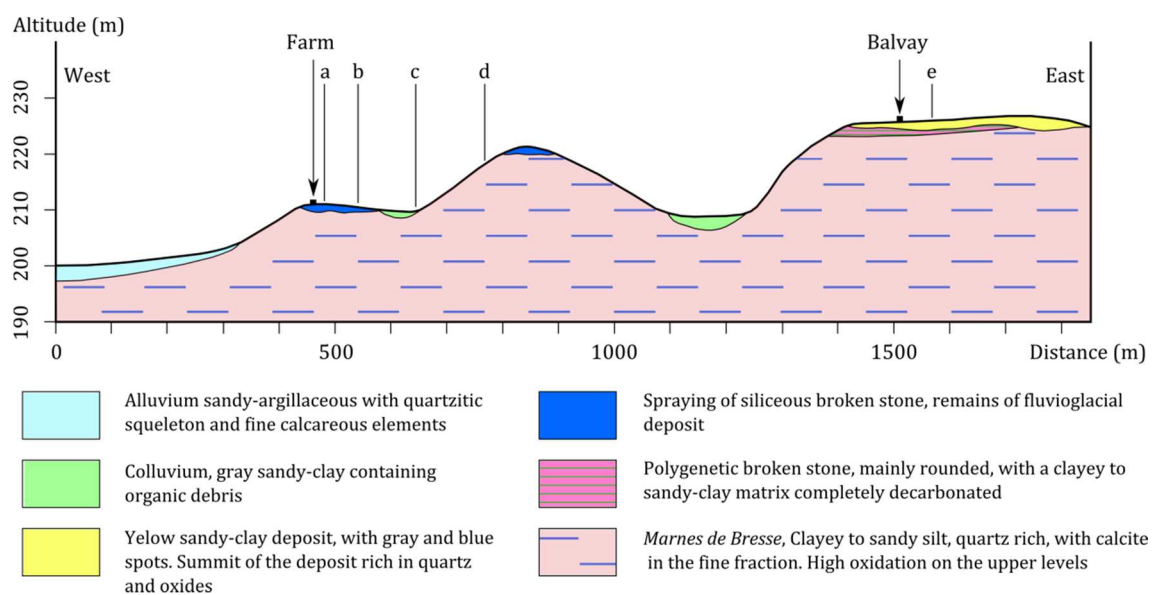
Figure 5. Geological East-West cross section of the surroundings of the rammed earth farm performed according to the geological map (Bergerat and Fleury 1985). Positions of pedological surveys are indicated (a, b, c, d and e).
