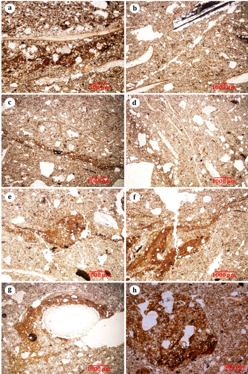
Figure 46. Fabric pedofeatures: subhorizontal limits (a, b and c) and oblique limit (d) underlined by sand alignments stems and voids parallel to the limits, deformed soil aggregates (e, f and g) and round aggregate (h). All pictures are taken in PPL.
