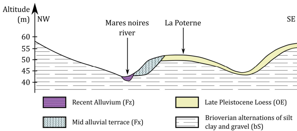
Figure 35. Geological cross section of the locality of "La Poterne", located on the city of Saint Gilles.
