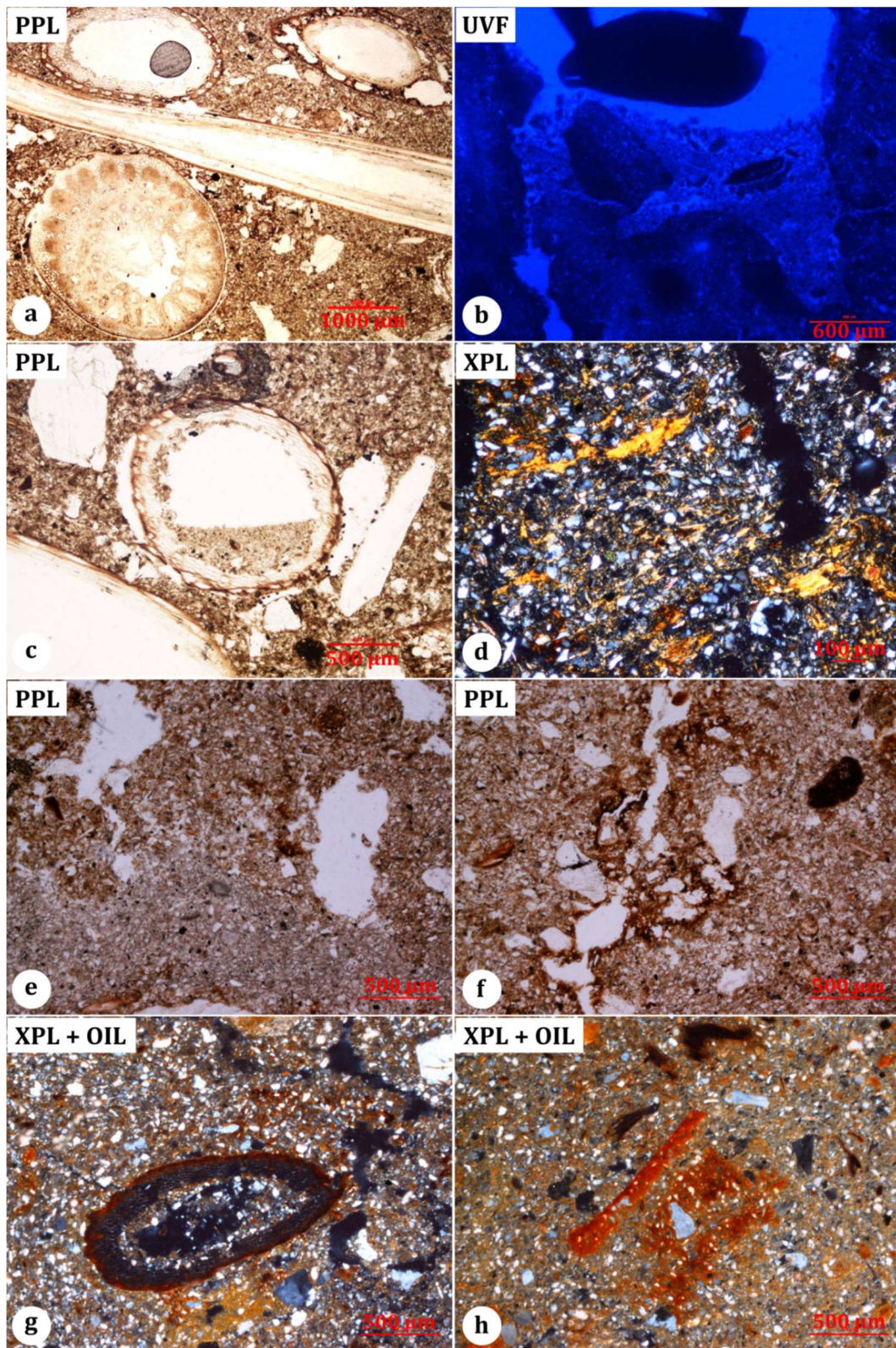
Figure 45. Microscope picture of a: stem residues; b: void coating; c: silty coating in the section of a stem; d: intercalations; e: clay depletion at the lower part of the photo; f: voids coating and hypo-coatings; g: stem internal/external hypo-coatings; h: Fe/Mn groundmass impregnations.
