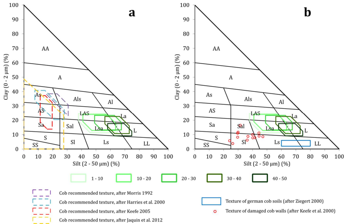
Figure 19. Confrontation of texture of fine earth identified as suitable for vernacular cob construction in Brittany with, a: cob recommended texture available in the literature [13,22,121,122], and b: texture of fine earth of German cob soils [155] and damaged cob walls built with soils derived from Permo-Triassic rocks [123]. Data are projected in the texture triangle of reference for French soils, defined by the GEPPA (A = clay; L = silt; S = sand). In this representation, regardless of the gravel content, sum of clay, silt and sand content is 100%.
