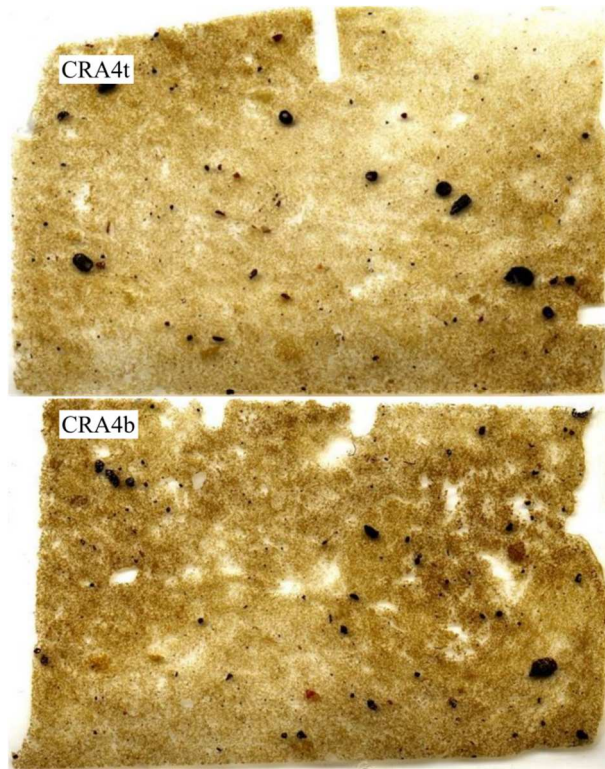
Figure 33. Effect of thin section thickness on brightness
