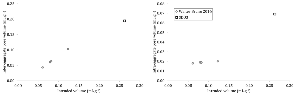
Figure 62. Comparison of inter and intra aggregate pore volume of hypercompacted earth blocks [358] with SDO3
