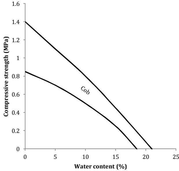
Figure 56. Variation in compressive strength against water content, after Saxton [120]
