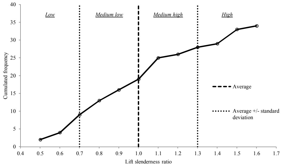
Figure 24. Cumulated frequency of lifts slenderness ratio together with average slenderness ratio (1.0 with standard deviation of 0.3) and average +/- standard deviation. Slenderness ratio are divided into 4 classes : Low (< 0.7), Medium low (0.7 - 1.0), Medium high (1.0 - 1.3) and High (> 1.3).
