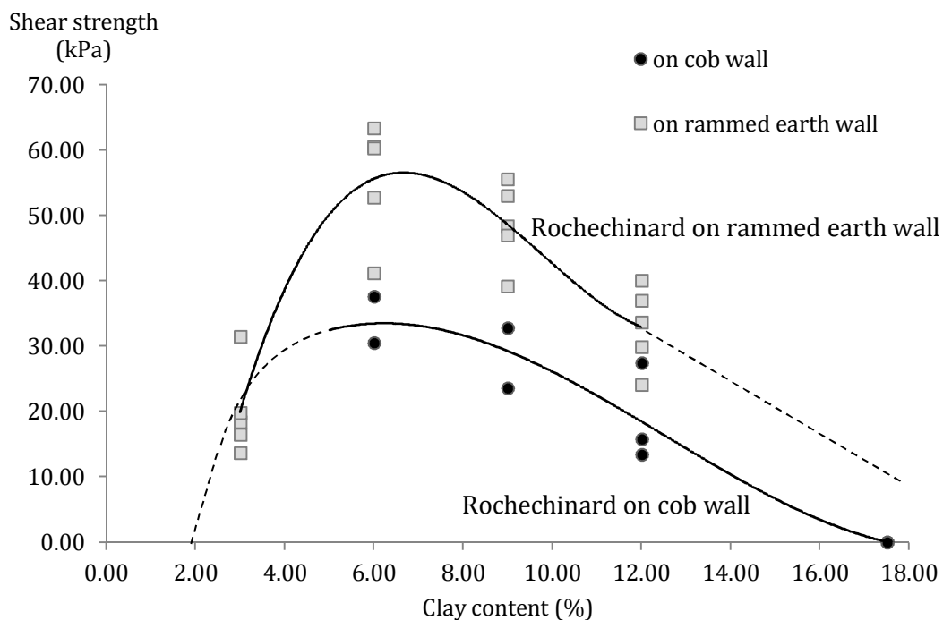
Figure 51. Shear strength vs. clay content of the Rochechinard specimens from the cob and rammed earth walls. Rochechinard data from the rammed earth blocks and cob wall are represented using a 3-degree polynomial function. As the 18 % clay content shrinkage specimen had fallen from the cob wall, the shear strength is assumed to be zero.
