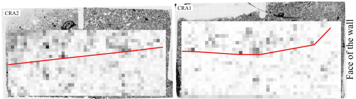
Figure 31. Horizontal section of rammed earth wall after image analysis. A continuous limit (red line) is identified through CRA1 and CRA2 thin section.
