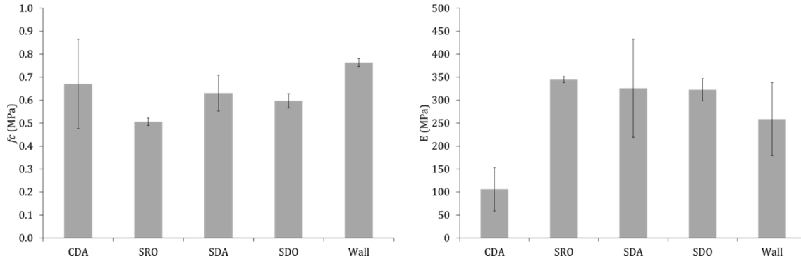
Figure 63. Comparison of average compressive strength ( f_c on left) and average Young's moduli ( E , on right) for the four cob specimen protocols and cob walls.
