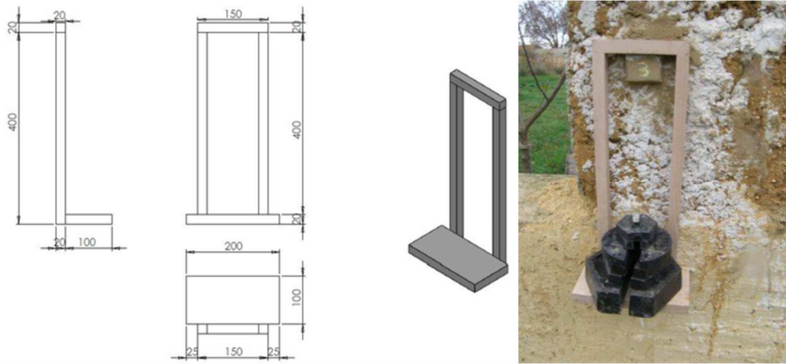
Figure 47. Shear test loading device example, 400 mm high, 150 mm large and 20 mm thick.
