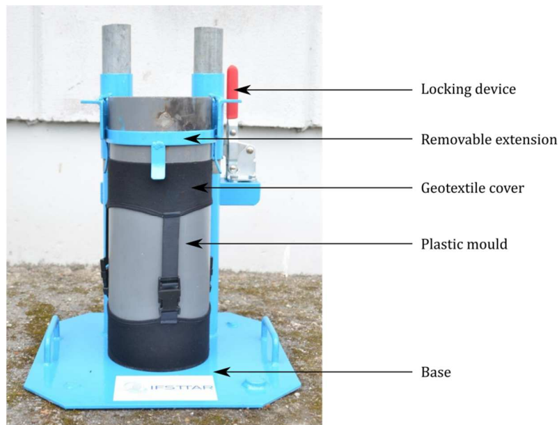
Figure 57. Device for cob specimen production.
