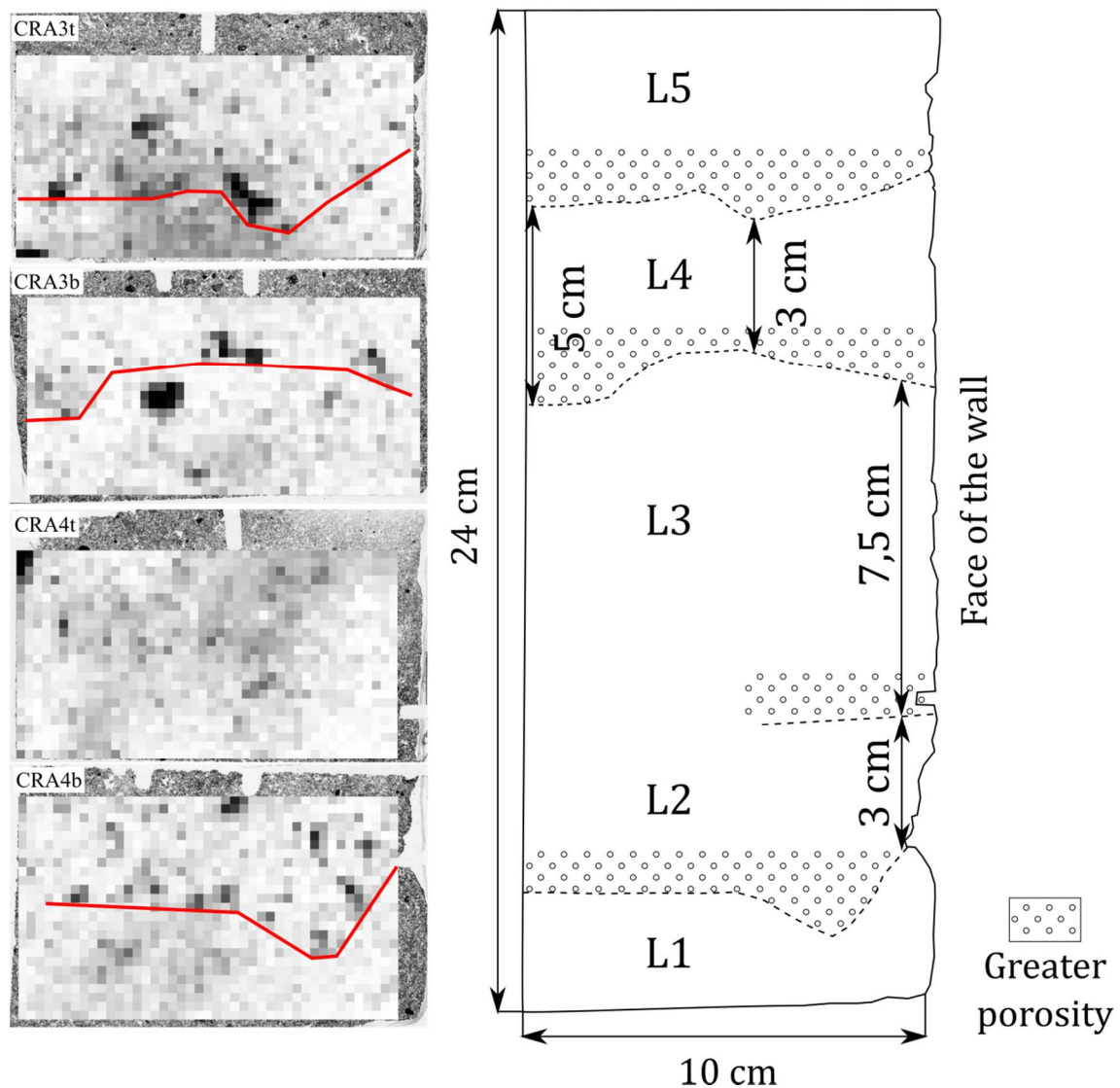
Figure 32. Vertical section of rammed earth wall after image analysis, on left, together with micromorphological analysis results, on right. Three of the four rammed earth layers limits observed by microscope can be detected by image analysis (red lines).
