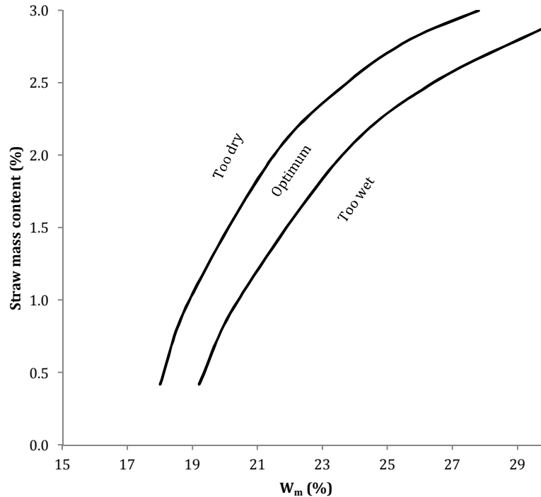
Figure 54. Optimal cob mixture with regard to water content of manufacturing stage ( W_m ) and straw content, after [120]
