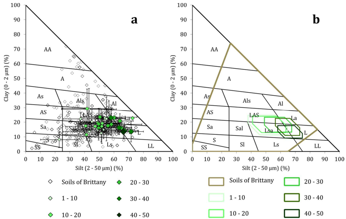
Figure 17. Texture of fine earth of strata of Brittany according to their cob frequency in percentage. Strata values are presented on a (diamond are mode values and error bars are estimated confidence interval) and frequency classes values, calculated according to section 2.4.3.1 are shown on b. Data are projected in the texture triangle of reference for French soils, defined by the GEPPA (A = clay; L = silt; S = sand). In this representation, regardless of the gravel content, sum of clay, silt and sand content is 100%.
