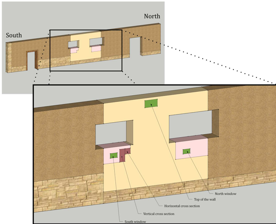
Figure 36. View of the three different construction stages (north, middle and south) identified in the wall, seen from the inside of the building. Sampling concerned the middle stage (in yellow): rose parts were collected, with particular samples for thin sections (red) and material identification (green).
