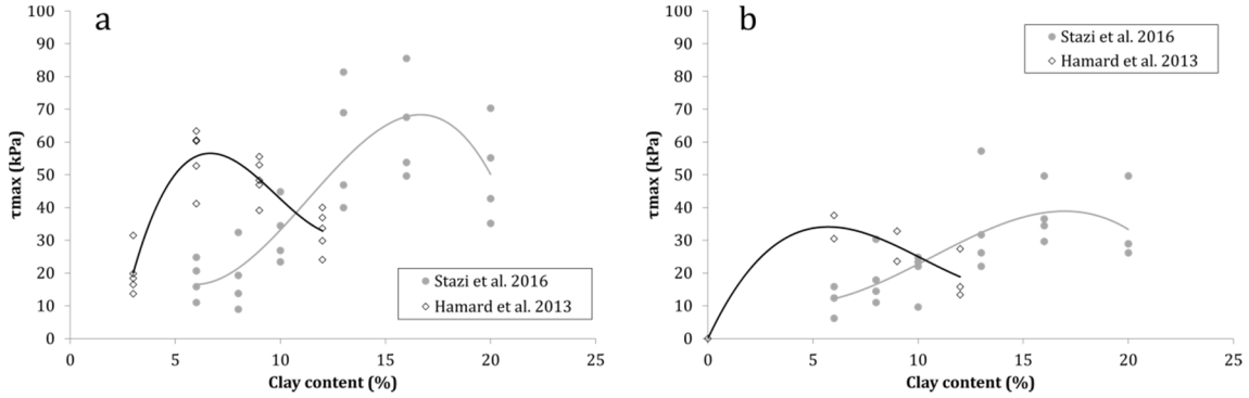
Figure 52. Comparison of shear test results of [306] and [345] performed on rammed earth wall (a) and cob wall (b)
