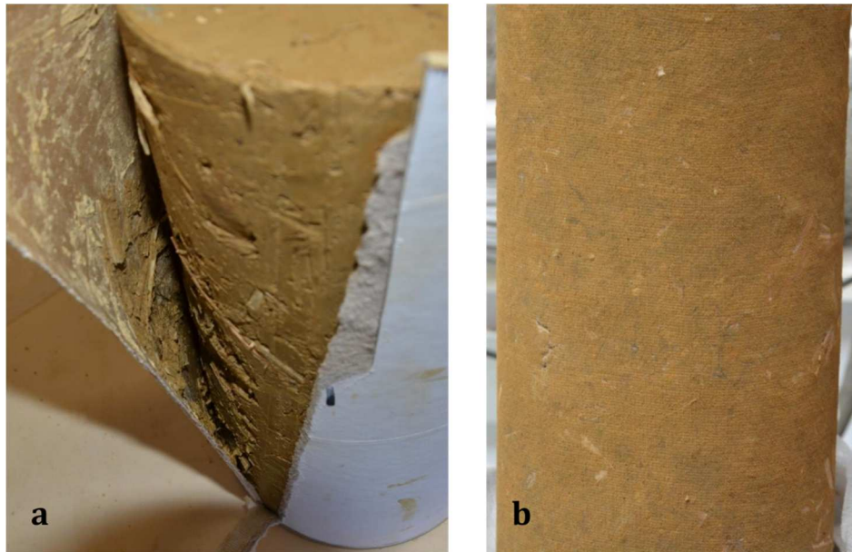
Figure 59. Surface state of specimens made in concrete mould (a) and in plastic mould with a flexible geotextile cover (b).
