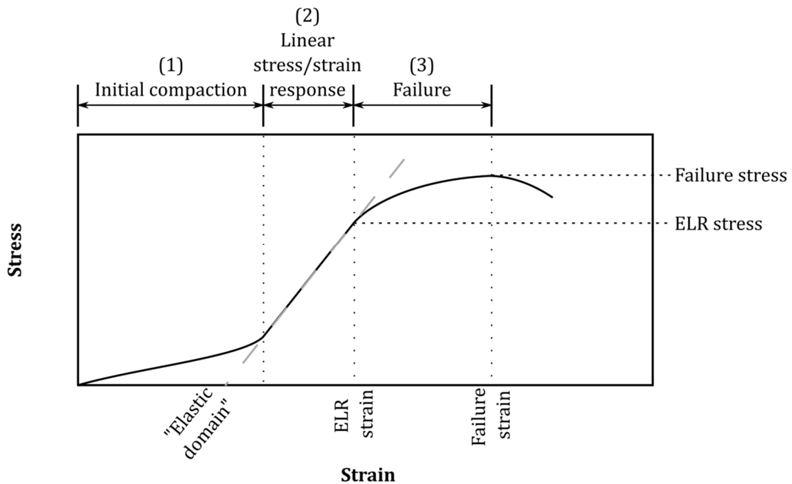
Figure 53. Typical cob Uniaxial Compressive Strength test (ELR = End of Linear stress/strain Response), after [252].
