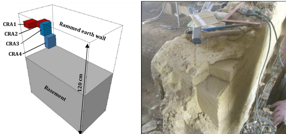
Figure 8. 3-dimension drawing of the 4 specimens sampling performed in the rammed earth wall (on left) and picture of the wall after sampling (on right).
