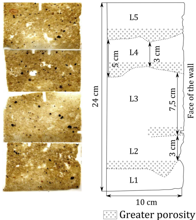
Figure 10. Vertical cross section, reconstructed thanks to 4 thin sections (CRA3t, CRA3d, CRA4t and CRA4d). Obvious limits are pictured by dotted lines. Obvious limits separate 5 layers, named L1 to L5, wherein porosity transition is underlined.
