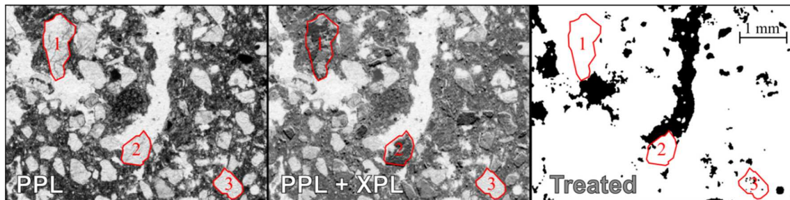
Figure 29. Result of image processing on a thin section thumbnail. Three different quartz minerals (1, 2 and 3) are outlined.
