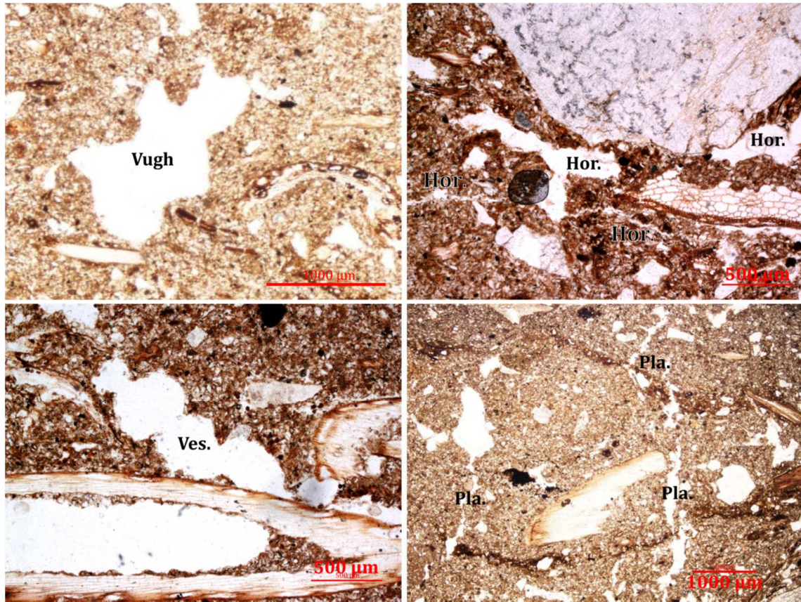
Figure 44. Microscope pictures of voids type: Vugh = random vughs; Hor. = horizontal vughs; Ves. = vesicles; Pla. = vertical planar voids.
