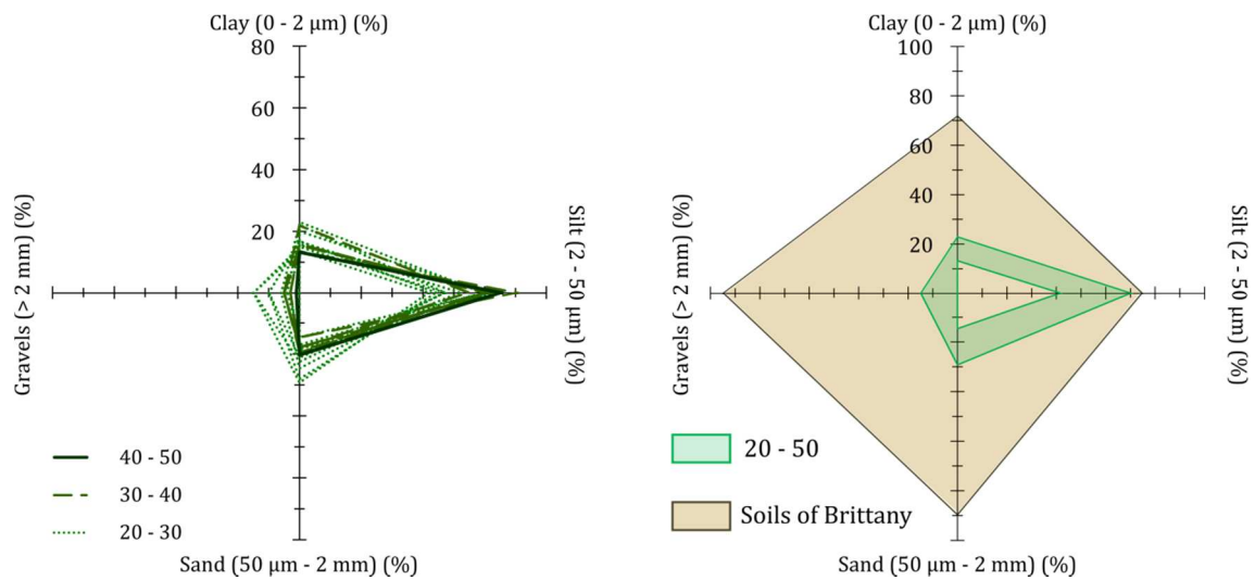
Figure 16. Texture of soils of 40-50 %; 30-40 % and 20-30 % cob frequency classes (left) and comparison of these textures (20-50 % cob frequency) with all soils of Brittany (right). The coloured surfaces of the radar graphical representation allow an easy comparison between recommended textures, but only the extremum clay, silt, sand and gravel contents are to be considered.
