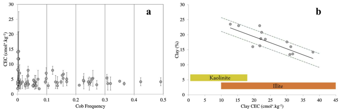
Figure 20. a: Cation Exchange Capacity (CEC) of strata of Brittany plotted against cob frequency, b: clay content of strata with a 20-50 % cob frequency plotted against the CEC of clay fraction (on right). A linear relationship is proposed between Clay content (CLAY) and Cation Exchange Capacity of Clay (CL_CEC) for cob in Brittany with a correlation coefficient of 0.78 and a standard error of 2.3. The solid line depicts this relationship and dotted lines depict the standard error.
