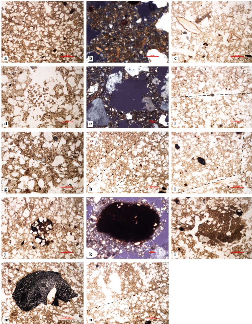
Figure 9. Details of thin sections. a: coarse texture (PPL, \times 2 ) (CRA1); b: fine texture (XPL, \times 20 ) (CRA1); c: vegetal debris (PPL, \times 2 ) (CRA4t); d: porosity of type 1 containing Enchytraeids excretions (PPL, \times 2 ) (CRA4t); e: porosity of type 2 (XPL, \times 10 ) (CRA3t); f: horizontally elongated cavity (PPL, \times 2 ) (CRA4t); g: flattened cavities alignment (PPL, \times 4 ) (CRA2); h: tilted sand particles alignments (PPL, \times 2 ) (CRA4t); i: subhorizontal associated to a subvertical sand particles alignment (PPL, \times 2 ) (CRA3t); j: sharp shape ferruginous nodule (PPL, \times 2 ) (CRA2); k: indistinct shape ferruginous nodule (XPL, \times 20 ) (CRA3t); l: silty-clayey aggregate (PPL, \times 2 ) (CRA3t); m: piece of charcoals (PPL, \times 2 ) (CRA4t); n: detail of an obvious limit, between a low porosity layer below and a high porosity layer above. This limit is underscored by a subhorizontal sand particles and flattened voids alignment (PPL, \times 2 ) (CRA3t).
