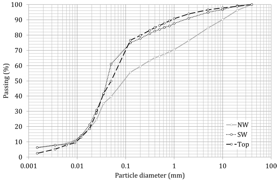
Figure 39. Particle size distribution of material collected in north window (NW), south window (SW) and in top of the wall (Top)
