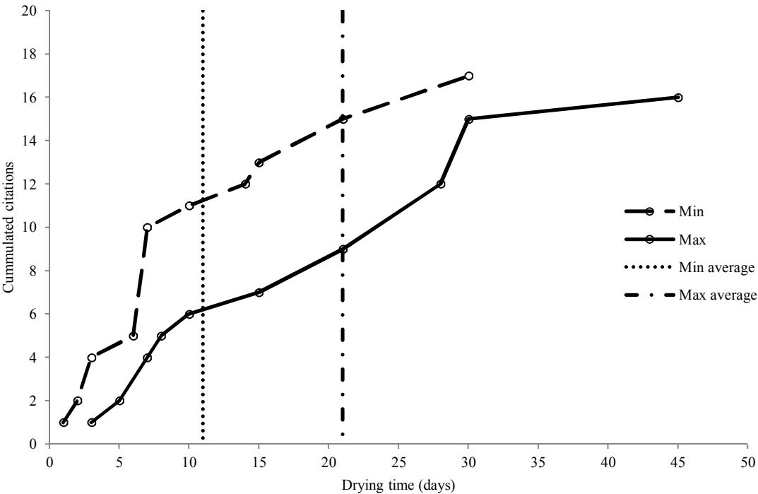
Figure 25. Cumulated citations of minimum (Min) and maximum (Max) drying time of cob lifts, together with calculated average minimum drying time (Min average) and average maximum drying time (Max average) of cob lifts.
