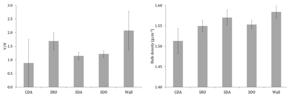
Figure 60. Comparison of average ratio of vertical by horizontal shrinkage ( V/H ), on left, and average bulk density, on right.
