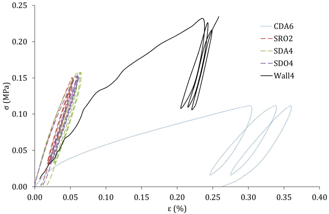
Figure 66. Cyclic loadings performed for modulus assessment
