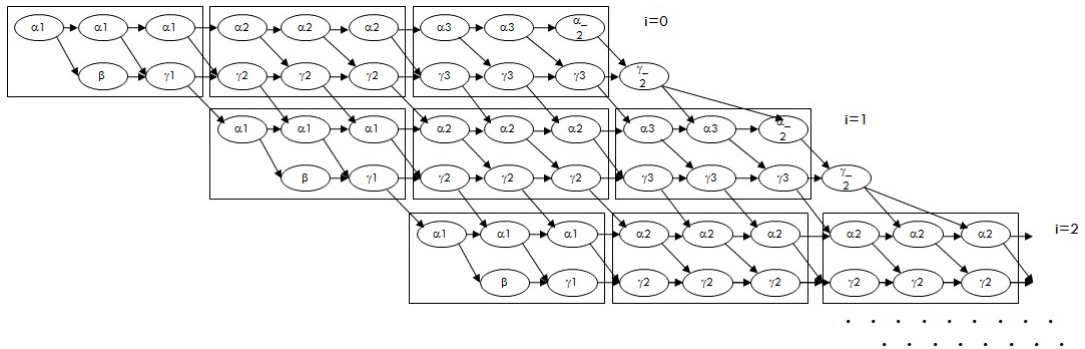
FIGURE C.11 – The data dependency graph of the proposed new Systolic Architecture with a Tow-dimensional array of Processing Elements (NW-8).
