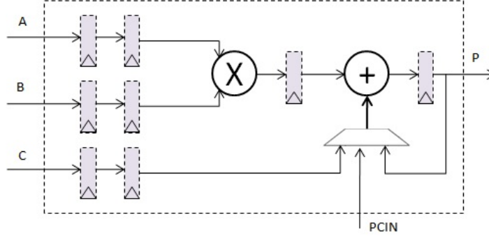
FIGURE C.1 – Structure of DSP block in modern FPGA device.
