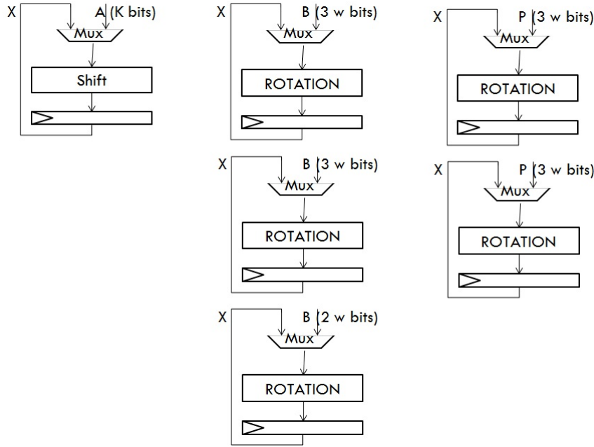
FIGURE C.12 – Internal architectures - Rotations.
