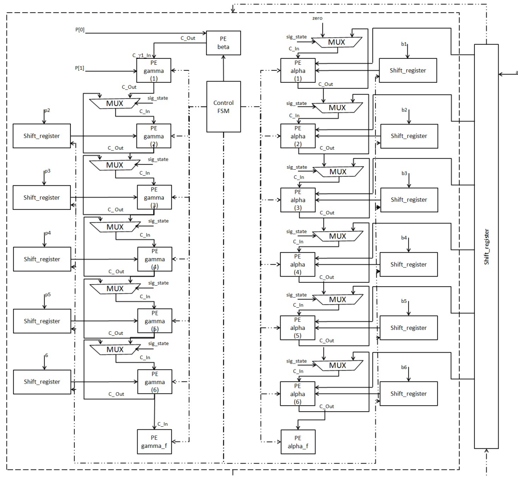
FIGURE C.14 – Proposed Montgomery modular multiplication architecture for the NW-16 version.
