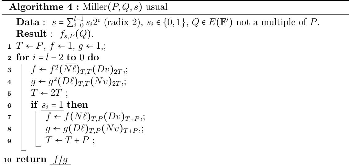
FIGURE A.1 – The usual Miller algorithm
