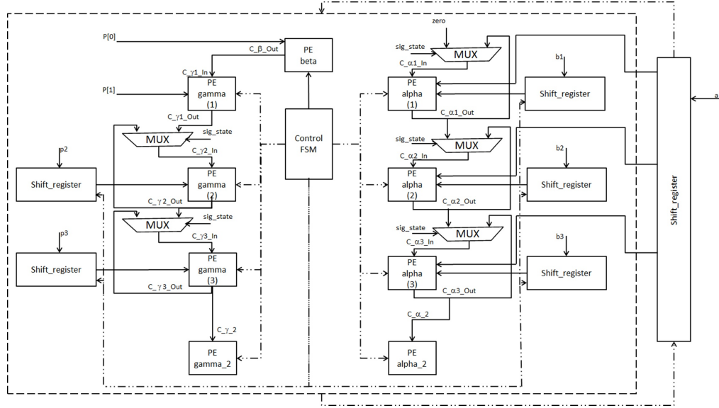
FIGURE C.10 – Proposed Montgomery modular multiplication architecture.
