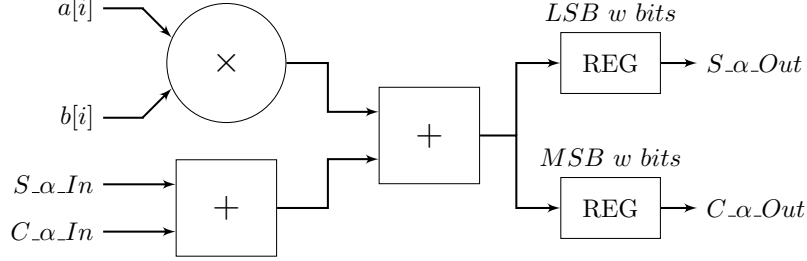
FIGURE C.4 – Alpha Processing Element internal architecture.
