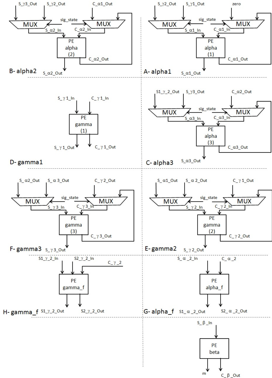
FIGURE C.25 – All Processing Elements.
