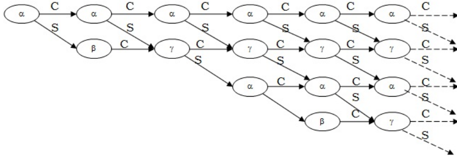
FIGURE C.2 – data dependency in general systolic architecture.
