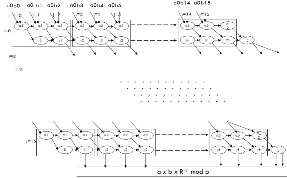
FIGURE C.15 – The data dependency graph of the proposed new Systolic Architecture with a Tow-dimensional array of Processing Elements (NW-16).
