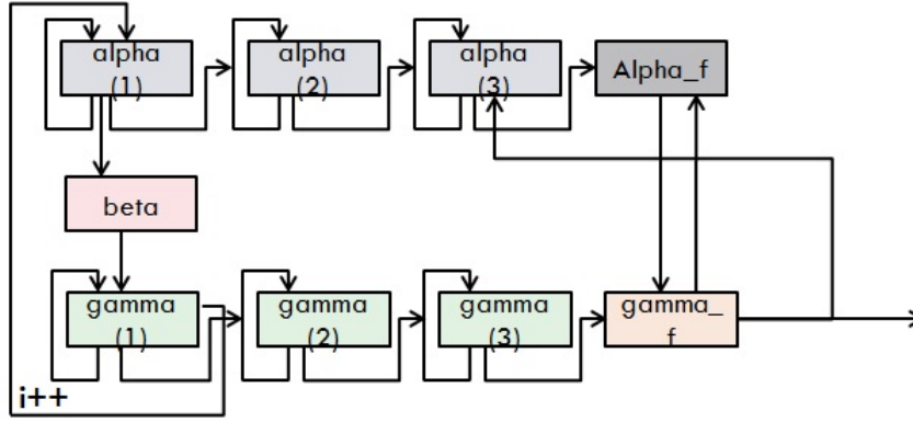
FIGURE C.9 – CIOS NW-8 Architecture.
