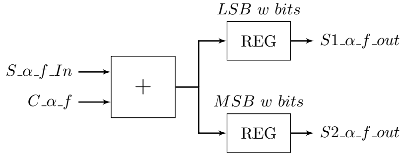
FIGURE C.7 – Alpha_f Processing Element internal architecture.
