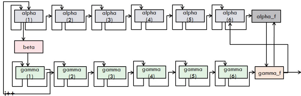
FIGURE C.13 – CIOS NW-16 Architecture.
