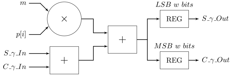
FIGURE C.6 – Gamma Processing Element internal architecture.
