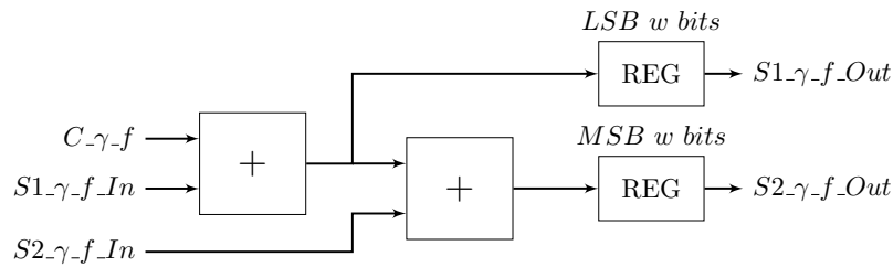
FIGURE C.8 – Gamma_f Processing Element internal architecture.
