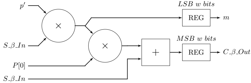
FIGURE C.5 – Beta Processing Element internal architecture.
