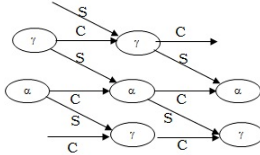
FIGURE C.3 – PEs of Systolic Architecture in two-dimensional array.
