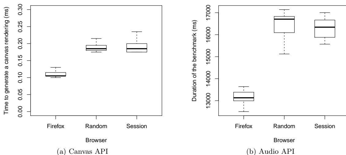
Figure 4.10: Benchmarking results
