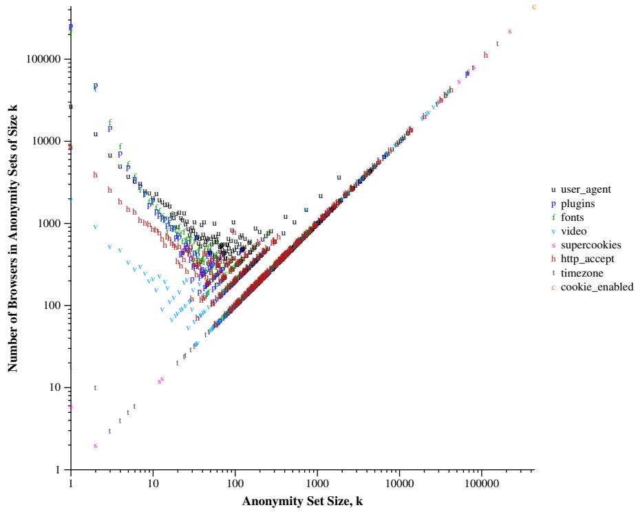
(a) Panopticklick distribution (Fig. 3 of [72])
