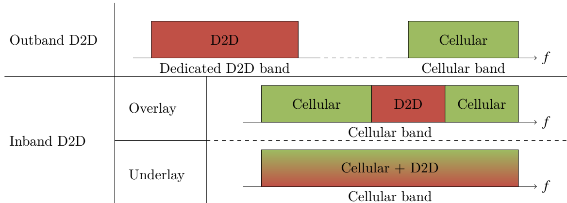
Figure 2.11: Typical classification of D2D spectrum allocation schemes [49]. Outband D2D is out of the scope of this thesis and our work will focus on inband D2D.
