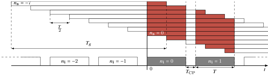
Figure 4.5: Time axis view of the interference caused by an OFDM/OQAM transmission on CP-OFDM receiving windows n_i = 0 and n_i = 1 .
