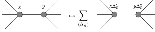
Figure 3.5.1: The splitting differential of \text{SGra}_{R, \Omega^*(\partial M)} (a gray vertex can be of any kind).
