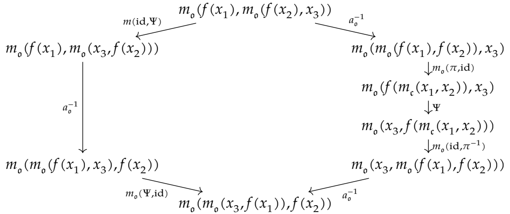
Figure 1.3.6: F is monoidal w.r.t. half-braidings
