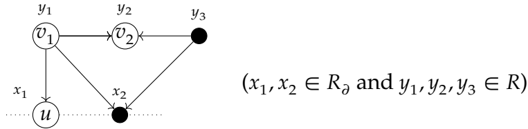
Figure 3.5.2: A colored labeled graph in \text{Tw SGr}_{R,\Omega^*(\partial M)}(\{u\}, \{v_1, v_2\}) .
