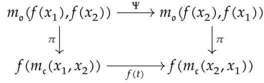
Figure 1.3.5: F is braided
