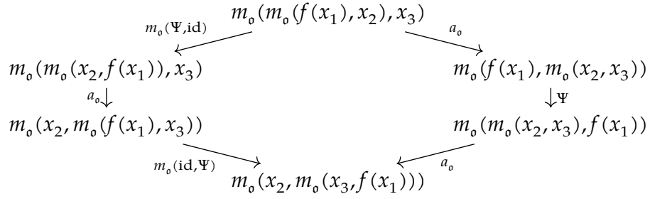
Figure 1.3.4: \Psi is a half-braiding
