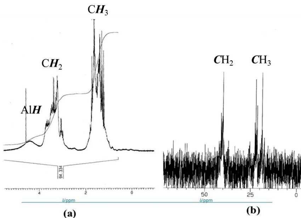
Figure II-2: Liquid-state NMR spectra of PEIA (a) 1 H and (b) 13 C.
