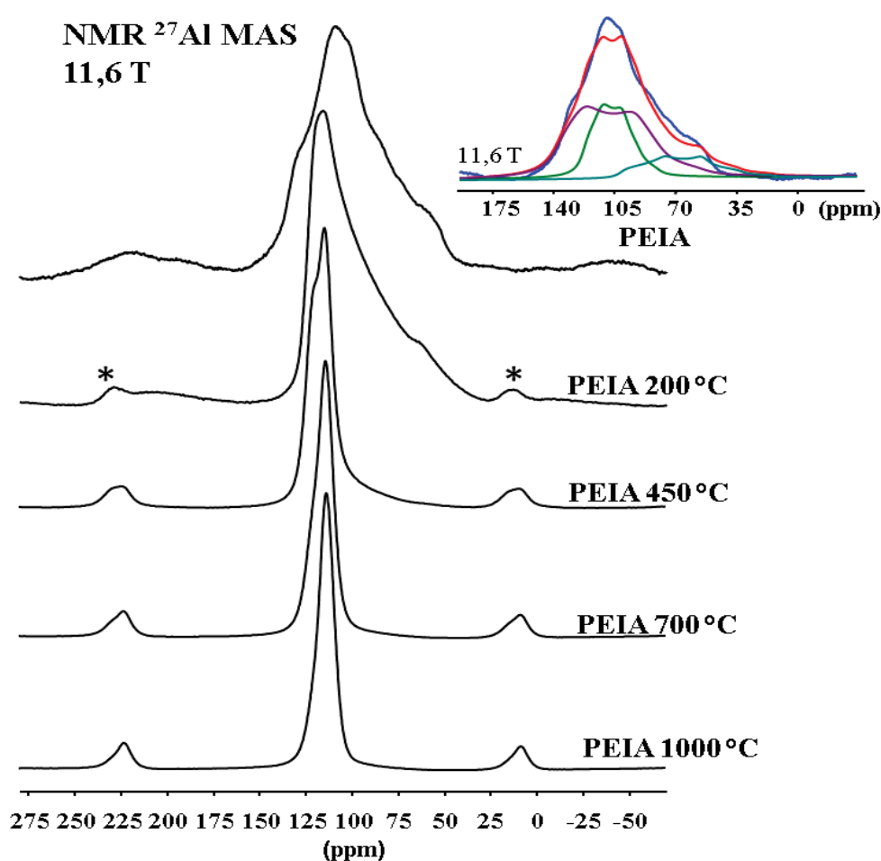
Figure II-7: 27 Al MAS NMR spectra of PEIA and NH 3 -treated intermediates. Spinning side bands are marked with asterisks [125].
