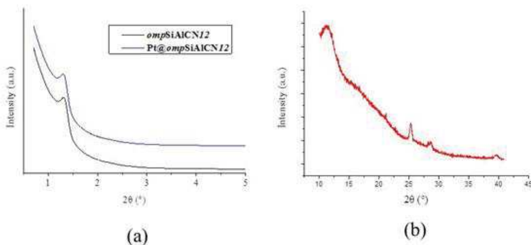
Figure IV-23: Pt@ompSiAlCN12: a) SA-XRD and b) Wide angle XRD.
