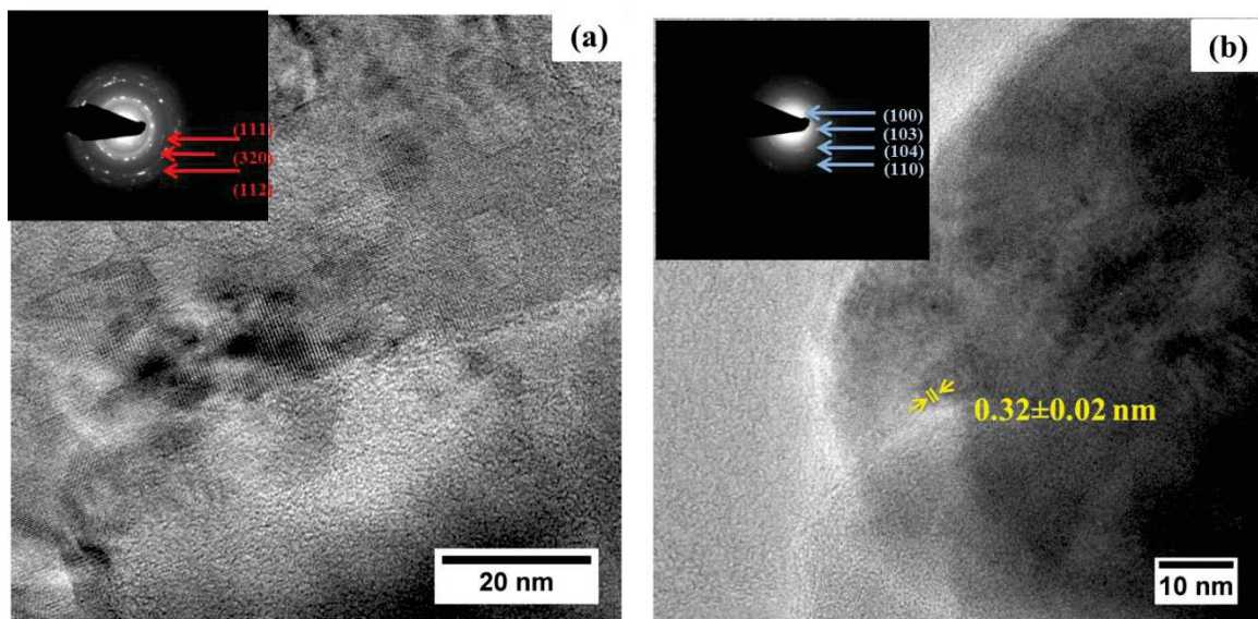
Figure V-20: TEM images of PMVAZ-d-SiAlCN at 1600°C in \text{N}_2 atmosphere.
