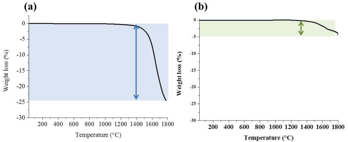
Figure V-29: HTTGA curve of (a) PAAZ30/PMMA70-80-74-1000°C and (b) PAAZ-1000°C under N 2 up to 1800°C with a heating rate of 5°C.min -1 .
