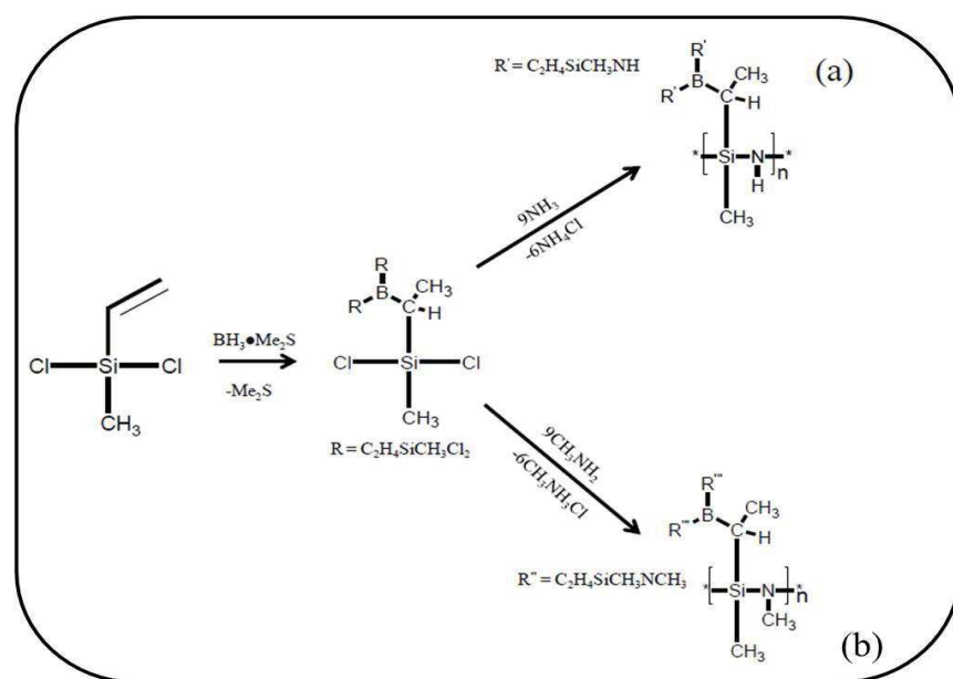
Figure I-23: Synthesis of polyborosilazane: monomer route.
