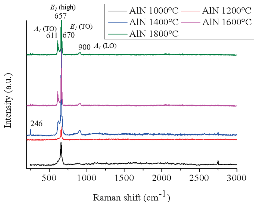
Figure II-10: Raman spectra of PEIA-1000 between 1000 and 1800°C under N 2 .
