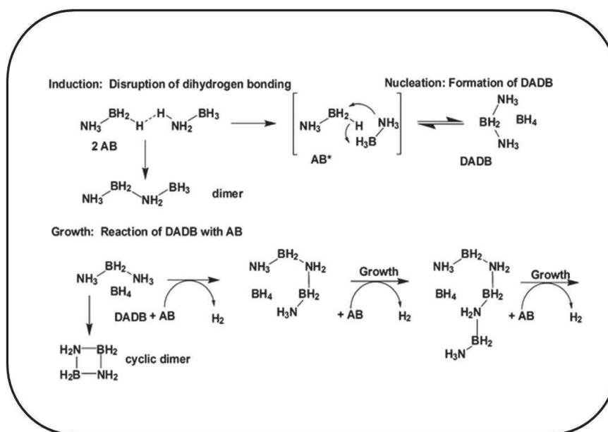
Figure I-5: Thermal dehydrogenation mechanism of AB [60].
