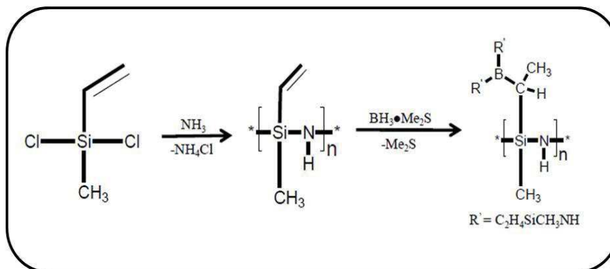
Figure I-24: Synthesis of polyborosilazane: polymer route.
