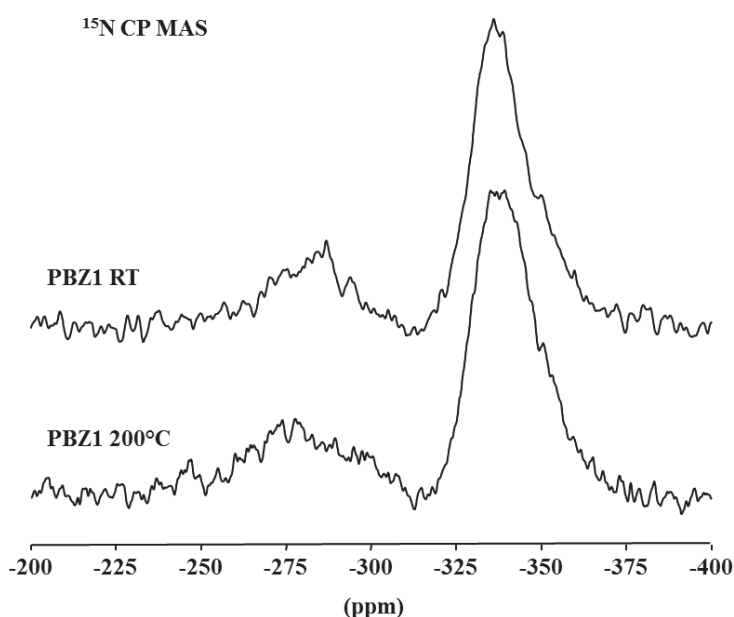
Figure V-40: ^{15}N CP MAS NMR spectra of PBZ1(1.2) and N_2 -treated intermediate at 200°C.
