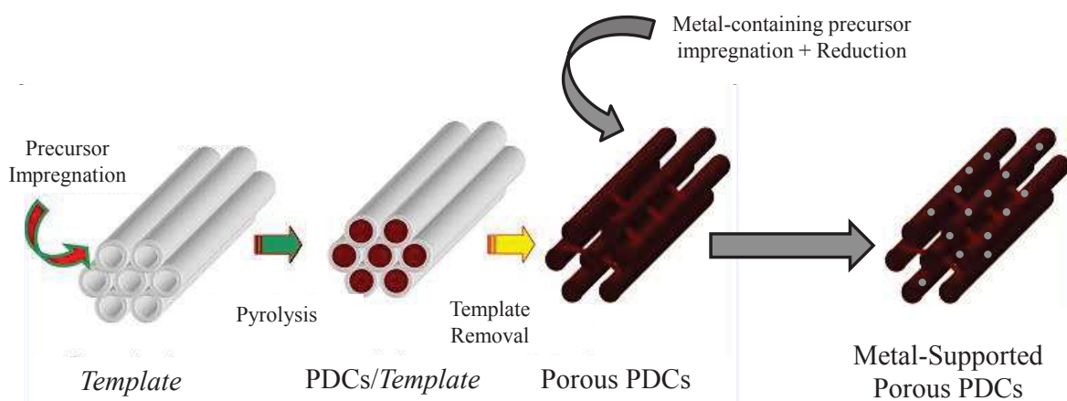
Figure IV-4: Two-step procedure to prepare metal-supported PDCs [223, 225].
