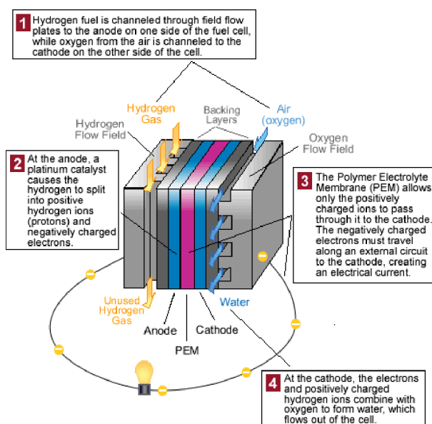
Figure IV-1: PEMFC system [278].
