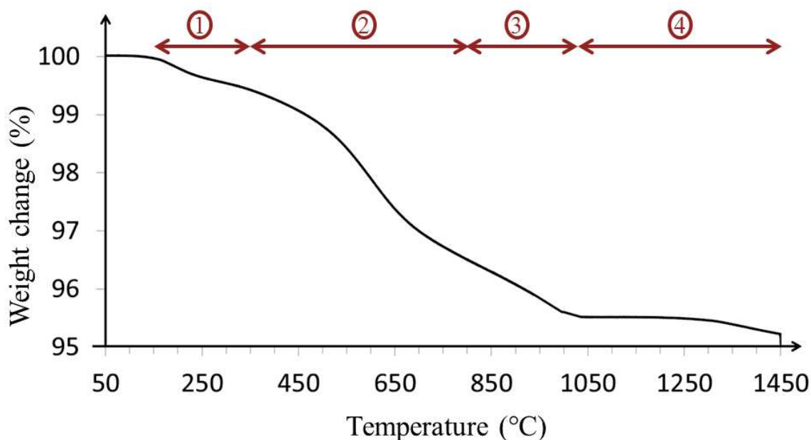
Figure III-3: TGA curve of the 4-step decomposition of PB up to 1450°C in N 2 atmosphere (dwelling time: 5°C.min -1 ).
