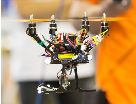
(a) AeCa robot version 1.0 (Top located actuators).
