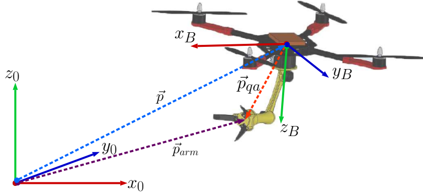
Figure 4.1 – 3d projection of the quadrotor and the manipulator arm.
