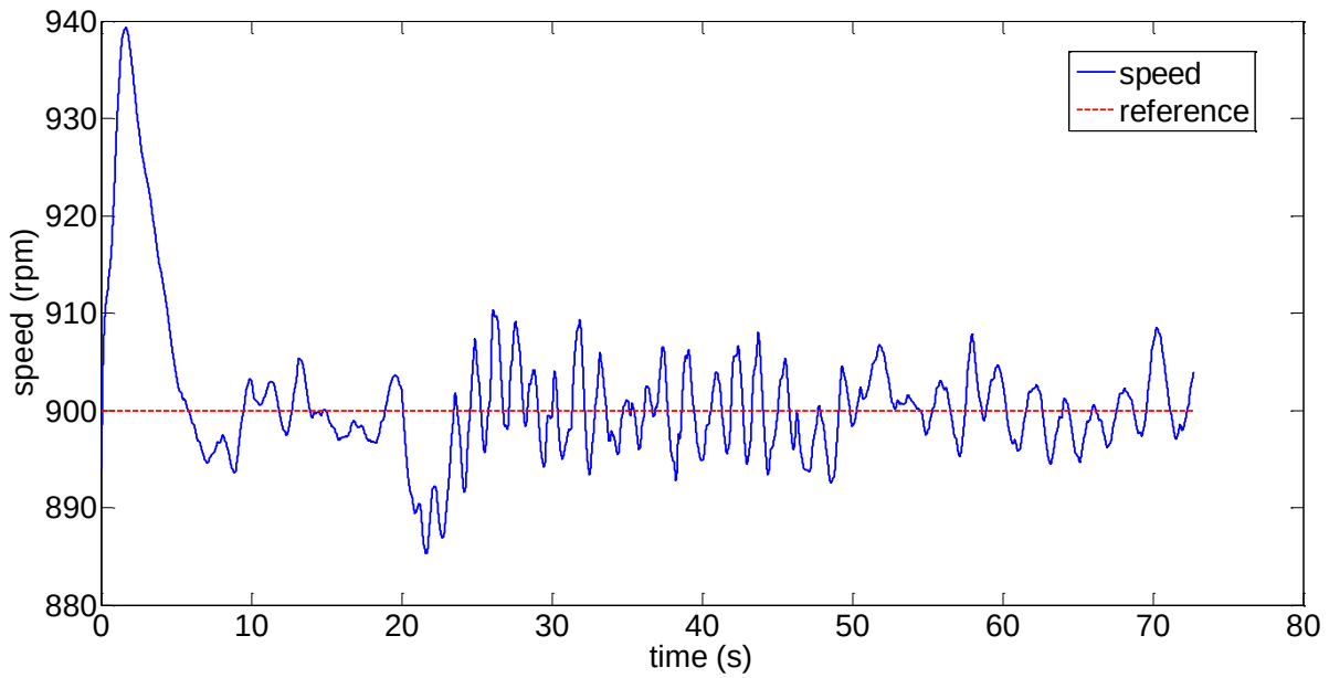
Fig. 84. Simulation result of idle speed control in presence of external disturbance
