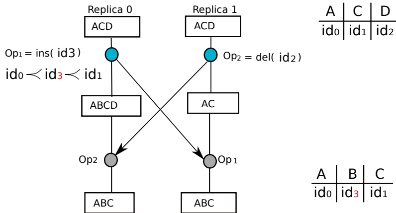
FIGURE 2.11 – Commutative Replicated Data Types
