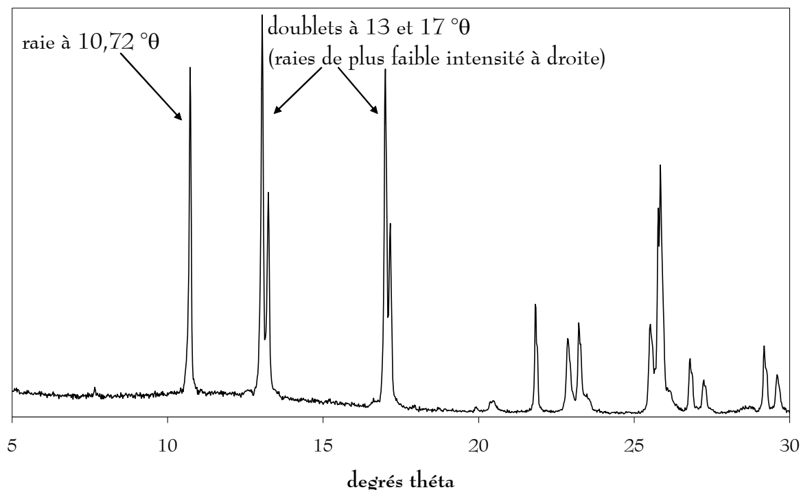
Figure 11 : Diffractogramme d' \text{U}_3\text{O}_8 pur.
