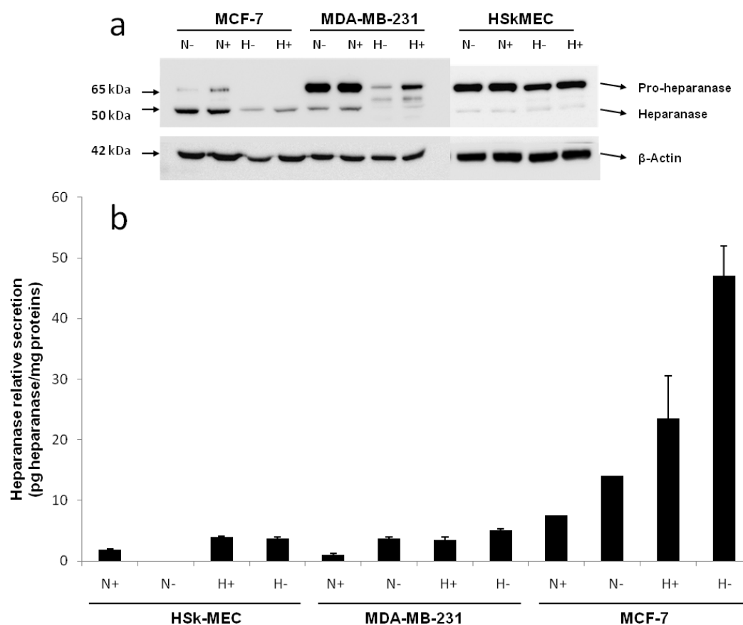
Figure 2. Determination of heparanase expression in both cell lysates and medium of HSkMEC, MDA-MB-231 and MCF-7 cells. (a). Western blot analysis of cell lysates (22.5 µg of total proteins) obtained from cells cultured under hypoxic or normoxic conditions for 48h in 2% FBS or FBS-free medium. Bands were reported relative to the level of β-Actin. (b). ELISA quantification of heparanase in cell supernatant obtained from cells cultured under hypoxic or normoxic conditions for 48h in 2% FBS or FBS-free medium. H indicates Hypoxia; N indicates Normoxia; (+) indicates that 2% FBS was present in the medium; (-) indicates that the medium was FBS-free. Results are expressed as a relative heparanase
