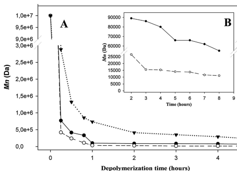
Fig. 2. (A) Effect of the H 2 O 2 ultrasonically-assisted radical depolymerization method on λ-carrageenan number-average molecular weight (Mn) with three different concentrations of H 2 O 2 . (B) Enlarged view showing the most effective depolymerization that was observed after 2–8 h. λ-carrageenan depolymerization in the presence of 0.75 mg/mL of H 2 O 2 (▲), 1.5 mg/mL of H 2 O 2 (●), and 7.5 mg/mL of H 2 O 2 (○).
