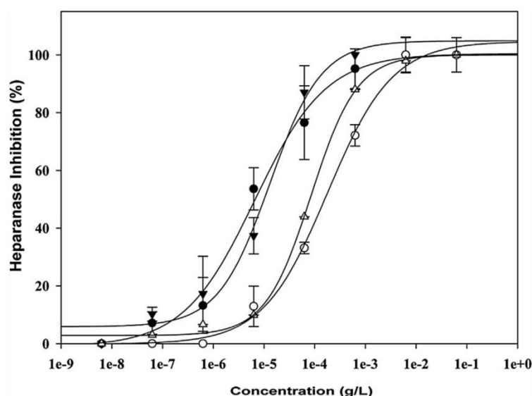
Fig. 4. Dose-response curves obtained for UF-heparin ( \blacktriangledown ), (Lovenox ® ) ( \triangle ), RD-GS-heparin ( \circ ) and RD-GS- \lambda -carrageenan ( \bullet ) using 100 ng/mL of heparanase, to determine the respective IC 50 .
