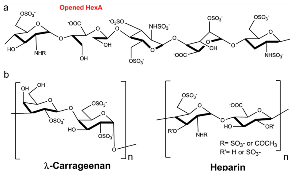
Fig. 1. Polysaccharide structure and impact of glycol splitting procedure. a) Glycol-split heparin pentasaccharide with opened hexuronic acid ring disrupt anticoagulant properties, b) Structure of \lambda -carrageenan and heparin. Both of these polysaccharide chains are sulfated and polyanionic, showing highly similar structures when the heparin disaccharides are sulfated at the R and R' positions.
