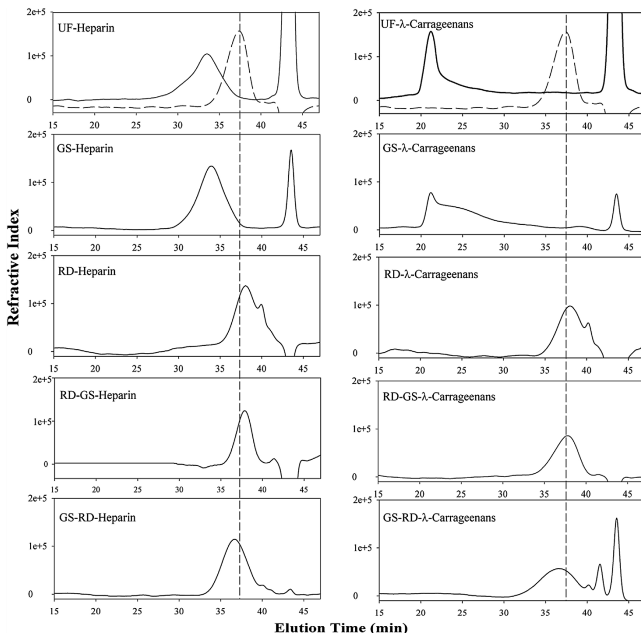
Fig. 3. SEC analysis of heparins and \lambda -carrageenans before and after different fractionation processes: glycol splitting (GS), ultrasonically-assisted radical depolymerization (RD) and the combination of both. RD-GS meaning depolymerization then glycol splitting, GS-RD meaning glycol splitting then depolymerization. Dashed chromatogram superimposed on UFH and UF- \lambda -carrageenans corresponds to the chromatogram of Lovenox ® and the dashed vertical line indicates its elution time. SEC separation was performed on a TSK-GEL G5000PW column in series with a TSK-GEL G4000PW at a flow rate of 0.5 mL/min using 0.1 M sodium nitrate (NaNO 3 ) as the eluent.
