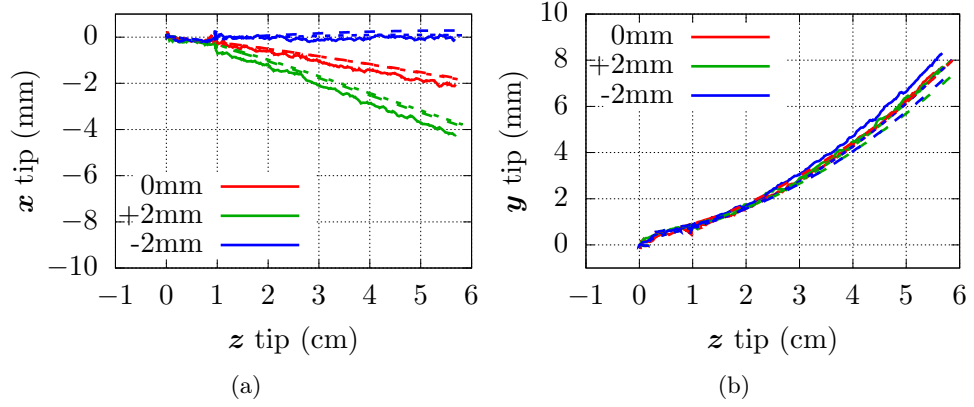
Figure 2.9: Tip position obtained when a translation is applied along the \mathbf{x} axis of the base frame between two insertion steps along the \mathbf{z} axis. Measures are shown with solid lines, virtual springs model with long-dashed lines and two-body model with short-dashed lines.
