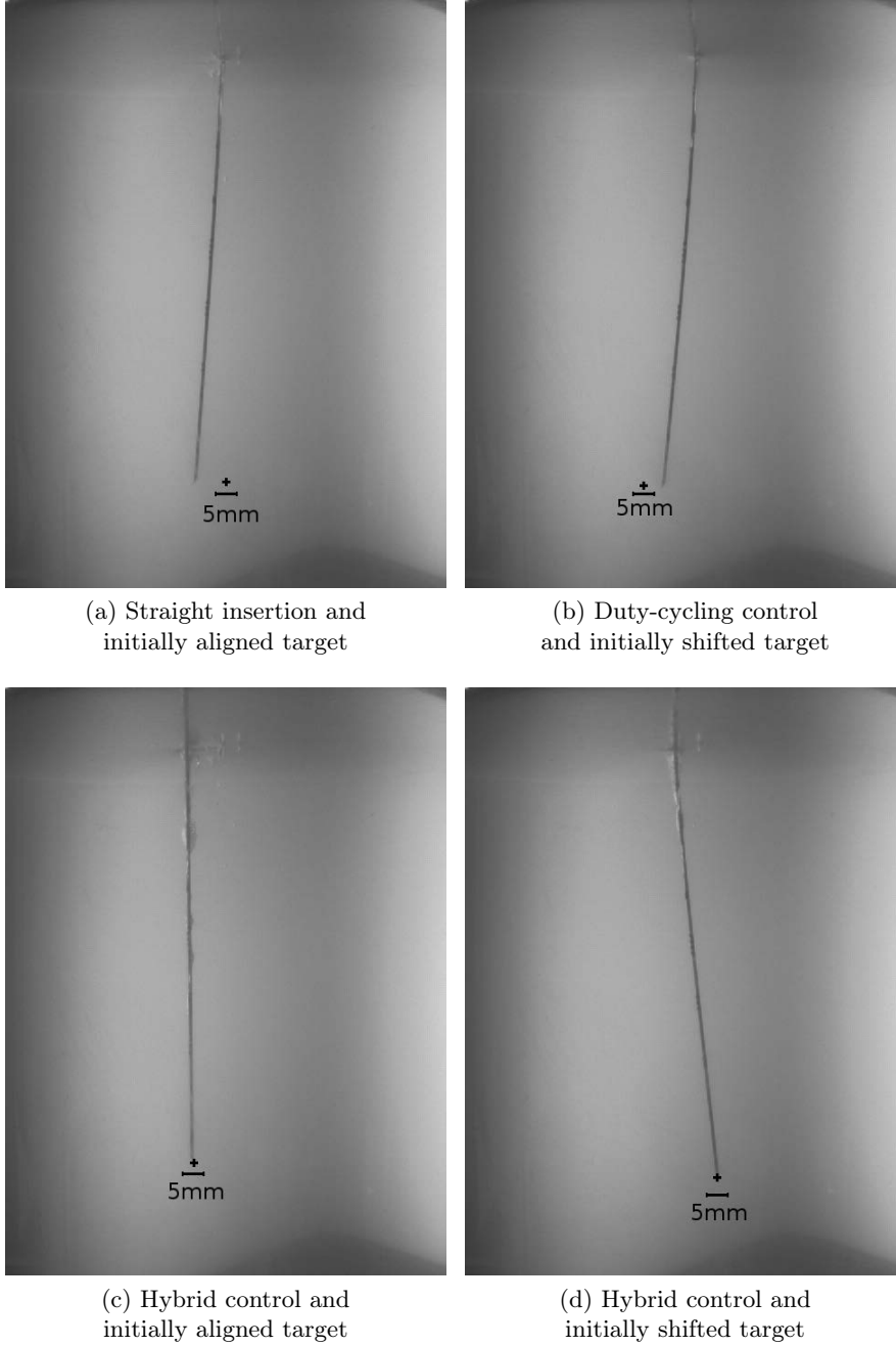
Figure 4.7: Final views of the front camera at the end of 4 insertions with different controls. The crosses represent the target. (a) Straight insertion with an initially aligned target: the target is missed due to tip deflection. (b) Duty-cycling control with a target shifted 1 cm away from the initial needle axis: duty-cycling control is saturated and the target is missed due to insufficient tip deflection. The target can be reached in both cases using the hybrid control framework ((c) aligned target and (d) shifted target).
