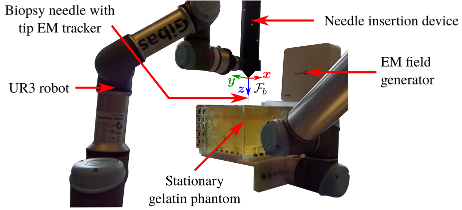
Figure 2.8: Picture of the setup used to acquire the trajectory of the tip of a real needle inserted in a gelatin phantom. The frame attached to the needle base is denoted by \{F_b\} .
