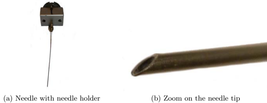
Figure 1.8: Picture of the needle used for the experiments in France.
