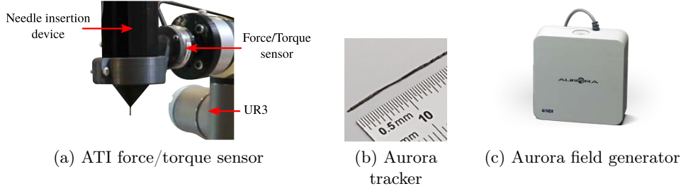
Figure 1.9: Picture of the electromagnetic tracking system and force sensor used for the experiments.
