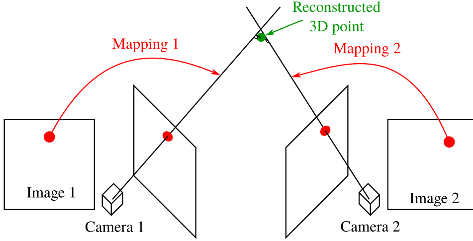
Figure 3.8: Illustration of the reconstruction of a 3D point from its position observed in two images acquired by two different cameras. The red dots represent the 2D position of the object seen in both images and the green dot is the estimation of the 3D position of the object.
