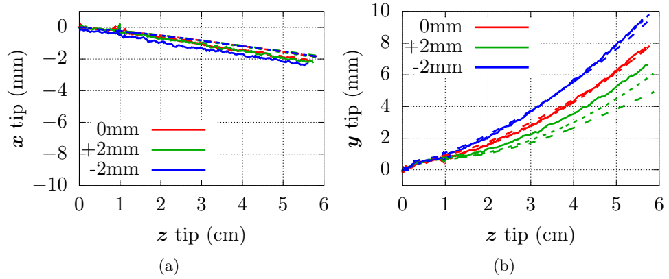
Figure 2.10: Tip position obtained when a translation is applied along the \mathbf{y} axis of the base frame between two insertion steps along the \mathbf{z} axis. Measures are shown with solid lines, virtual springs model with long-dashed lines and two-body model with short-dashed lines.
