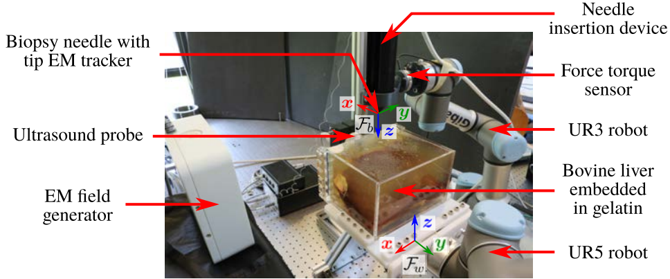
Figure 5.7: Picture of the setup used to perform needle insertions toward a target embedded in an ex-vivo bovine liver while compensating for lateral motions of the phantom.
