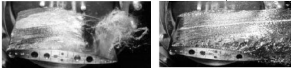
(a) Attached partial cavitation pocket on a profile (b) Supercavitation pocket on a profile
