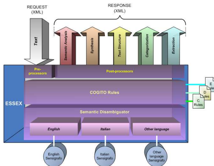
FIGURE 3.3 – architecture d'ESSEX
