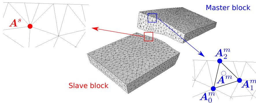
Figure 1.9: Node to triangle condition. \mathbf{A}^s is a node on the slave fault mirror. It is projected onto the master fault mirror. The image of \mathbf{A}^s onto the master triangle \mathbf{A}_0^m \mathbf{A}_1^m \mathbf{A}_2^m is \mathbf{A}^m which is defined by its barycentric coordinates. Data courtesy of Total.
