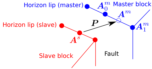
Figure 1.8: Node to edge condition. \mathbf{A}^s is a node on the slave fault cutoff line. It is projected onto the master fault cutoff line. The image of \mathbf{A}^s onto the master edge \mathbf{A}_0^m \mathbf{A}_1^m is \mathbf{A}^m (defined by its barycentric coordinates in the edge).
