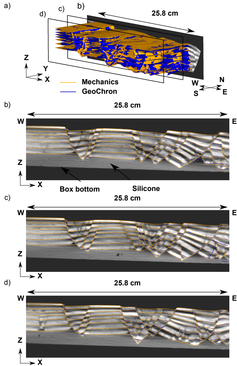
Figure 3.3: Visual comparison of the unrestrained state between the GeoChron-based input model (dark blue) and the mechanics-based input model (orange). In each sub-figure both models are displayed. a) Overlaid 3D models. The CT image and the two rectangles with black borders are the cross sections presented in b), c) and d) respectively on the north, the center and the south of the model. Both models are visually very similar along the model. CT data courtesy of IFPEN and C&C Reservoirs, 2016, DAKS TM - Digital Analogs Knowledge System.
