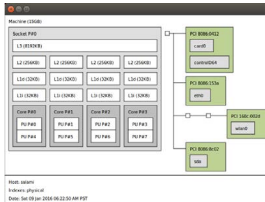
Figure 2.1: Multi-core architecture
