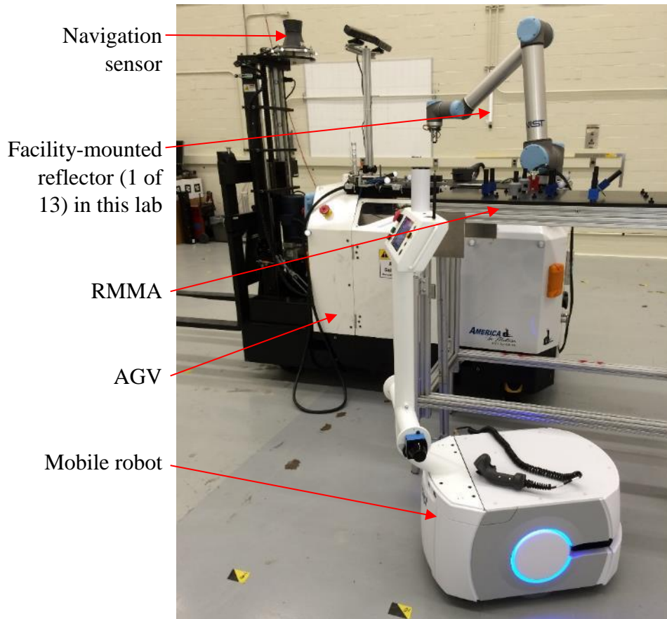
Figure 31. AGV with onboard manipulator behind an autonomous mobile robot (foreground) and the RMMA between the vehicles.
