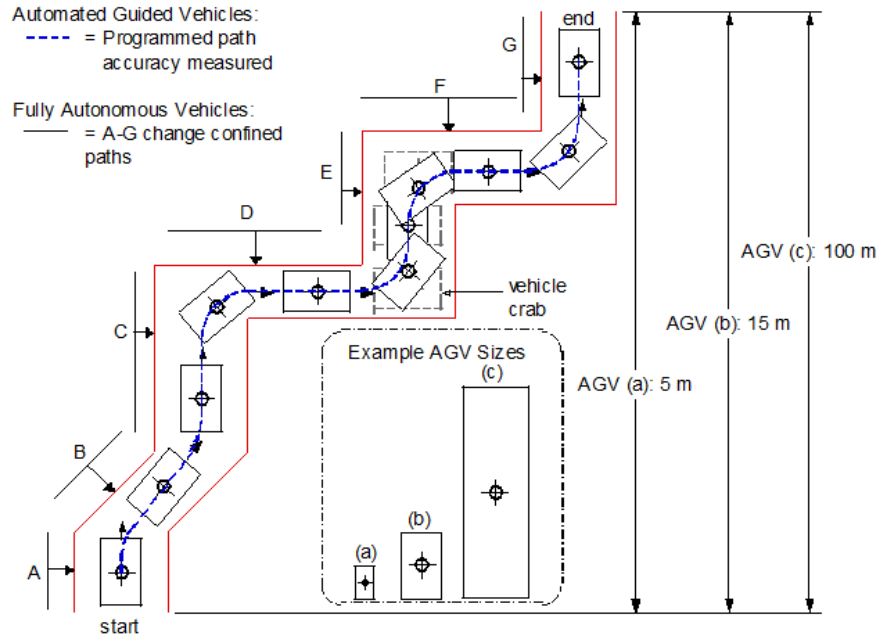
Figure 44. Example reconfigurable apparatus for navigation tests for various AGV sizes.
