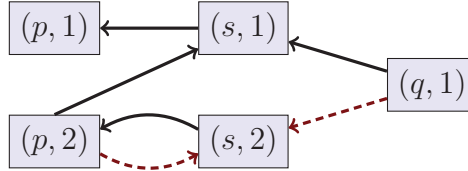
Figure 3.4: PPG(\mathcal{R}) from Example 3.12
