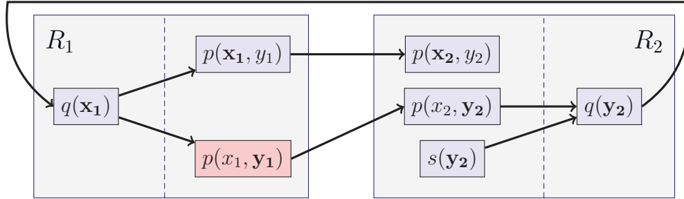
Figure 3.6: Full Position Graph of \{R_1, R_2\} from Example 3.17
