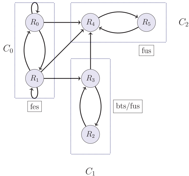
Figure 2.6: Graph of Rule Dependencies of \mathcal{R} from Example 2.18
