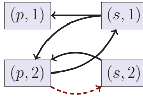
Figure 2.3: Predicate Position Graph of \mathcal{R} from Example 2.6
