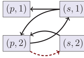
Figure 2.3: Predicate Position Graph of \mathcal{R} from Example 2.6
