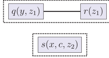
Figure 1.2: Piece Graph of rule R from Example 1.10
