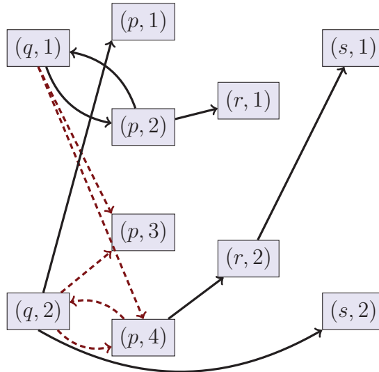
Figure 2.5: Predicate Position Graph of \mathcal{R} from Example 2.17
