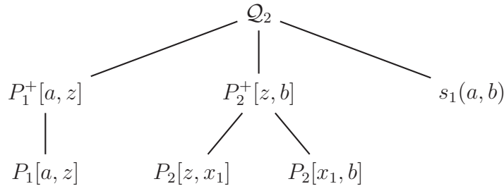
Figure 4.2: Instantiation T_1 from Example 4.3
