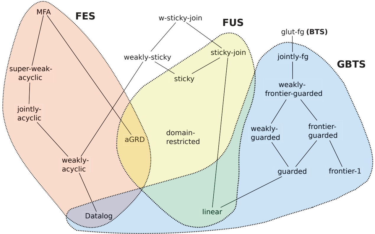
Figure 2.1: Relations between known decidable rule classes
