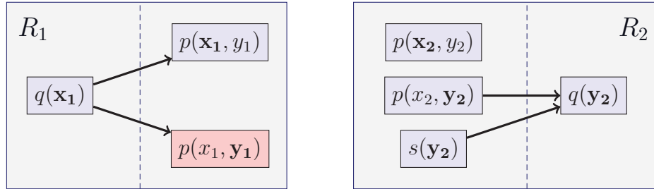
Figure 3.5: Basic Position Graph of \{R_1, R_2\} from Example 3.17
