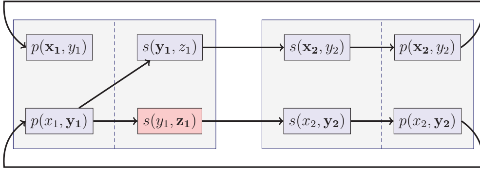
Figure 3.7: PG^F(\mathcal{R}) from Example 3.19
