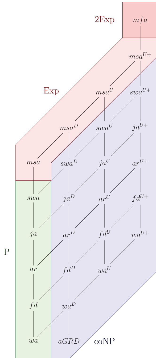
Figure 3.10: Relations between acyclicity properties with complexities of recognition
