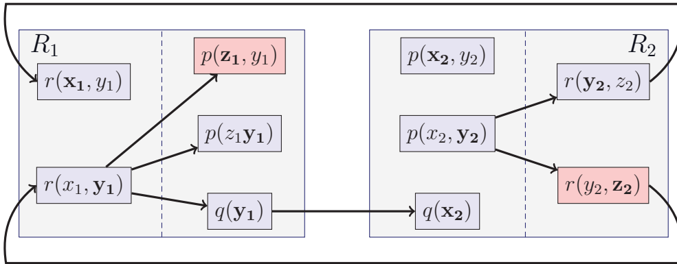
Figure 3.9: PG^U(\mathcal{R}) from Example 3.22
