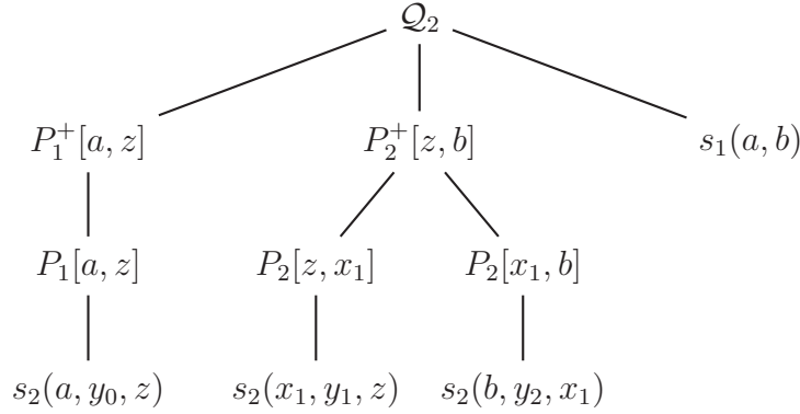
Figure 4.4: Instantiation of Q_3 from Example 4.9
