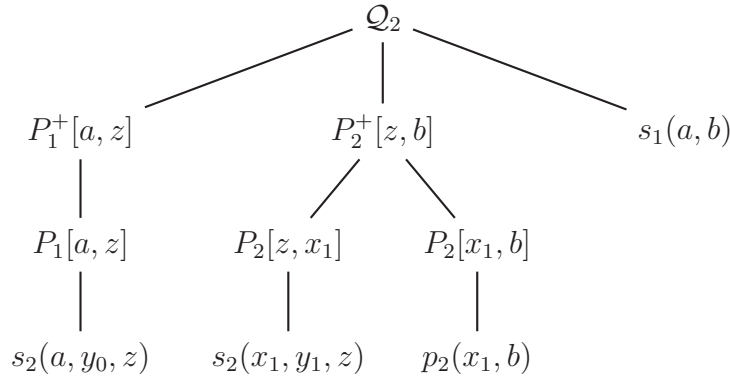
Figure 4.2: Instantiation T_1 from Example 4.3
