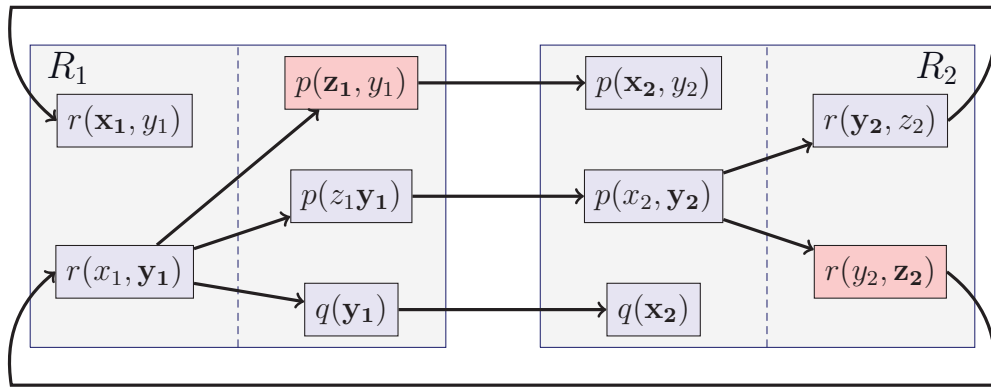
Figure 3.8: PG^D(\mathcal{R}) from Example 3.20
