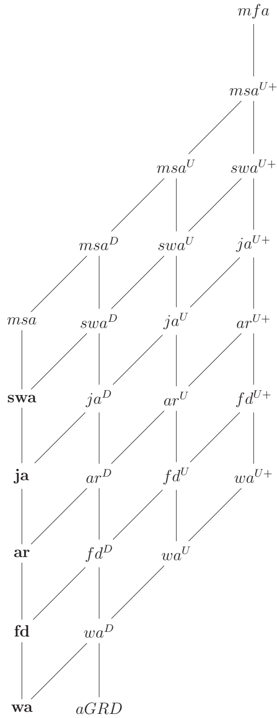
Figure 4.1: The landscape of C+trans classes for C \in FES . Decidable C+trans are in bold. All the other C+trans classes are undecidable even for atomic CQs.
