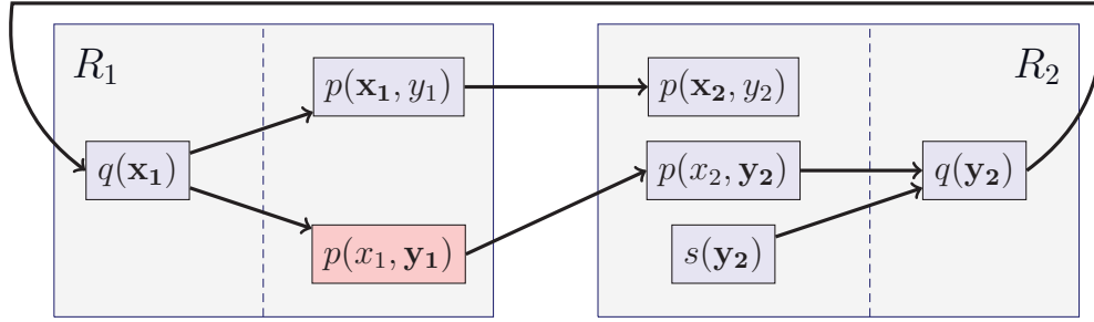
Figure 3.6: Full Position Graph of \{R_1, R_2\} from Example 3.17
