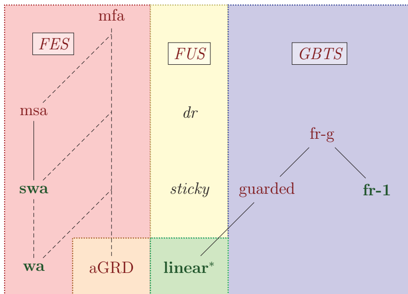
Figure 4.6: Decidability of Entailment over C+trans Knowledge Bases
