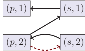
Figure 3.2: Predicate Position Graph of \{R_1, R_2\} from Example 3.10
