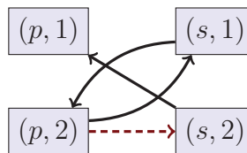
Figure 2.2: Predicate Position Graph of \{R_1, R_2\} from Example 2.5
