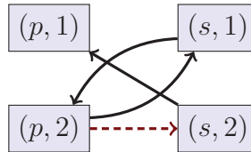
Figure 3.3: Predicate Position Graph of \{R_1, R'_2\} from Example 3.11
