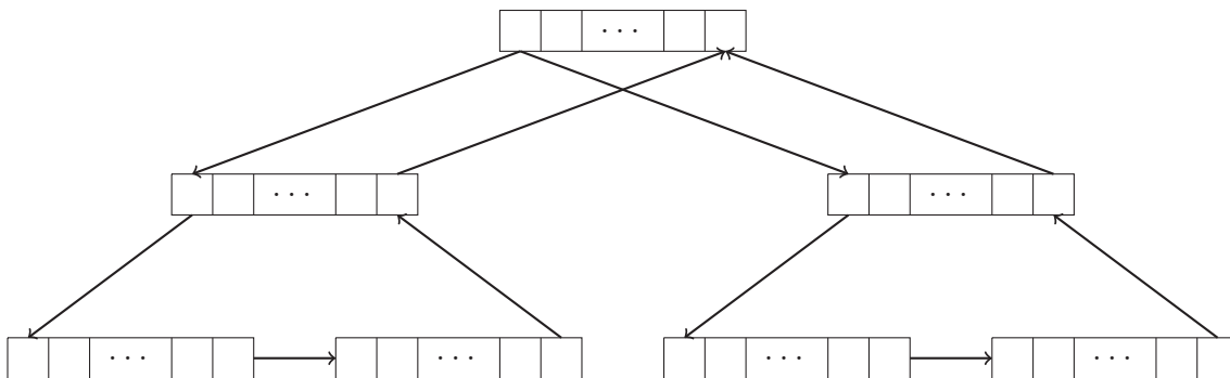
Figure 4.5: Reduction from ATM simulation to atomic CQ entailment over linear+trans knowledge bases. Edges stand for p -atoms and arrays stand for configuration atoms, with the first and last elements corresponding to the begin and end terms.
