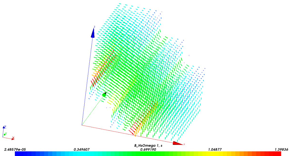
Figure 2.30 Magnetic Flux Density Distribution for Topology with Proposed Methodology (Linear Case)
