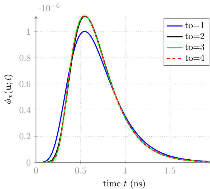
Figure 3.3.5: This figure shows results for different time order up to 4 for \mathbb{P}_3 solutions on an homogeneous testcase and using a mesh of size 2mm, time step 20ps, final time 2000ps. The results seem to converge from time order 3, but is acceptable from time order 2 as well as for the \mathbb{P}_2 case (fig. 3.3.4).
