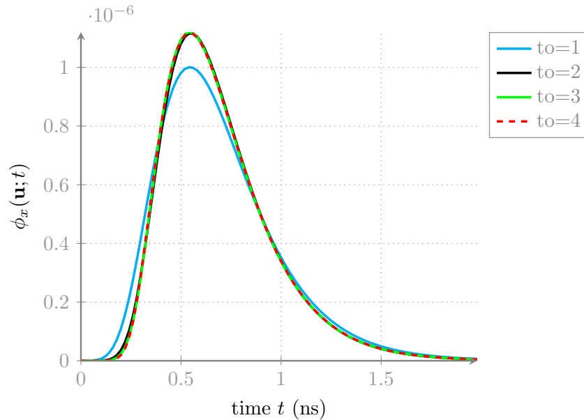
Figure 3.3.4: This figure shows computation results for different time order up to 4 for \mathbb{P}_2 solutions on an homogeneous object. The mesh size is 2mm, the time step 20ps and the final time 2000ps. We see that the solution seems to converge from time order 3, but with an acceptable result in time order 2. Note also we have a variation of intensity in that case, we obtain more precise solution at higher order.
