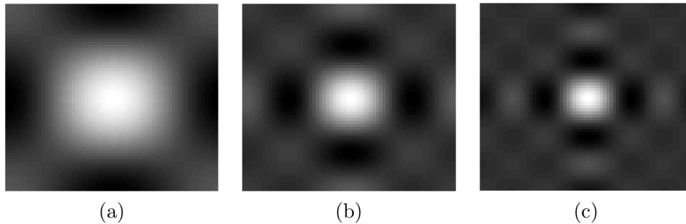
Figure 7.4 ~ SPECTRA OF THE UNIFORM BLUR OPERATORS ~ They are respectively applied on (a) Red, (b) Green and (c) Blue channels of the original color image, with a uniform boxcar point spread function of size n \times n (with pixel value: 1/n^2 ) with n = 3, 5 , and 7 .
