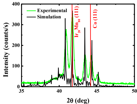
Figure 51. Large angle specular X-ray diffraction measurement (green) from a [\text{Co}(5\text{nm})/\text{Ir}_{0.2}\text{Mn}_{0.8}(5\text{nm})]_{15} multilayers deposited on LNO41 Y-cut. Simulated curve is presented in black.
