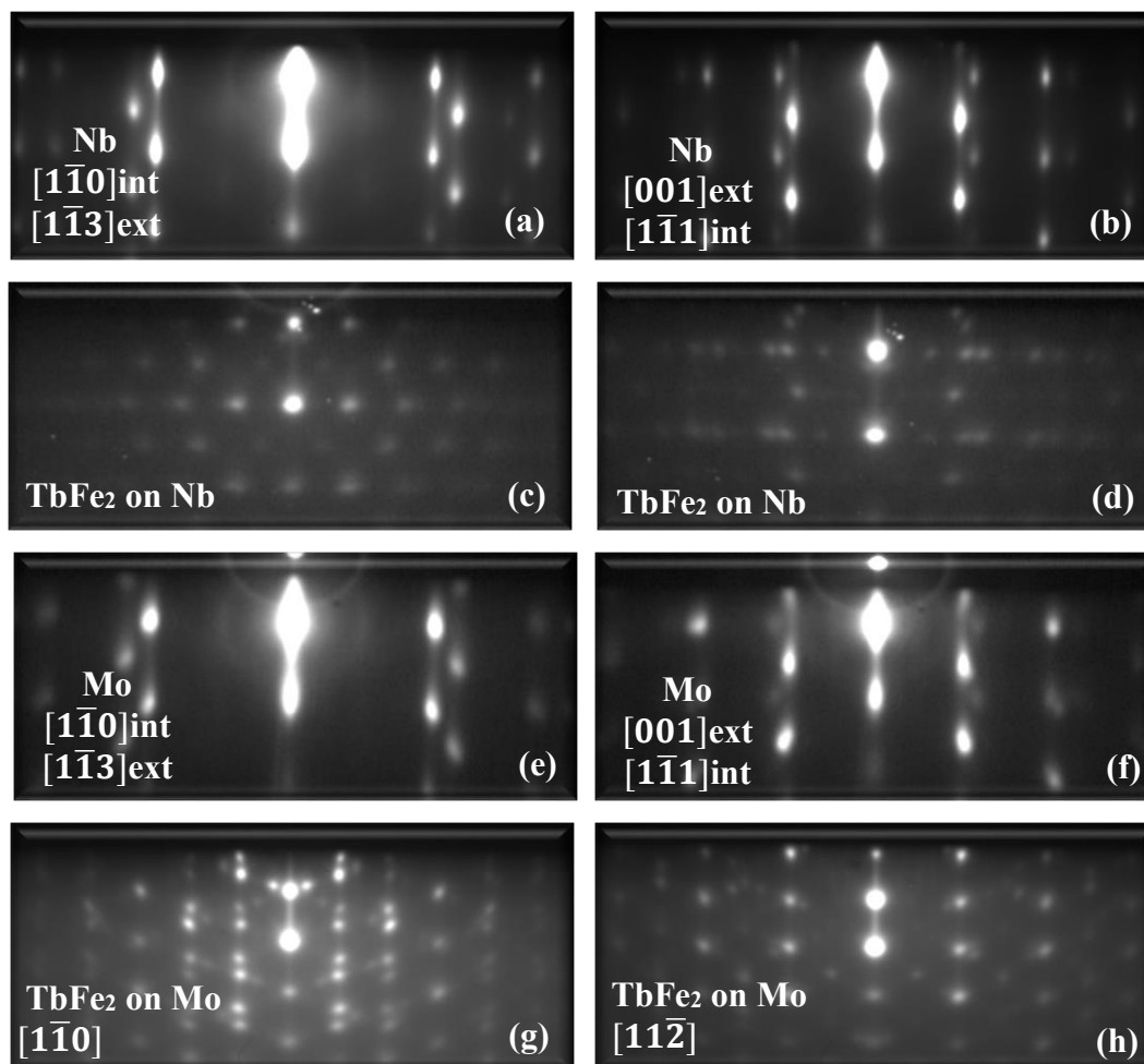
Figure 36. RHEED patterns collected along two azimuths rotated by 90° for 50 nm thick Nb deposited at 450°C on LNOZ/Ti (a and b), 50 nm thick TbFe 2 deposited on Ti/Nb at 650 °C (c and d), 50 nm thick of Mo deposited at 450 °C on LNOZ/Ti (e and f) and 50 nm thick TbFe 2 deposited on Ti/Mo at 650 °C (g and h).
