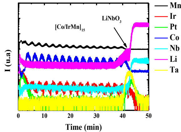
Figure 67. SIMS spectra measured during etching of a LNO41/Ta(5nm)/[Co(5nm)/Ir 0.2 Mn 0.8 (5nm)] 15 /Pt(5nm).
