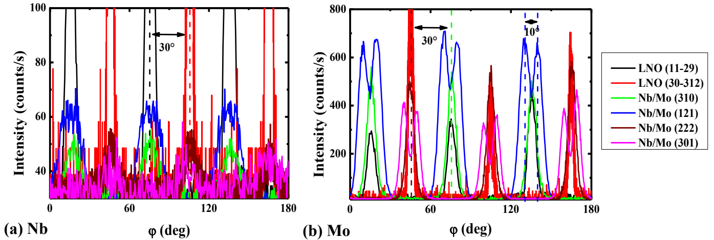
Figure 25. \phi scans for asymmetrical reflections measured for Nb (a) and Mo (b) deposited on LNO Z-cut. AR are also measured for LNO in both cases.
