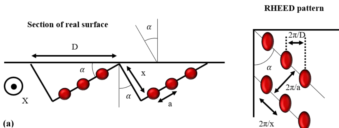
Figure 121. Sketch of a RHEED pattern (b) obtained from a stepped surface (a).
