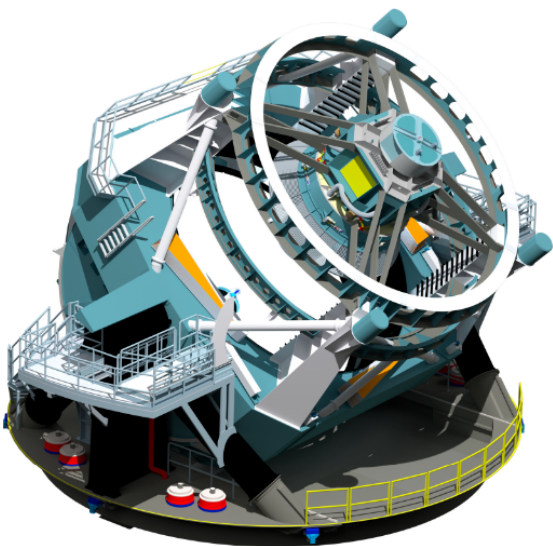
FIGURE 5.2: Left : Design of the telescope. The compactness of the mount is required to ensure a quick dampening of the vibrations after slewing. Right : Rendering of the camera clearly showing the two (of three) field corrector lenses and the red filter in front of the 3.2 \times 10^9 pixels of the focal plane. Five of the six filters will be loaded on the carousel (only the blue filter is shown in the image), ready to be automatically inserted in front of the focal plane. Credits https://www.lsst.org/ .
