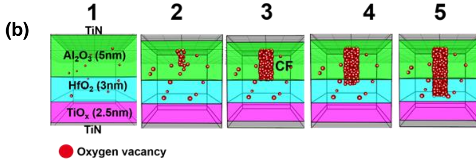
Figure 4. 4 : (a) Simulated I/V characteristic of the Set process for the S3 sample. (b) Corresponding evolution of defect creation in the HfO_2 and Al_2O_3 layers. (c) CF evolution during the Set process.
