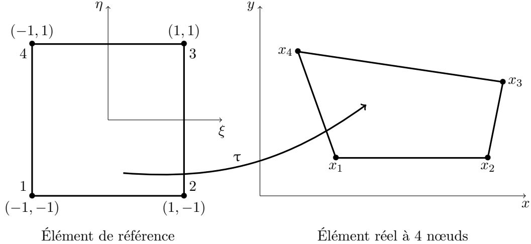
FIGURE 2.3 – Transformation \tau
