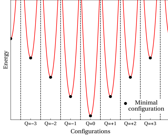
Figure 4.2: Energy profile of \mathcal{E} = \int d^2\mathbf{r} (\nabla \mathbf{m})^2 for different configurations \mathbf{m}(\mathbf{r}) with boundary condition \mathbf{m}(|\mathbf{r}| \rightarrow \infty) \rightarrow \mathbf{m}_\infty . Topological sectors in configuration space are labeled by an integer Q . In each topological sector, the energy-minimizing configuration is marked by a black dot.
