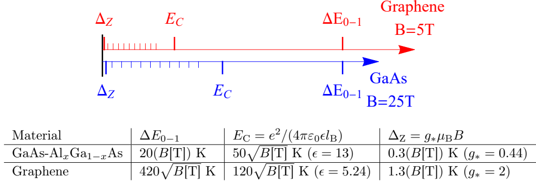
Figure 1.3: Energy scales. (blue) GaAs-Al x Ga 1-x As hetero-structure and quantum well, (red) graphene. The energy separation \Delta E_{0-1} between N = 0 and N = 1 LL is \Delta E_{0-1} = \hbar e B / m_* for GaAs-Al x Ga 1-x As and \Delta E_{0-1} = \sqrt{2} \hbar v_F / l_B for graphene. Notice that the ratio \Delta E_{0-1} / E_C \sim \hbar v_F / (e^2 / \epsilon) for graphene does not depend on the magnetic length nor any other length scales.
