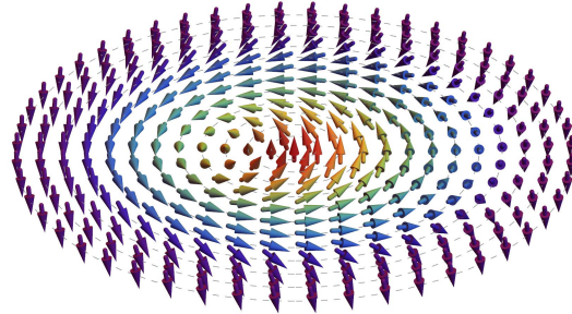
Figure 1: Skyrmion.
