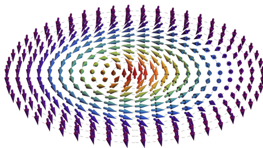
Figure 1.1: Skyrmion.
