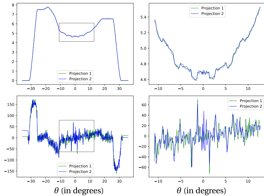
Figure 56: Same plots as Figure 55 with noisy projections.
