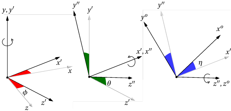
Figure 11: The zxy Tait-Bryan angles convention. First, a rotation of \phi about the y world axis is applied ( left ). Then, a rotation of \theta about the rotated x axis ( middle ). Finally, a rotation of \eta about the rotated z axis ( right ). The final coordinates are the OCS coordinates (x^o, y^o, z^o) .
