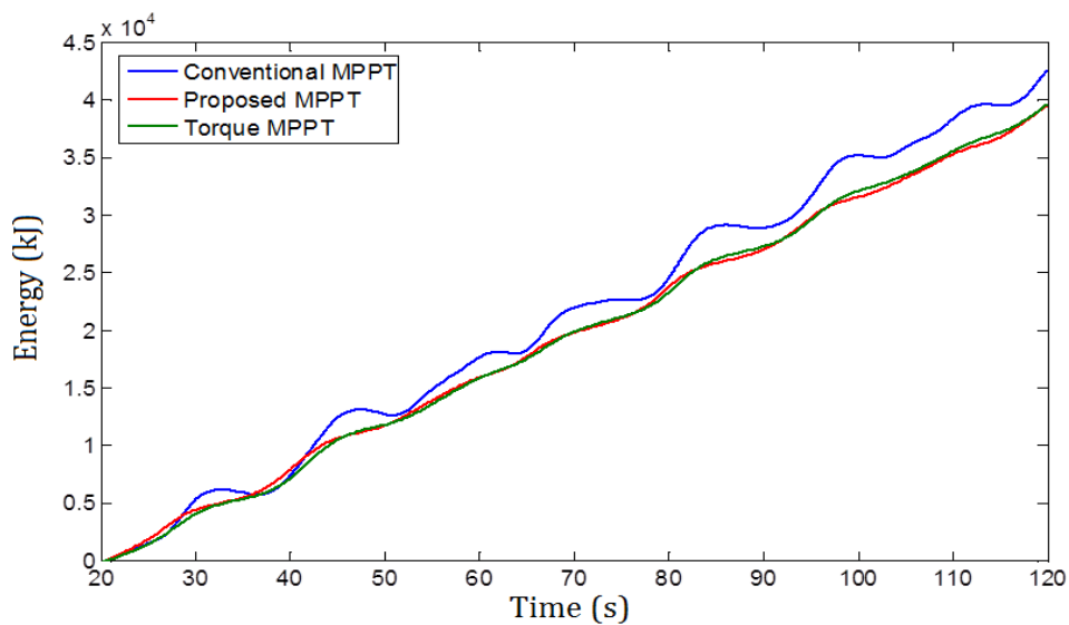
Fig. II.22. Comparison of generator-produced energy.
