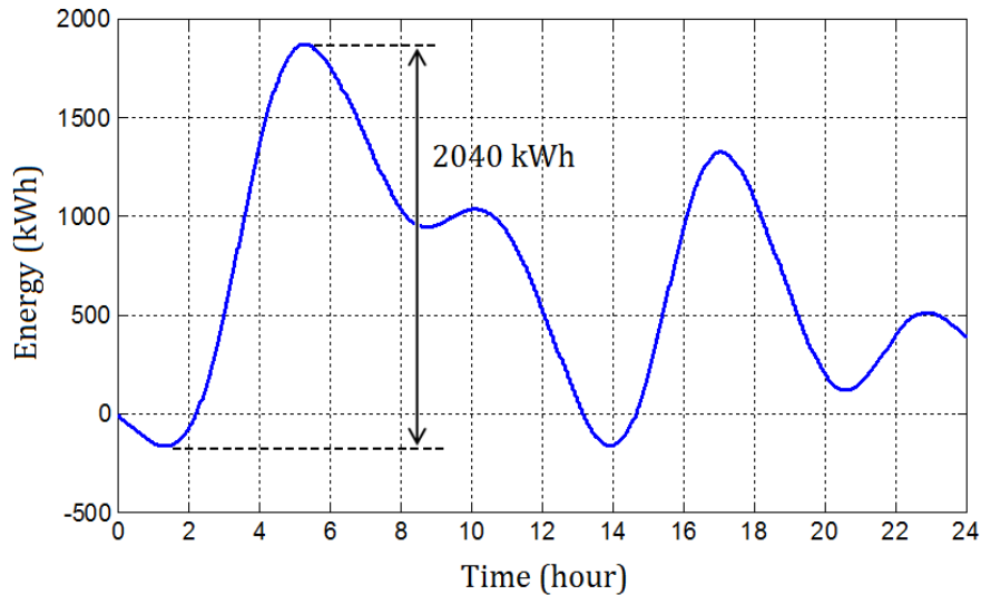
Fig. III. 4. The energy level change profile.
