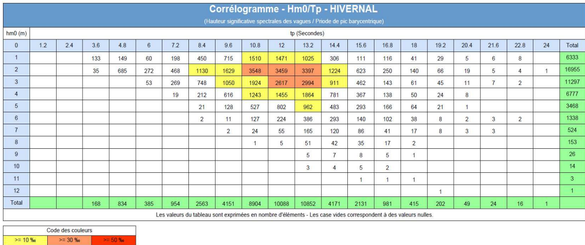
Fig. I.7. Correlation diagram of swell at Les Pierres Noires [22].
