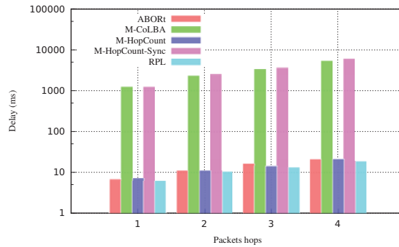
FIGURE 4.22: Packet end-to-end delay according to the number of hops from source node to the sink. Generation of 5 packets per second per node.
