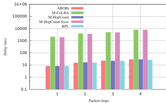
FIGURE 4.23: Packet end-to-end delay according to the number of hops from source node to the sink. Generation of 10 packets per second per node.
