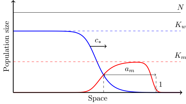
Figure 3.2 – Shape of the stationary front of the spreading epidemic. The epidemic moves at a constant speed c^* . The mutant genotype (in red) is prevalent at the edge of the front and reaches a maximal density of K_m . Behind the front, the wild type genotype (in blue) takes over and reaches a higher density K_w . The size of the area where the mutant is more abundant than the wild type is called the mutant's range, a_m .
