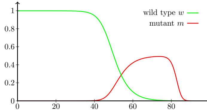
Figure 2.1 – Numerical simulation of (2.2) with r = 2 , K = 0.5 , \mu = 0.01 , with a heaviside initial condition for w and null initial condition for m . The numerical code is based on an implicit Euler scheme. For large times, the solution seems to converge to a travelling wave, that we represent here, propagating towards large x . In the initial phase of the epidemics, the mutant ( m , red line) population is dominant, but this mutant population is then quickly replaced by a population almost exclusively composed of wild types ( w , green line). Although the steady states on the back of the wave seems to be close to (w(x), m(x)) = (1, 0) , we actually know that (w^*, m^*) \in (0, 1) \times (0, K) .
