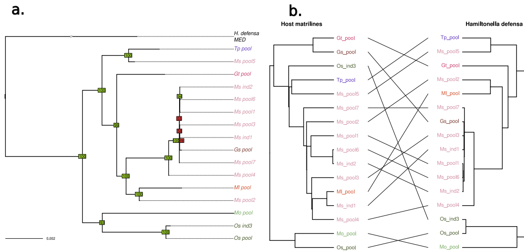
Figure 3 a) Phylogeny of Hamiltonella defensa . Phylogeny was inferred by Maximum likelihood based on a concatenate of 118 membrane protein-coding genes. Bootstrap values above or below 90 appear in green and red, respectively. b) Tanglegram of Hamiltonella defensa phylogeny with host matriline phylogeny
