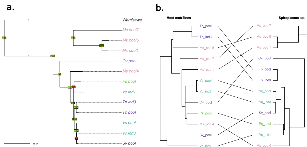
Figure 4 a) Phylogeny of Spiroplasma sp. . Phylogeny was inferred by Neighbor Joining based on a whole genome variant calling. Bootstrap values above or below 90 appear in green and red, respectively. b) Tanglegram of Spiroplasma sp. phylogeny with host matriline phylogeny
