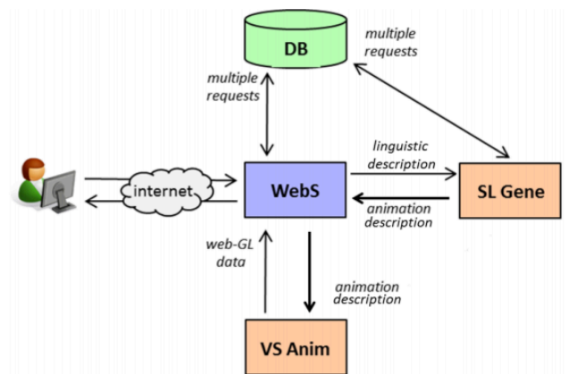
Figure 4.6: Architecture globale de KAZOO (Braffort et al, 2016)
