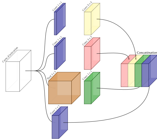
FIGURE 2.13 – Module Inception [163].
