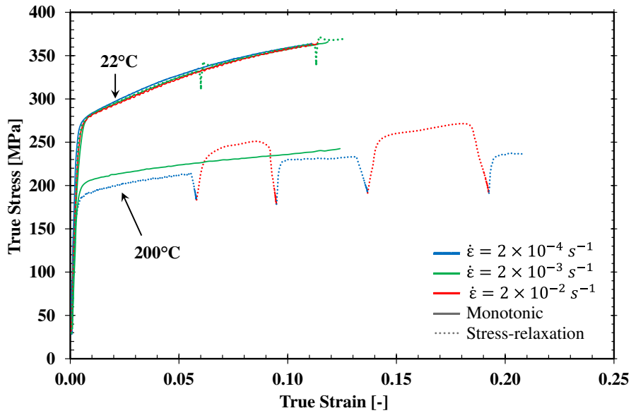
Figure 6 – Influence of the strain-rate on the true stress – true strain curves obtained from uniaxial tensile tests performed at 22 and 200 °C, for the EN AW 6061-T6 in specimens oriented along the RD.
