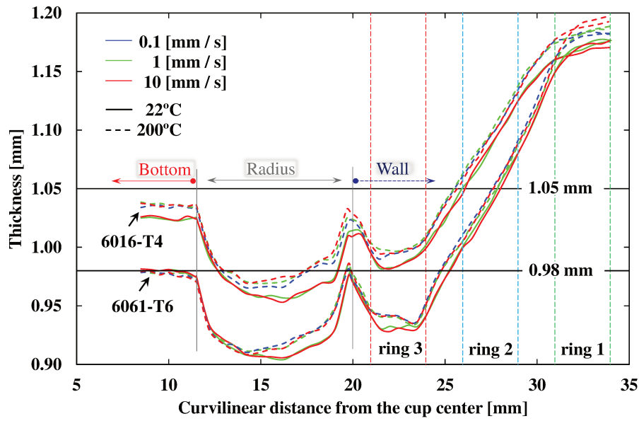
a) Cup Thickness
