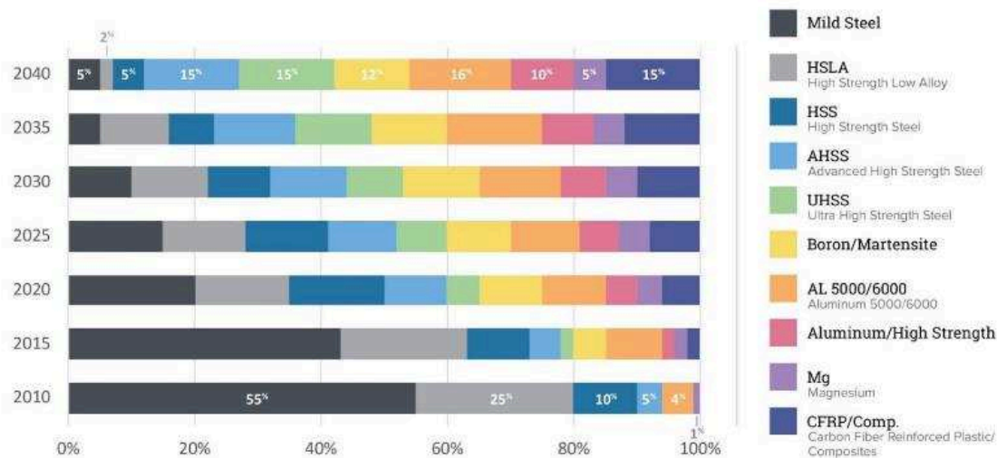
Figure 1.3 –Material distribution in the U.S. fleet (Body-in-white plus closures) (Smith et al., 2016).
