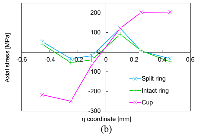
Fig. 10 Axial stress distributions along the middle section of the Top ring at the end of the forming and unloading stage, in the intact ring and in the split-ring: (a) Lower gap; (b) Higher gap
