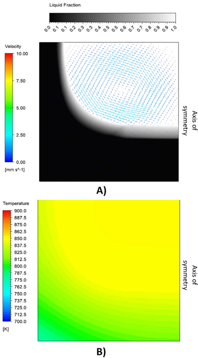
Figure 126 Numerical results at 60 seconds with almost 50% of material solidified. A) Liquid fraction field with the flow field shown by vectors. The local maximum flow velocity is 2 mm/s. B) Temperature fields
