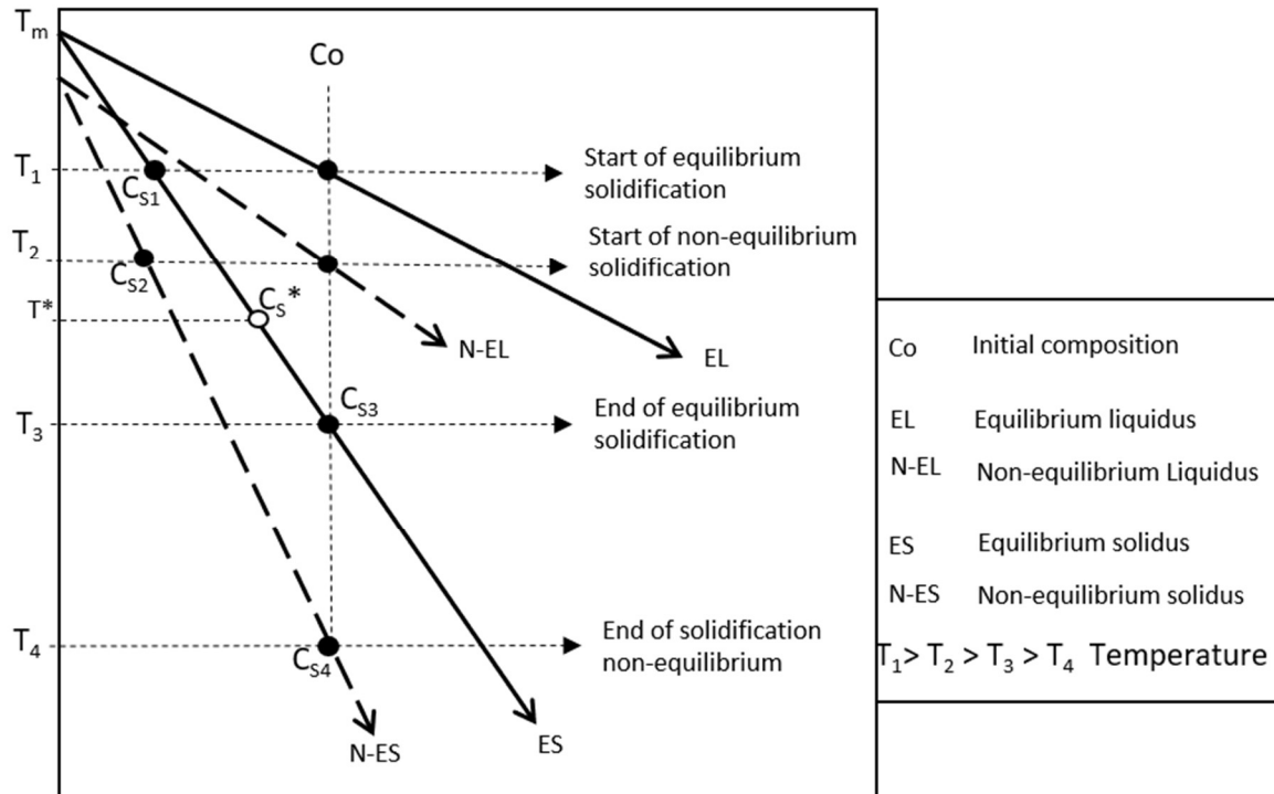
Figure 18 Comparison of equilibrium and non-equilibrium phase diagram. T_1 and T_3 are the temperature at which under equilibrium solidification begins and ends respectively. T_2 and T_4 are the start and end of solidification under non-equilibrium solidification. The difference between T_1 and T_2 is undercooling due to the rapid solidification. T_m is the melting temperature of pure element A.
