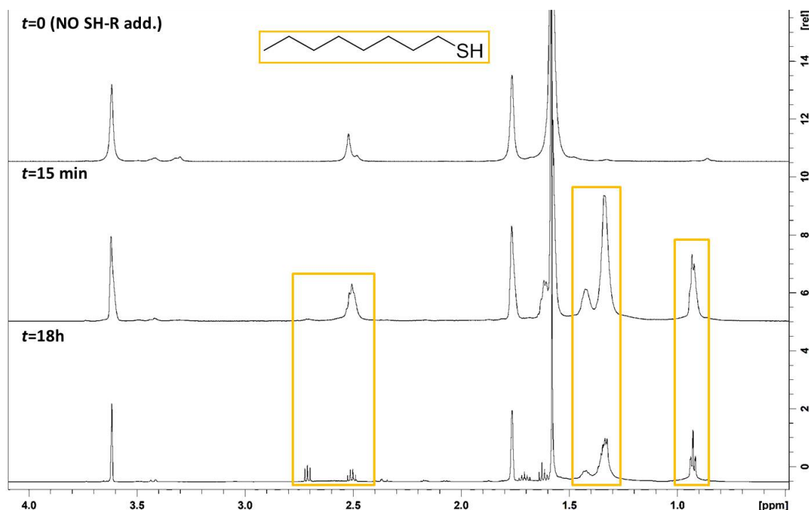
Figure 9. ^1\text{H} -NMR spectra (aliphatic region) in d^8 -THF of the exchange experiment based on the addition of 1-octanethiol onto preformed Ru-0.2PP NPs at t=0 (before addition of thiol), t=15 min and t=18 h.
