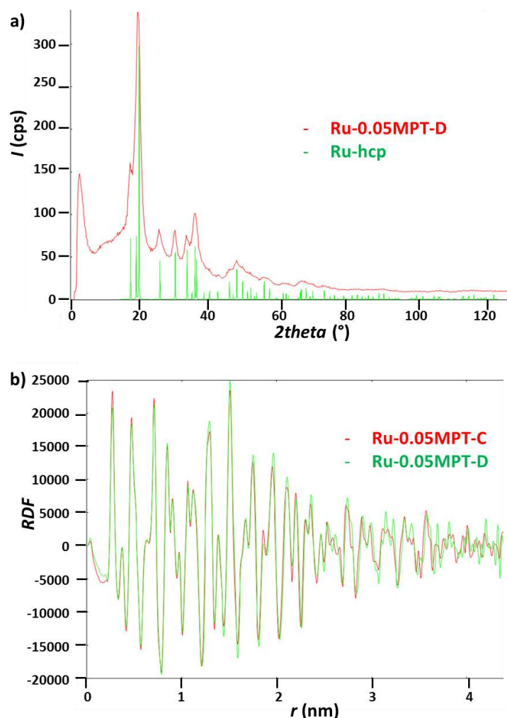
Figure 21. a) WAXS and b) RDF analysis of Ru-0.05MPT NPs after exposure of a THF-suspension to 3 bar O_2 at 50°C during 3 days. Comparison with Ru-hcp (a) and Ru-0.05MPT-C (b).
