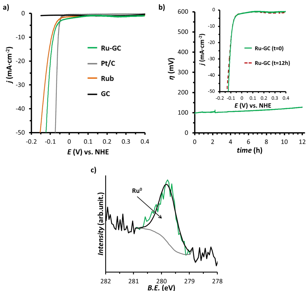
Figure 3. a) LSV curves of Ru-GC (green), Rub (orange), Pt/C (grey) and bare GC d electrode (black) in 0.5 M \text{H}_2\text{SO}_4 solution at 10 \text{ mV}\cdot\text{s}^{-1} ; b) current-controlled bulk electrolysis experiment of Ru-GC at j = -10 \text{ mA}\cdot\text{cm}^{-2} in 0.5 M \text{H}_2\text{SO}_4 , without ohmic drop compensation. Inset, LSV curves of the initial Ru-GC (green) and after 12h bulk electrolysis experiment at j = -10 \text{ mA}\cdot\text{cm}^{-2} (dashed red) in 0.5 M \text{H}_2\text{SO}_4 solution at 10 \text{ mV}\cdot\text{s}^{-1} ; c) XPS spectra of Ru-GC (green) after 15 min bulk electrolysis at j = -10 \text{ mA}\cdot\text{cm}^{-2} in 0.5 M \text{H}_2\text{SO}_4 . Background (grey), metallic-Ru component (dashed black), envelop (bold).
