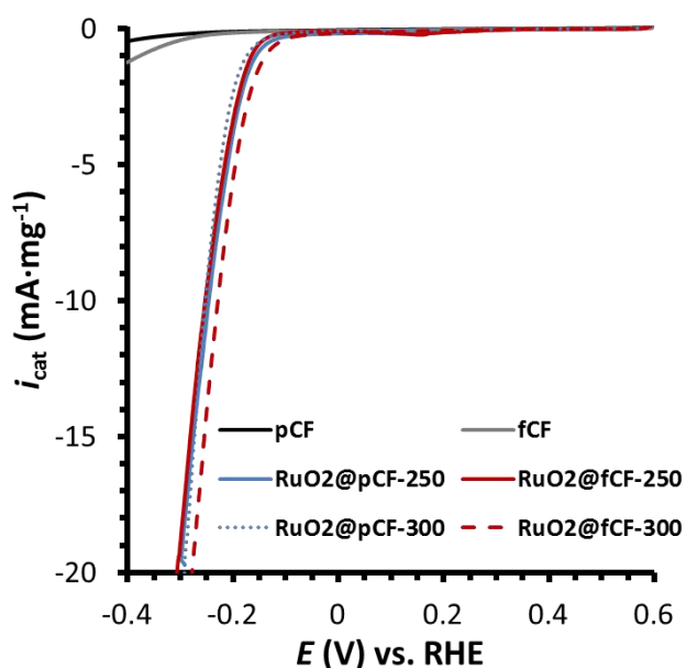
Figure 13. Polarization curves of \text{RuO}_2(250)@\text{pCF} (blue), \text{RuO}_2(300)@\text{pCF} (dashed-blue), \text{RuO}_2(250)@\text{fCF} (red), \text{RuO}_2(300)@\text{fCF} (red), bare pCF (black) and fCF (grey).
