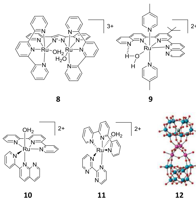
Figure 12. Structure of Llobet's dinuclear [\text{Ru}^{\text{II}}_2(\text{bpp})(\text{trpy})_2(\text{H}_2\text{O})_2]^{3+} ( 8 ), Thummel's [\text{Ru}^{\text{II}}(\text{tnp})(\text{Mepypy})_2(\text{H}_2\text{O})]^{2+} ( 9 ) and [\text{Ru}^{\text{II}}(\text{trpy})(\text{pynap})(\text{H}_2\text{O})]^{2+} ( 10 ), Meyer's [\text{Ru}(\text{trpy})(\text{bpm})(\text{OH}_2)]^{2+} ( 11 ), and Bonchio's \text{Ru}_4\text{-POM} ( 12 ).
