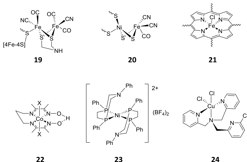
Figure 16. Earth-abundant metal-based complexes as HECs: [Fe-Fe]-hydrogenase ( 19 ), 107 [Ni-Fe]-hydrogenase ( 20 ), 107 Fe-based porphyrin ( 21 ), 108 [Co III (DO)(DOH)pnX 2 ] ( 22 ), 113 [Ni(P 2 Ph N Ph ) 2 ](BF 4 ) 2 ( 23 ) 114 and [Cu(Cl-TMA)Cl 2 ] ( 24 ). 115a
