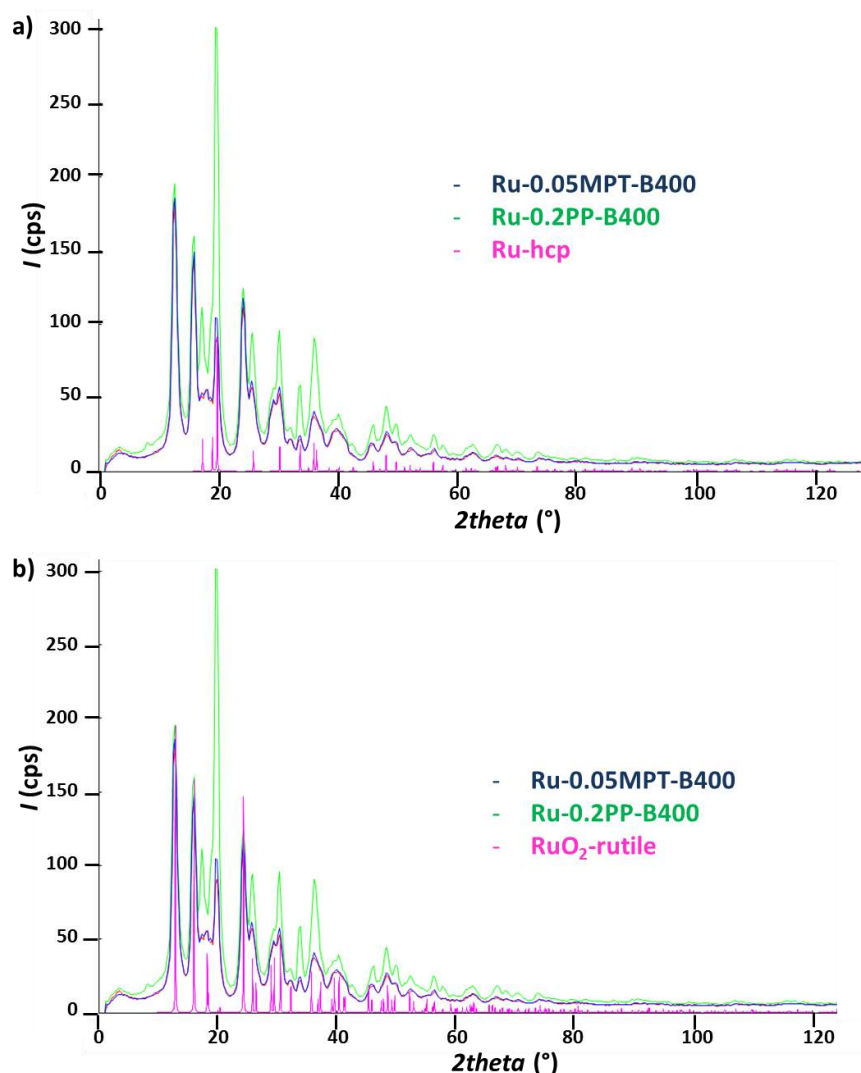
Figure 17. WAXS analysis of Ru-0.2PP and Ru-0.05MPT NPs after air exposure at (400 °C). Comparison with a) Ru-hcp and b) \text{RuO}_2 reference phases.
