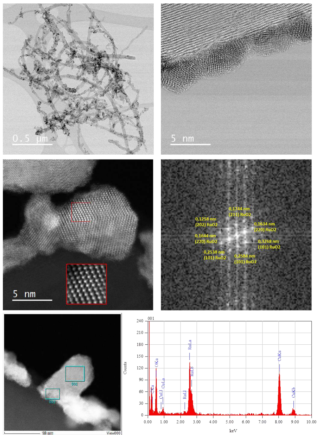
Figure 6. HRTEM images, FFT patterns and EDX analysis of RuO 2 @CNT.
