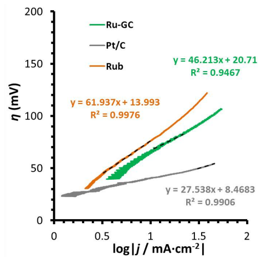
Figure 4. Tafel Plot of Ru-GC (green), Rub (orange) and Pt/C (grey) in 0.5 M H 2 SO 4 .
