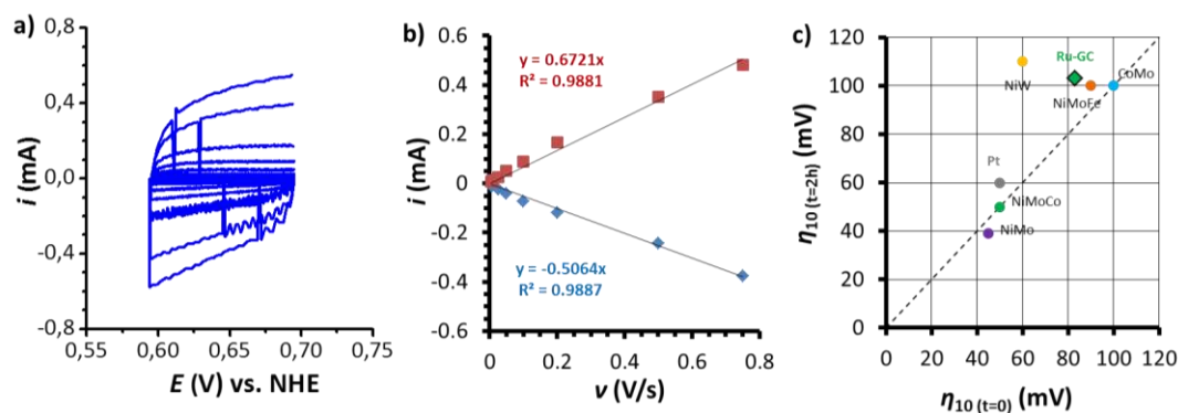
Figure 4. a) Representative multi CV experiment at different scan rates for C_{DL} determination in 0.5 M H 2 SO 4 ; b) plot of current values at 0.65 V (vs. NHE) for the different scan rates, for C_{DL} determination; c) graphical representation of electrocatalysts benchmarking comparison.
