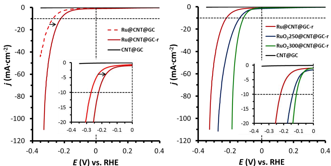
Figure 14. Left, polarization curves of Ru@CNT@GC (dashed red) and Ru@CNT@GC-r (dark red) before and after reductive process at j = -10 \text{ mA}\cdot\text{cm}^{-2} in 1\text{M H}_2\text{SO}_4 , respectively; right, Ru@CNT@GC-r (dark red), \text{RuO}_2250\text{@CNT@GC-r} (blue) and \text{RuO}_2300\text{@CNT@GC-r} (green) after reductive process at j = -10 \text{ mA}\cdot\text{cm}^{-2} in 1\text{M H}_2\text{SO}_4 .
