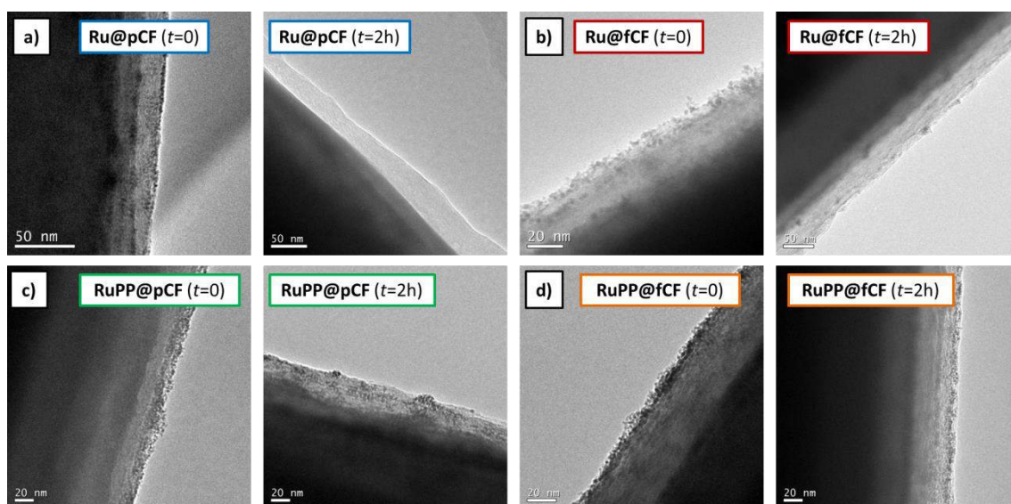
Figure 7. Representative TEM images of a) Ru@pCF , b) Ru@fCF , c) RuPP@pCF and d) RuPP@fCF at t=0 and t=2h after bulk electrolysis in 1 M H_2SO_4 at \eta = 250 and 350 mV for Ru@xCF and RuPP@xCF, respectively.
