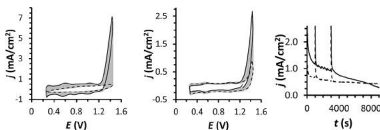
Figure 4. 1000 repetitive CV scans at pH 7 at a scan rate of 100 \text{ mV s}^{-1} from 0.25 to 1.45 V for 2b 2+ : 3b (left, \Gamma_{2b^{2+}} = 2.07 \text{ nmol cm}^{-2} and \Gamma_{3b} = 0.36 \text{ nmol cm}^{-2} ) and 2c 2+ : 3c (middle: \Gamma_{2c^{2+}} = 0.13 \text{ nmol cm}^{-2} and \Gamma_{3c} = 0.03 \text{ nmol cm}^{-2} ) at \text{GC}_d . Black solid line is the first cycle, black dashed line is the 1000th cycle. In gray are 2nd–999th cycles. Right: bulk electrolysis of 2b 2+ : 3b (solid black, \Gamma_{2b^{2+}} = 2.10 \text{ nmol cm}^{-2} and \Gamma_{3b} = 0.40 \text{ nmol cm}^{-2} ) and 2c 2+ : 3c (dashed black, \Gamma_{2c^{2+}} = 0.11 \text{ nmol cm}^{-2} and \Gamma_{3c} = 0.03 \text{ nmol cm}^{-2} ) in a phosphate buffered solution at pH 7 at E_{\text{app}} = 1.45 \text{ V} under stirring using \text{GC}_d as WE. The experiments were stopped at 1000 s and 3000 s and then subsequently reinitialized. See Figure S29 for an analogous experiment on bare MWCNT@ \text{GC}_d .
