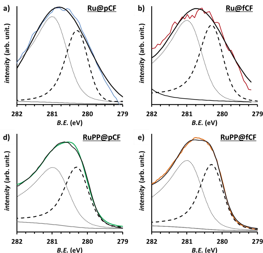
Figure 4. XPS analysis of a) Ru@pCF (blue), b) Ru@fCF (red), c) RuPP@pCF (green) and d) RuPP@fCF (orange). Background (grey), metallic-Ru component ( \text{Ru } 3d_{5/2} -279.8, dashed black), \text{RuO}_2 -component ( \text{Ru } 3d_{5/2} -280.8, dotted-black), envelope (bold).
