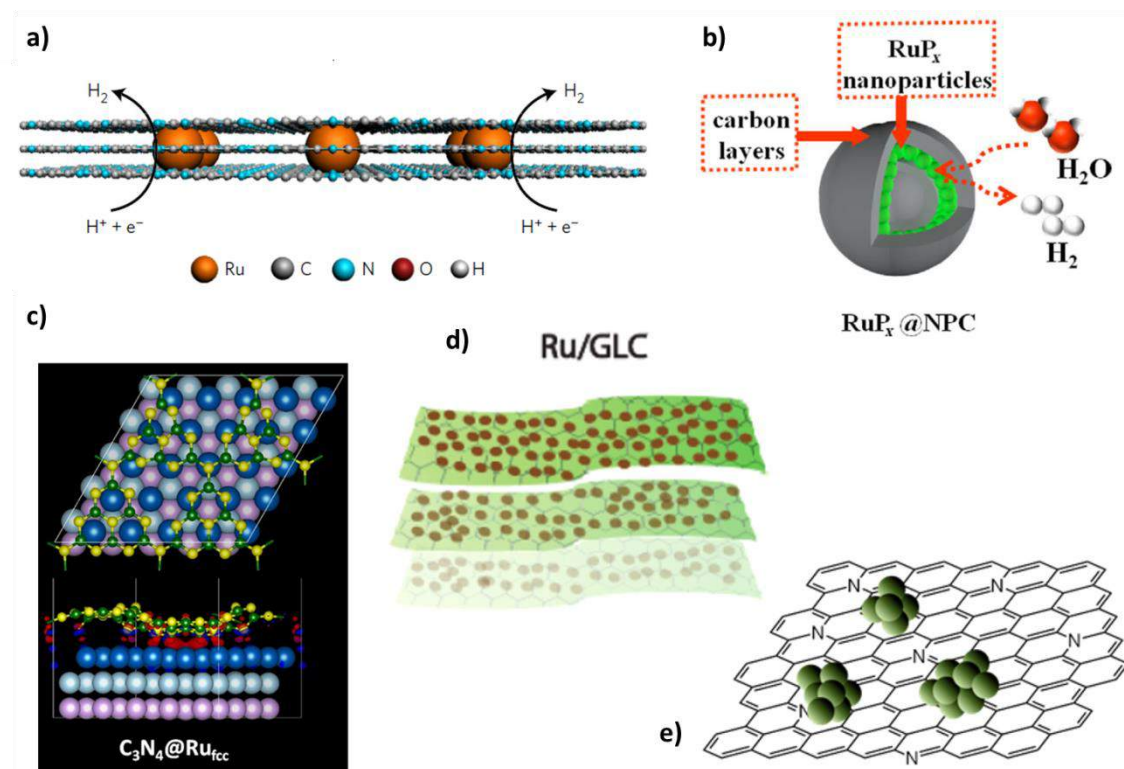
Figure 19. Ru-based nanosystems as HECs: a) Baek's \text{Ru}@C_2N , 119 b) Liu's \text{RuP}_x@NPC , 127 c) Qiao's \text{Ru}/C_3N_4/C , 131 d) Adschiri's \text{Ru}/\text{GLC} 125 and e) Tour's \text{Ru-NG750} . 130
