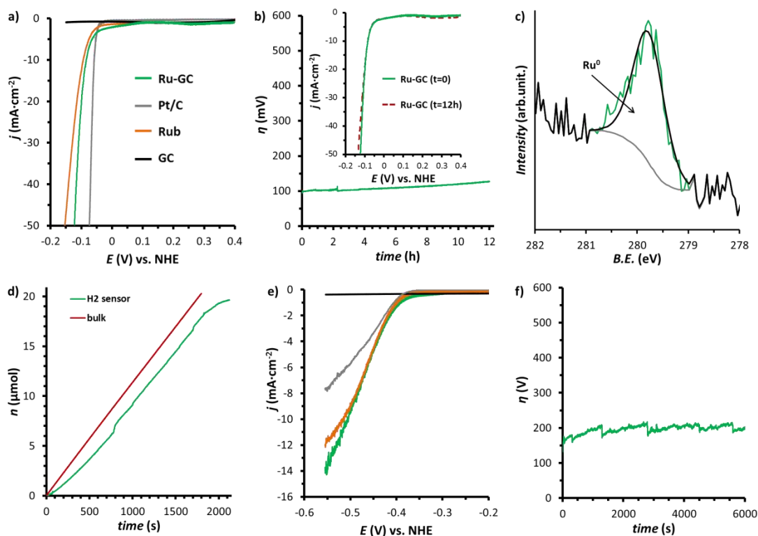
Figure 3 a) LSV curves of Ru-GC (green), Rub (orange), Pt/C (grey) and bare GC d electrode (black) in 0.5 M H 2 SO 4 solution; b) current-controlled bulk electrolysis experiment of Ru-GC at j = -10 \text{ mA}\cdot\text{cm}^{-2} in 0.5 M H 2 SO 4 . Inset, LSV curves of the initial Ru-GC (green) and after 12h bulk electrolysis (dashed red); c) XPS spectra of Ru-GC (green) after 15 min bulk electrolysis at j = -10 \text{ mA}\cdot\text{cm}^{-2} in 0.5 M H 2 SO 4 . Background (grey), metallic-Ru component (dashed black), envelop (bold); d) H 2 evolution profile measured by Clark electrode (green) compared to CPE (red); e) LSV curves of the Ru-GC (green), Rub (orange), Pt/C (grey) and bare GC d (black) in 0.1 M PBS; f) current-controlled bulk electrolysis of the Ru-GC at j = -10 \text{ mA}\cdot\text{cm}^{-2} in 0.1 M PBS, without ohmic-drop compensation.
