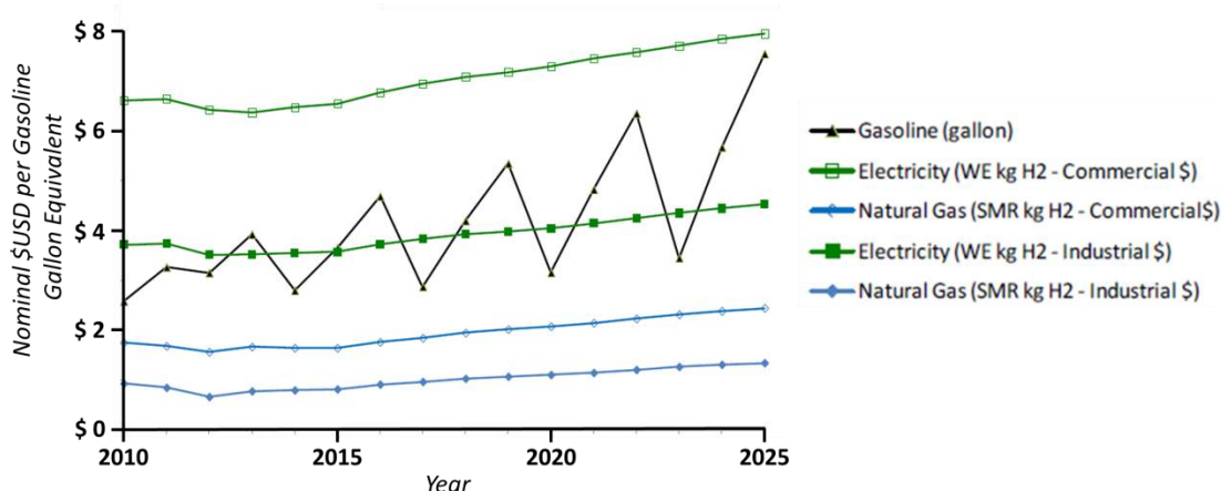
Figure 3. Past, present and future perspective on the cost of using H_2 instead of gasoline, published by Air Products. 22 Gasoline (black triangle), commercial electricity from WE (empty green square), industrial electricity from WE (filled green square), commercial natural gas from SMR (empty blue diamond) and industrial natural gas from SMR (filled blue diamond).
