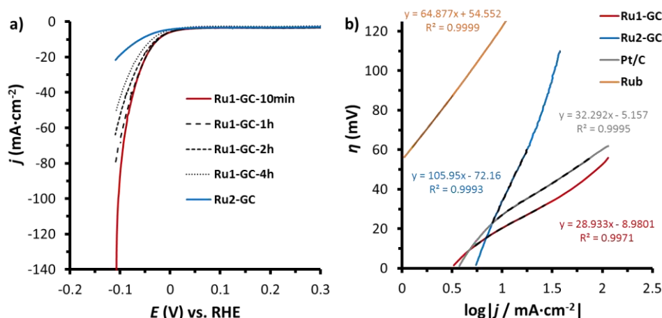
Figure 9. a) Polarization curves of Ru1-GC (after 10 minutes, electrode and electrochemical set-up preparation time) and subsequent curves, and Ru2-GC (blue) in 1 M \text{H}_2\text{SO}_4 . b) Tafel plot of Ru1-GC (dark red), Ru2-GC (blue), Pt/C (grey) and Rub (orange) in 1 M \text{H}_2\text{SO}_4 .
