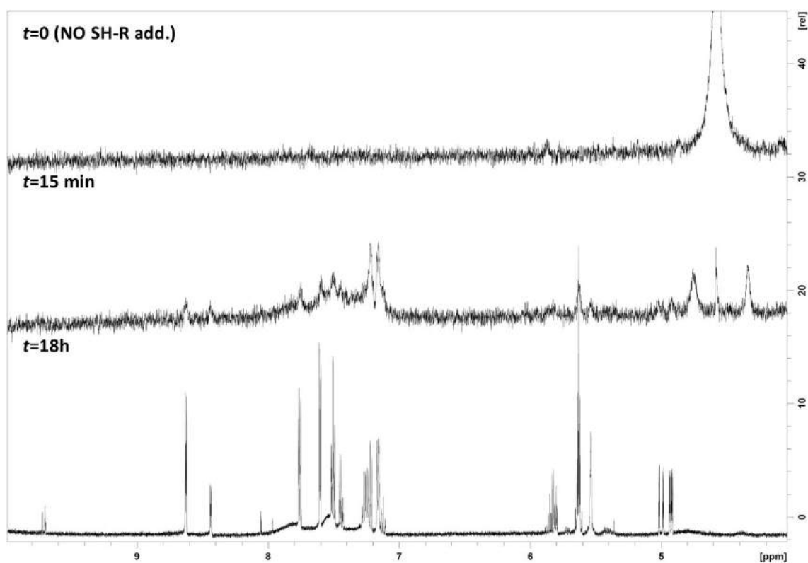
Figure 10. ^1\text{H} -NMR spectra (aromatic region) in d^8 -THF of the exchange experiment based on the addition of 1-octanethiol onto preformed Ru-0.2PP NPs at t=0 (before addition of thiol), t=15 min and t=18 h.
