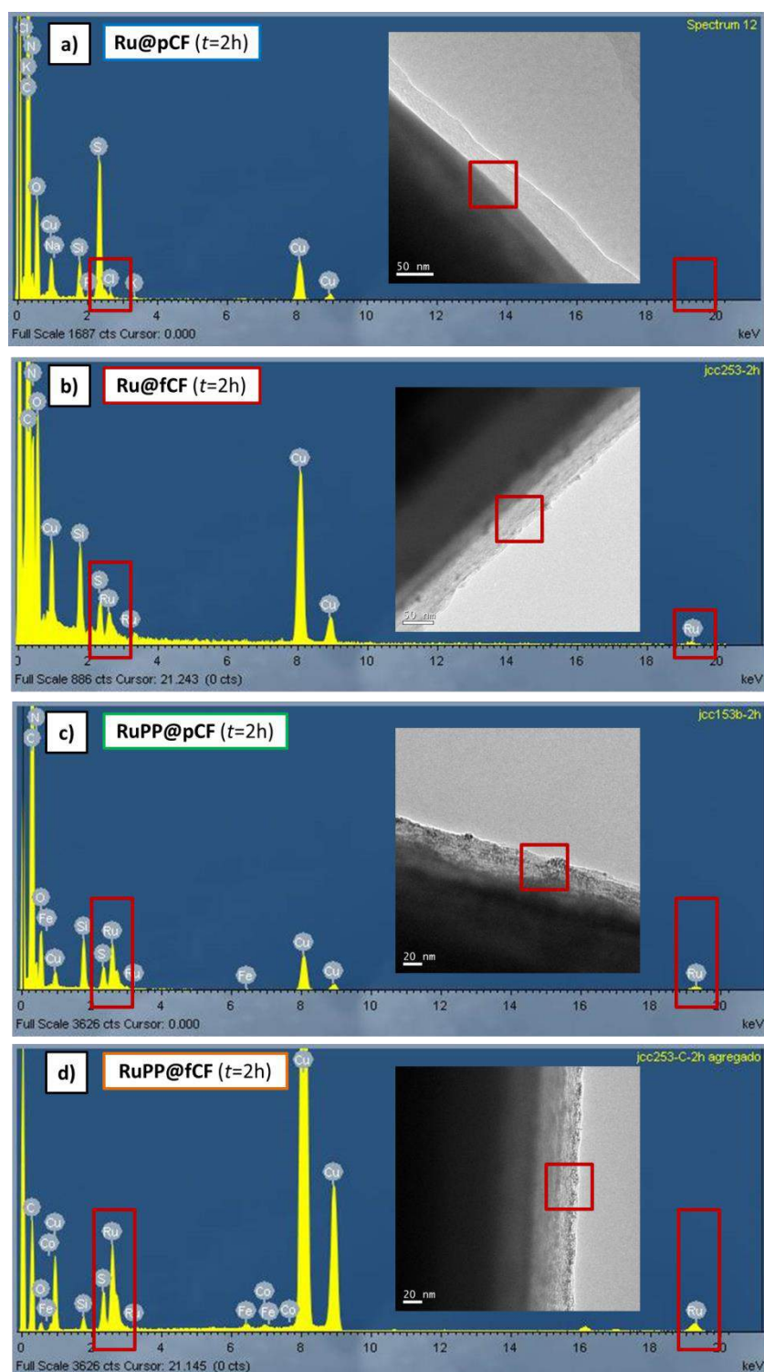
Figure 8. TEM/EDX analysis of a) Ru@pCF , b) Ru@fCF , c) RuPP@pCF and d) RuPP@fCF at t=2h after bulk electrolysis in 1 M H_2SO_4 at \eta = 250 and 350 mV for Ru@xCF and RuPP@xCF, respectively.
