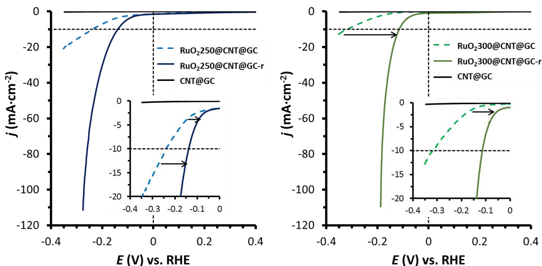
Figure 8. Polarization curves of RuO 2 @CNT systems before and after reductive process at |j| = 10 \text{ mA}\cdot\text{cm}^{-2} in 1 M \text{H}_2\text{SO}_4 . Left, RuO 2 250@CNT@GC (dashed blue) and RuO 2 250@CNT@GC-r (dark blue); right, RuO 2 300@CNT@GC (dashed green) and RuO 2 300@CNT@GC-r (dark green).
