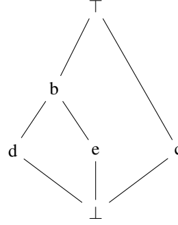
Figure 1.4: A lattice.
