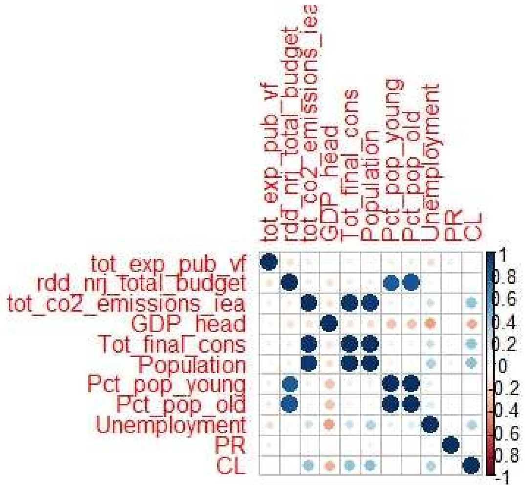
Figure 3.3: Correlation matrix
