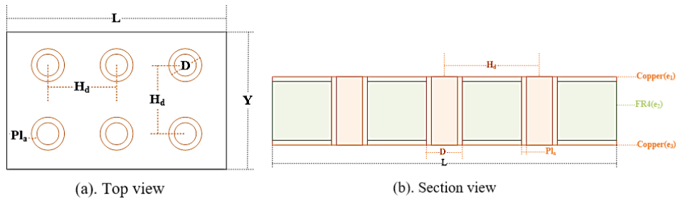
Fig.3-5. Top and section view of the PCB substrates with multiple thermal vias in pattern 1
