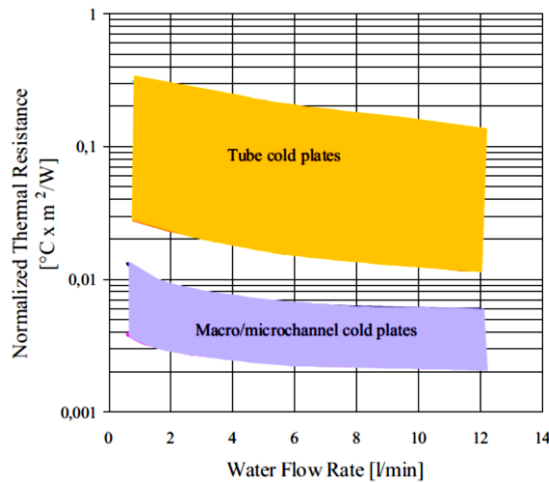
Fig.1-27. Thermal resistance of commercial available cold plates as a function of water flow [125]
