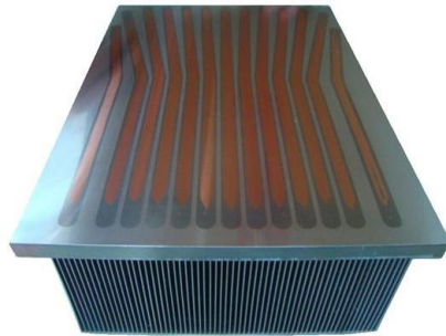
(c). Air cooled heat sink with embedded heat pipes
