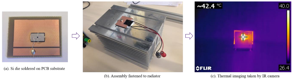
Fig.2-8. Thermal imaging of a simple PCB structure
