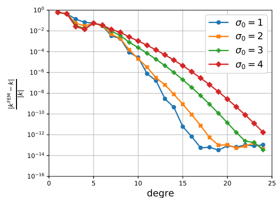
(f) k_{0,2}
