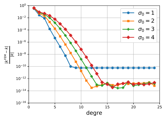
(b) k_{2,0}
