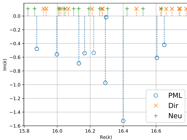
(b) p = -1
