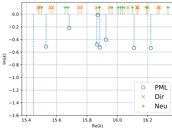
(a) p = +1
