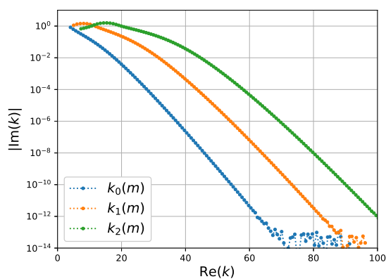
(c) Disque
