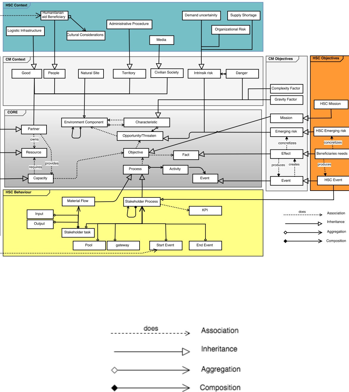
Figure 29 UML relationships between classes used on the HSC metamodel
