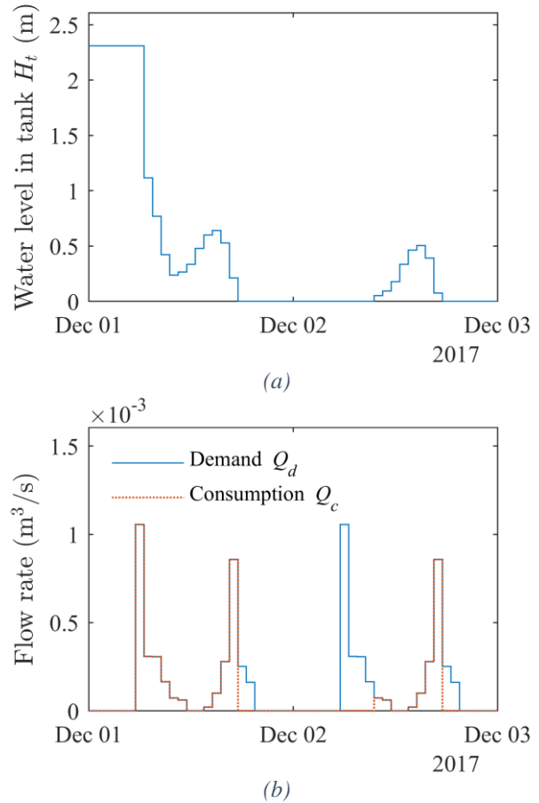
Figure III-19 – Undersized PVWPS. (a) Water level in the tank (b) Demand and consumption flow rates.
