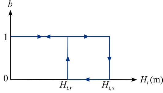
Figure III-8 – Controller model.
