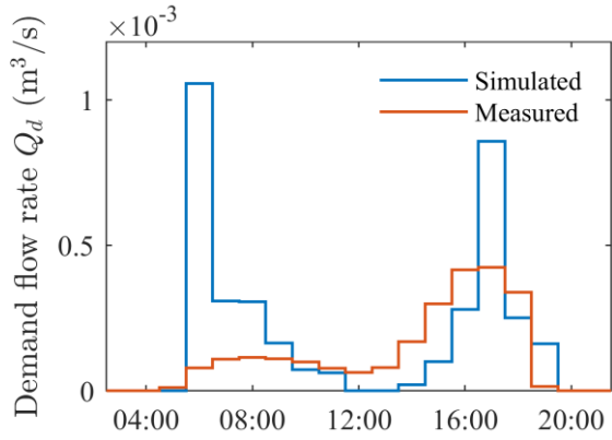
Figure III-3 – Demand flow rate profile simulated by the demand model and measured by the data logger (i.e. flow meter data) – dry season.
