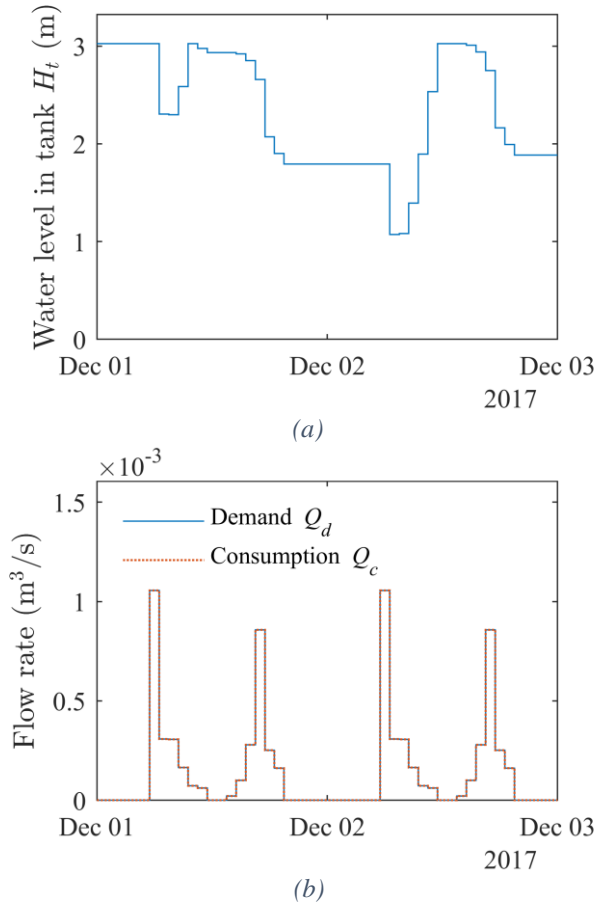
Figure III-18 – Oversized PVWPS. (a) Water level in the tank (b) Demand and consumption flow rates.
