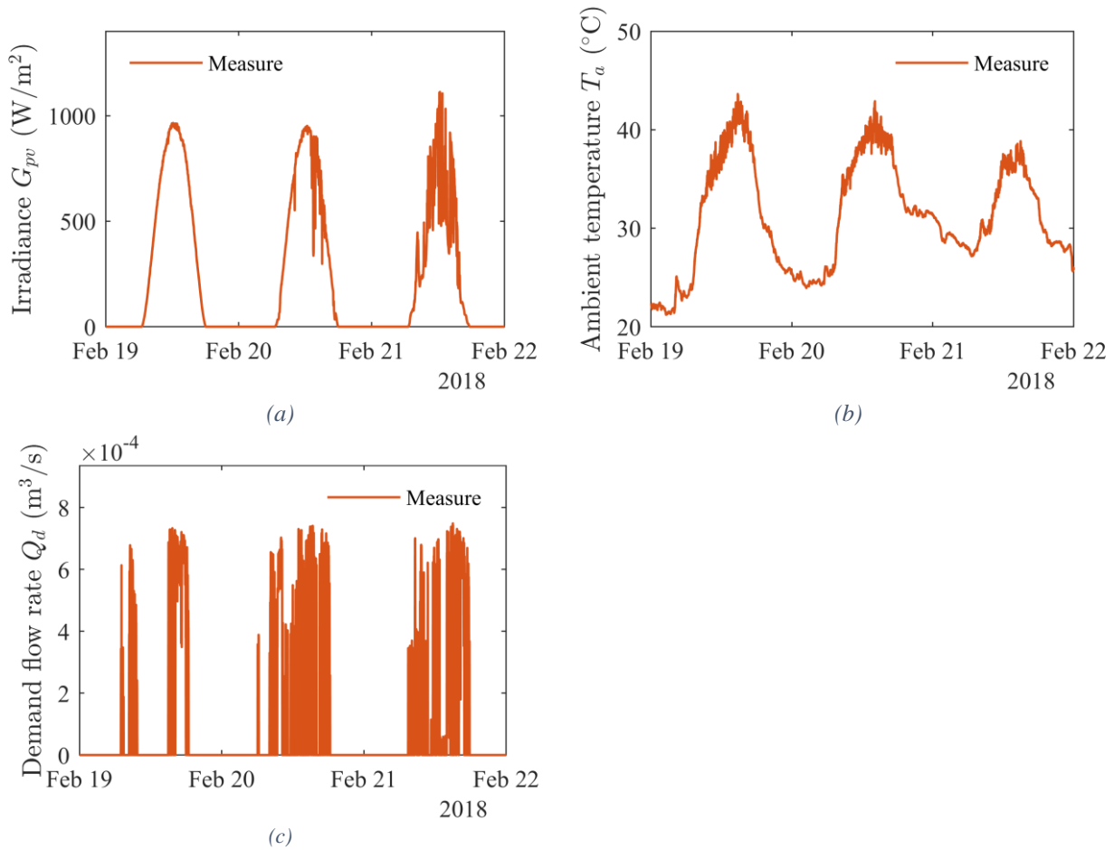
Figure III-11 – Measured model inputs (a) irradiance (b) ambient temperature (c) demand flow rate.
