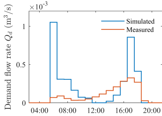
Figure III-4 – Demand flow rate profile simulated by the demand model and measured by the data logger (i.e. flow meter data) – wet season.
