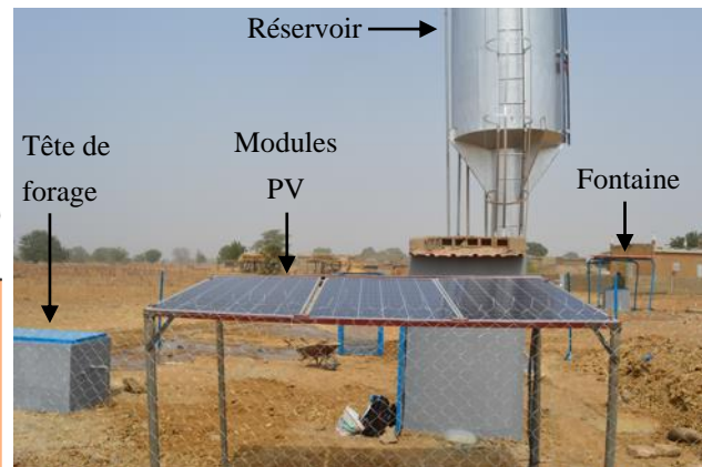
figure 3 – Photo du PVWPS.
