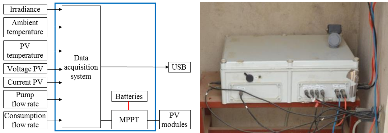
Figure II-13 – Data logger developed for monitoring the PVWPS of Gogma.
