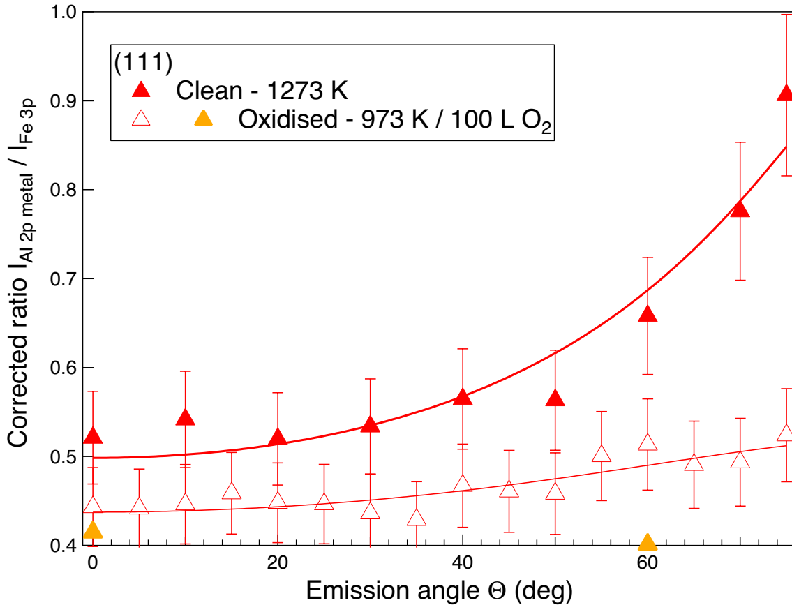
Figure 6.26: Segregation under the oxide at the (111) surface from the angular variation of the corrected ratio I_{\text{Al } 2p \text{ metal}} / I_{\text{Fe } 3p} (pass energy E_p = 50 eV) in the as-prepared (111) surface (1273 K; filled triangles) and after oxidation (973 K, 100 L of \text{O}_2 ; open triangles). Data (points) have been fitted with a model of continuous profile of segregation (lines, Eq. 5.4) which values are given in Tab. 5.3, 6.2. The orange points correspond to another measurement.
