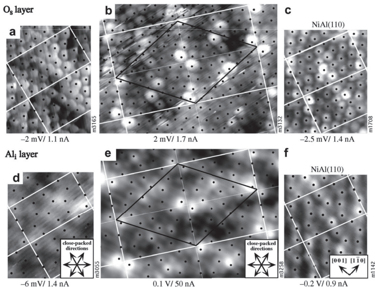
Figure 3.29: Atomic resolved STM images of an oxidised Cu-9 at.% Al(111) (100 L of \text{O}_2 at 953 K). a-c) The surface O layer and d-f) the interface Al layer visible at higher tunneling resistance. The left images (a,d) display the first (incommensurate) oxide structure and the centre images (b,e) show the second (commensurate) one. As a matter of comparison, the oxide on NiAl(110) is shown on right side. The dots mark the atomic positions of the alumina calculated on NiAl(110) [15]. In (b,e) the primitive unit cell is drawn in black and the four rectangular building blocks are marked in white. From Ref. [18].
