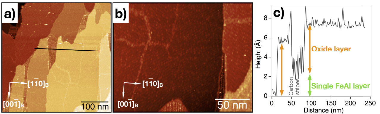
Figure 6.14: STM images of the \text{Fe}_{0.85}\text{Al}_{0.15} (110) surface after annealing at 1073 K in 2 \times 10^{-7} mbar \text{O}_2 for 10 min (90 L): a) 400 \times 400 \text{ nm}^2 , U_b = 2.0 \text{ V} , I_t = 0.4 \text{ nA} . b) 200 \times 145 \text{ nm}^2 , U_b = 2.0 \text{ V} , I_t = 0.4 \text{ nA} . c) Line profile from image-a.
