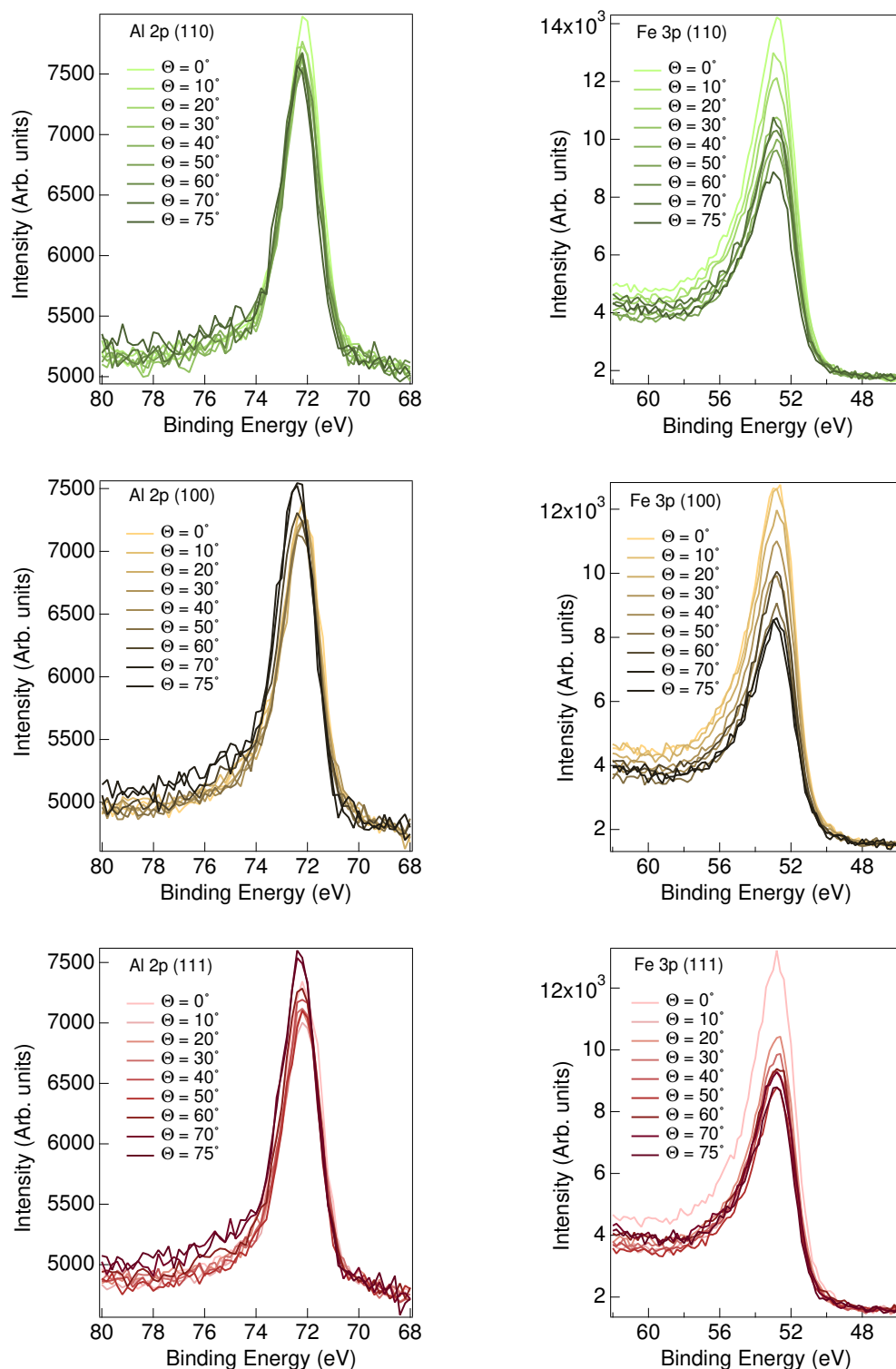
Figure 5.6: Evolution with emission angle \Theta of Al 2p and Fe 3p core levels of (110), (100) and (111) surfaces of clean \text{Fe}_{0.85}\text{Al}_{0.15} annealed at 1273 K. Spectra have been normalised to background.
