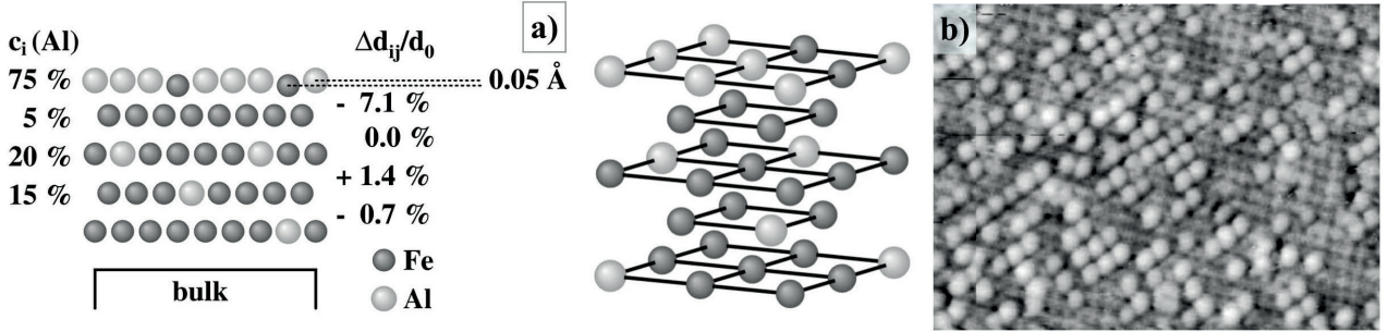
Figure 3.11: a) Structural models of \text{Fe}_{0.85}\text{Al}_{0.15}(100)\text{-(1 \times 1)} and b) room temperature STM image of this surface ( 100 \times 83 \text{ \AA} , U_b = -6 \text{ mV} , I_t = 0.46 \text{ nA} ). According to authors, a clear chemical contrast is achieved between Fe (protruding atoms) and Al (dark indentations). From Ref. [32].
