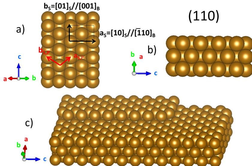
Figure 3.4: Same as Fig. 3.3 but for the (110) orientation. a) Top view along [110]_B . The primitive unit cell is shown by red arrows. b) Side view along [\bar{1}10]_B . c) View in perspective with a monoatomic step.
