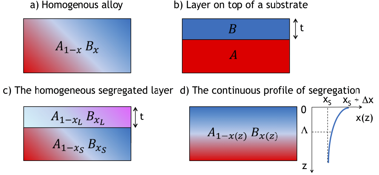
Figure 5.3: Models of profile of concentration used for photoemission analysis. a) The homogeneous semi-infinite alloy A_{1-x}B_x . b) The thin film on a substrate. c) The homogeneous segregated layer A_{1-x_L}B_{x_L} on a semi-infinite alloy A_{1-x_S}B_{x_S} . d) The continuous profile of segregation A_{1-x(z)}B_{x(z)} .
