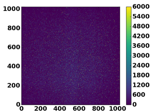
Fig. 7. Image resulting from the sum of 31 integrations of 800 ms each taken by the HIRG detector protected from any light signal by a cold plate but with the Ru source in front of the cryostat. The observed spikes energies expressed in DN are color-coded, their spatial distribution shows that the source was not perfectly centred. (For interpretation of the references to color in this figure legend, the reader is referred to the Web version of this article.)
