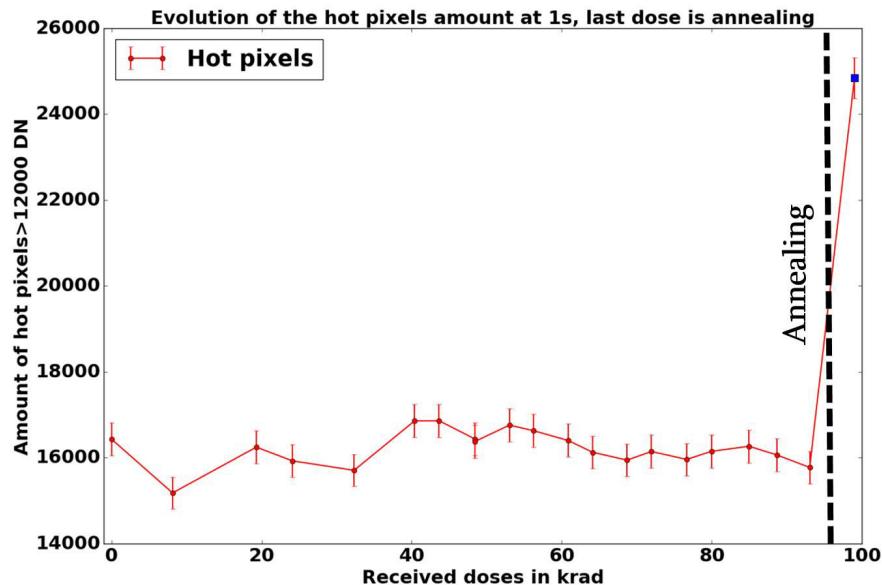
Figure 11: Variations of the number of hot pixels, averaged over 25 frames, during the TID sequences as a function of received dose after temperature bias compensation, at 1 s integration time. Error bars are computed as \pm 3 \cdot \sqrt{N} . The last blue point is on a different horizontal scale: it corresponds to the last sequence acquired after annealing but without further irradiation. It appears that the annealing deprecated the pixels status instead of improving it.
