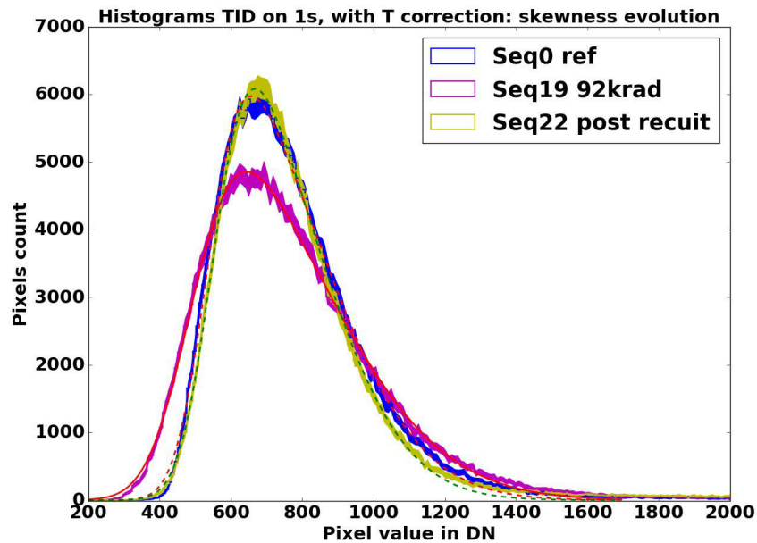
Figure 12: Histogram of the dark signal at 1 s on the detector with the exclusion of bad pixels. The thickness of the curves corresponds to 2-sigma error bars, showing that the dark signal non uniformity (histogram width or skewness) is increased by the irradiation but returns to normal after annealing. The changes of peak value due to measurement temperature differences between those 3 sequences has been corrected here. Red dotted line, red line and green line are best fit results with skewed Gaussian model.
