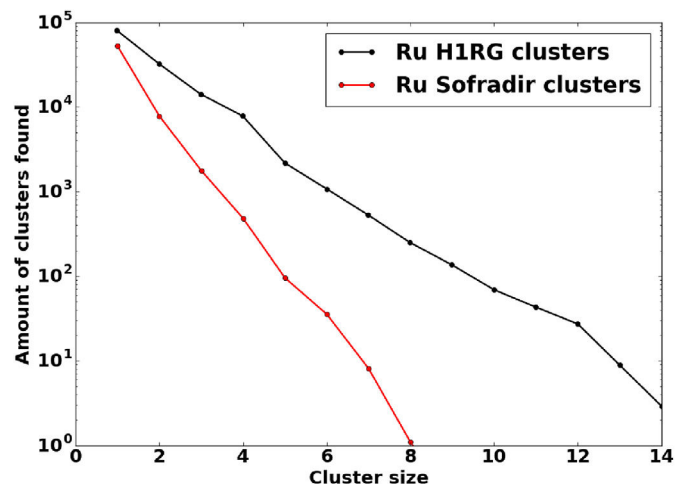
Fig. 14. Histogram of detected clusters versus their size with the Ru source, in black for HIRG and in red for Sofradir. (For interpretation of the references to color in this figure legend, the reader is referred to the Web version of this article.)
