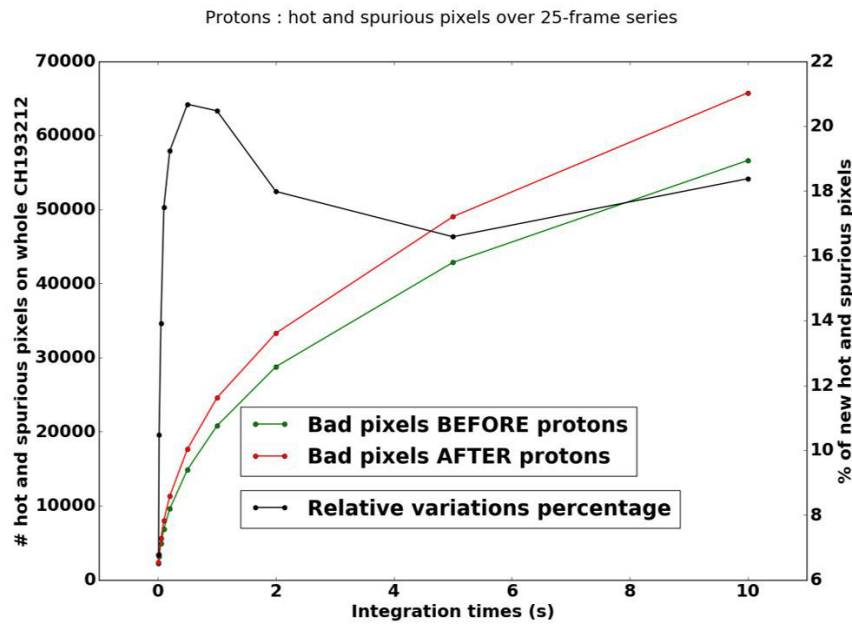
Figure 8: Number of hot pixels as a function of integration time before (green) and after (red) irradiation by protons. The relative increase in the number of bad pixels is illustrated by the relative variations percentage in black curve. Those variations are about 19\% \pm 2\% for integration times between 100 ms and 10 s.
