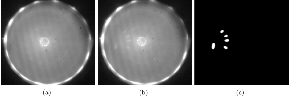
Figure 4.9: Finger tracking: (a) Background image with no fingers. The illumination is almost uniform on the sphere except close to the opening where we do not expect any tracking and at the pole where the LEDs are specularly reflected. (b) Sensed image with touching fingers. (c) Retrieved blobs, containing touch related information
