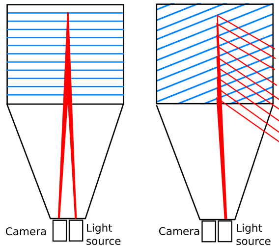
Figure 5.9: By rotating the prismatic film, the camera is no longer dazzled by the specular reflection of the light source.
