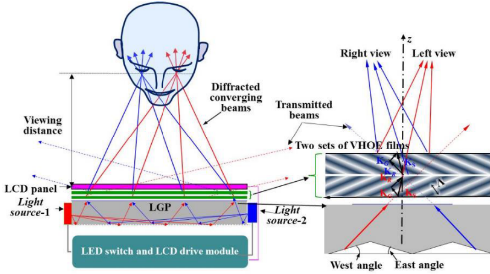
Figure 3.6: A light guide and HOE solution to provide a directional backlight: LED sources emit light in a guide from different sides and a HOE directs the rays toward different viewing zones (source: [HBF + 14])
