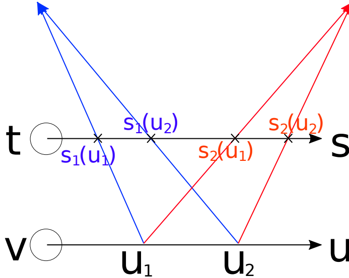
Figure 3.10: light-field parametrization of a schematic autostereoscopic display (seen from above)
