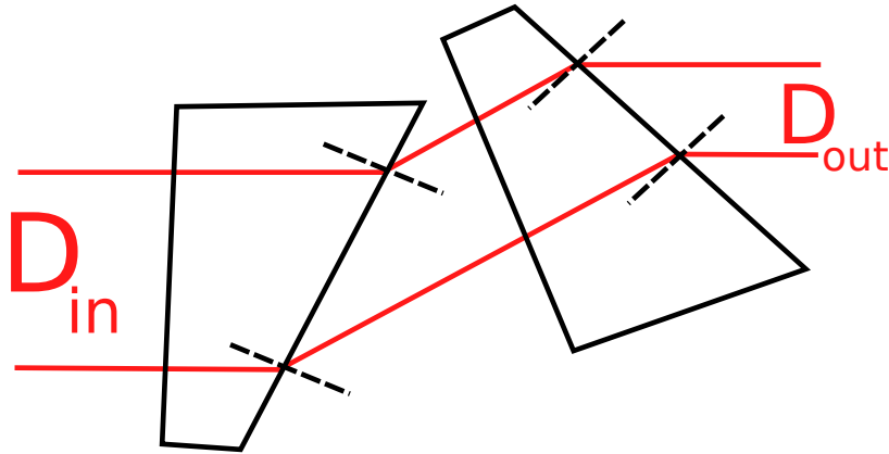
Figure 4.15: A pair of prisms can shape a beam in one dimension without affecting the other.
