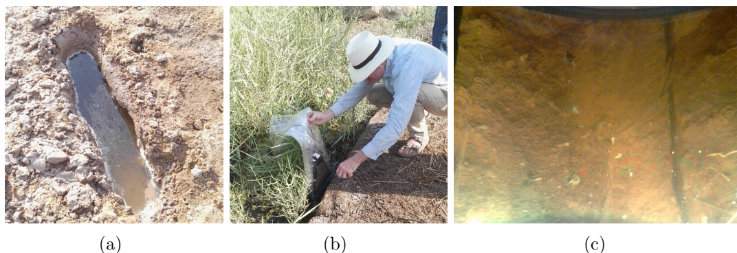
Figure 5.13: (a) An overflooded trench where the wedge can be used; (b) a wedge being used for observing the side of a flooded area; (c) image acquired underwater.
