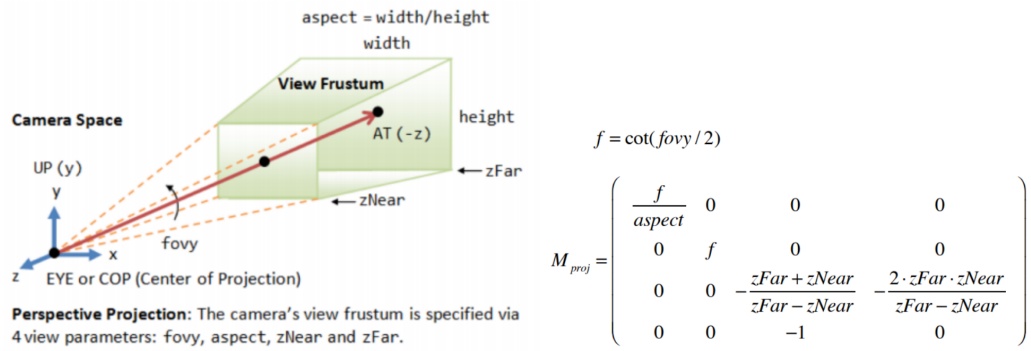
Figure 2.16: Perspective camera model and projection matrix (source: [Wet19])
