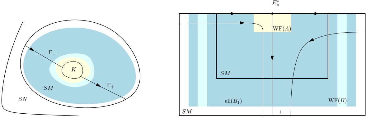
FIGURE 7.2 – In yellow, light blue, darker blue : (resp.) WF(A) , WF(B) , ell(B_1) . Left : The projection of the previous sets on the base SM . Right : Vertical lines represent the dynamics in the physical space SM , horizontal lines represent the dynamics in the cotangent space T^*(SM) .
